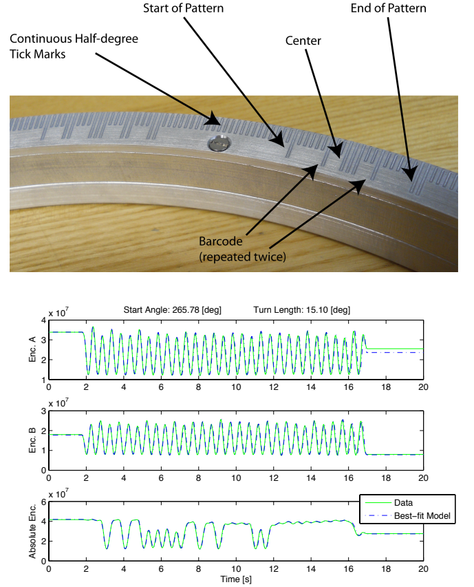
FIG. 6. Main encoder. The top panel is a photograph showing both the continuous and barcode tracks of the encoder attached to the main gear. The bottom panels are plots of encoder data (in raw ADC units) from a 15-degree turn taken with a mechanism operating cold in the SPIDER flight cryostat. The best-fit model timestream is overplotted, which allows a precise estimate of the start and stop angles.
