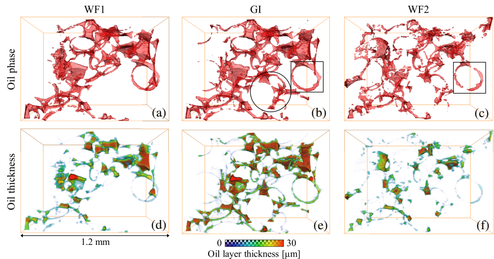
Figure 9. (a–c) Three-dimensional rendering of the connected oil phase in a subset of the rock at the end of WF1, GI, and WF2, respectively. In the circled region of panel (b), we highlighted the formation of new oil layers during GI. (d–f) Thickness map of the oil phase represented in panels (a)–(c).
