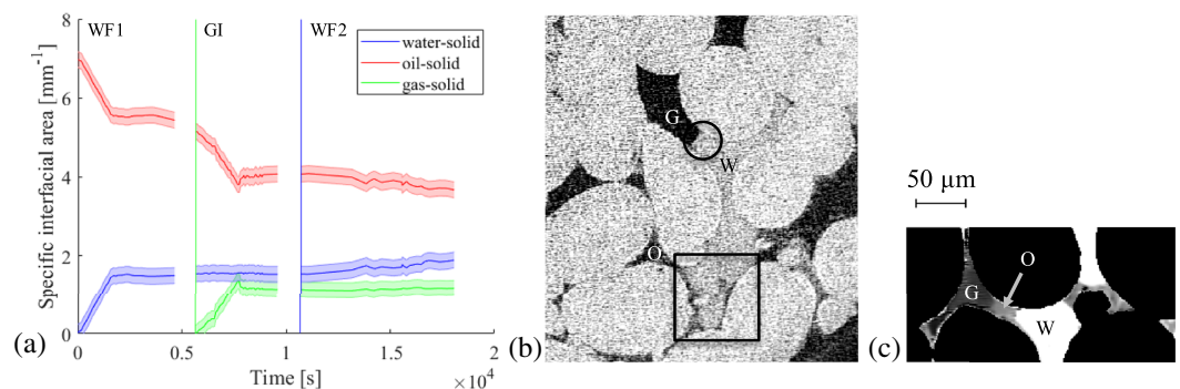
Figure 7. (a) The interfacial area between each phase and the solid, normalized to the total image volume; the width of the lines indicate the uncertainty in the measurements, estimated by using different training data sets for segmentation. (b) Two-dimensional slice of the gray scale image at the end of WF2, where G is gas, W is water, and O is oil. (c) Another slice of the gray scale image at the end of WF2, where the rock phase has been masked out for easier visual inspection. G is gas, W is water, and O is oil.
