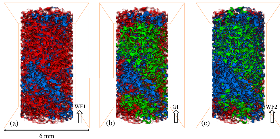
Figure 4. Three-dimensional rendering of oil (red), water (blue), and gas (green) at the end of (a) first waterflooding (WF1), (b) gas injection (GI), and (c) second waterflooding (WF2). The arrows show the direction of the injection of water and gas.
