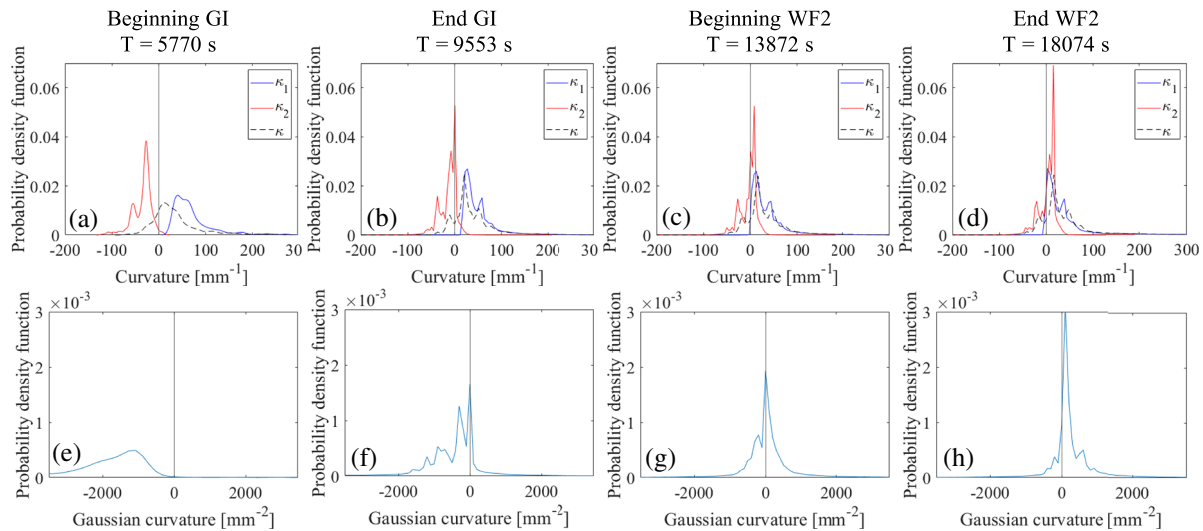
Figure 13. Focus on the gas-oil curvatures at four different times of the experiments (refer to Table 3). (a–d) Probability distributions of the curvatures \kappa_1 and \kappa_2 at the gas-oil interface in the two principal directions, along with the total curvature \kappa = \kappa_1 + \kappa_2 . (e–h) Gaussian curvatures \kappa_g = \kappa_1 \times \kappa_2 . The probability density functions are based on point measurements on the whole images. The resulting histogram is normalized such that the area under the curves sums to 1.
