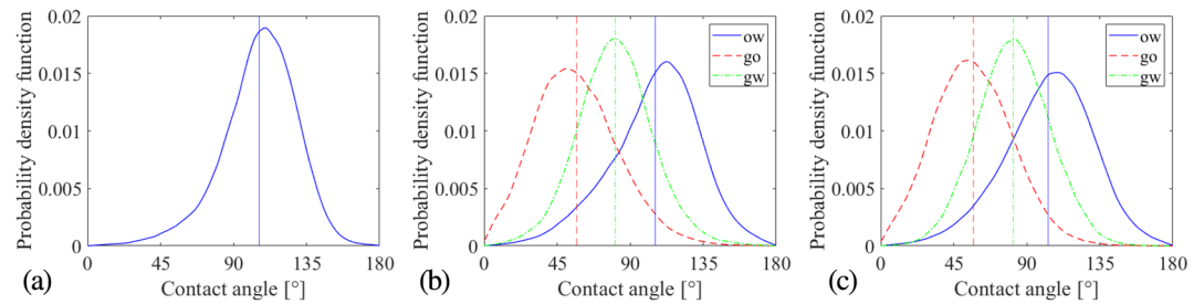
Figure 5. Estimations of probability density functions obtained from the histograms of the geometric contact angles, computed from the static images at the end of each injection: (a) WF1, (b) GI, and (c) WF2. The contacts angles are computed for oil-water (ow), gas-oil (go) and gas-water (gw) solid contacts. The vertical lines represent the mean values.
