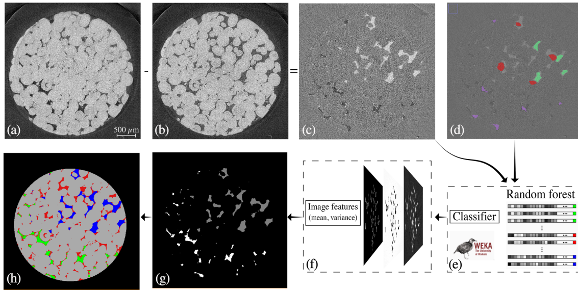
Figure 3. Workflow for image segmentation. (a) Image with four phases: gas, oil, water, and rock from darker to brighter. Rock and water have a similar attenuation coefficient. (b) Image taken before starting the dynamic experiment, with the sample filled with oil. Panel (c) is the differential image obtained subtracting panel (b) from panel (a): Gas-filled pores are black, while water-filled pores are white. Panel (d) represents the creation of the training data set, which is done on the differential image (c): Gas-filled pores were marked in purple, water-filled ones in green, and noninvaded regions in red. Panel (e) shows the WEKA machine-learning training algorithm, which takes panels (c) and (d) as input and creates a classifier. Panel (f) shows the image features on which the classifier is applied: These are the mean and variance of the gray scale values of the image. Panel (g) is the resulting segmented differential image, obtained using the classifier and the image features: Gas-invaded pores are white, brine-invaded pores are gray, and noninvaded pores are black. Panel (h) is the final segmented image, obtained by combining panel (g) with a segmented image of the sample before starting injection: Gas is green, oil is red, water is blue, and the rock is gray.
