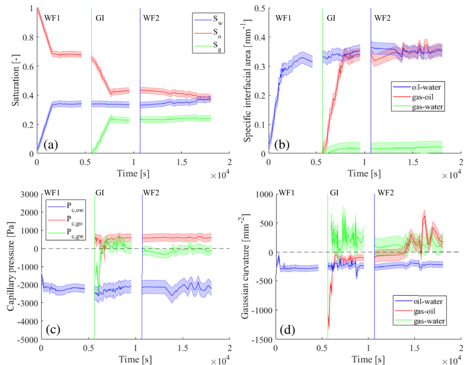
Figure 11. (a) Dynamic changes in saturations, (b) interfacial areas specific to the total volume, (c) capillary pressures, and (d) Gaussian curvatures between the phases involved in the experiment. The shadowed regions indicate the measurement uncertainty, obtained by using different training data sets for segmentation, and vertical lines show when each injection started. Horizontal dashed lines were added to the capillary pressure and Gaussian curvature plots to help distinguish between positive and negative values.
