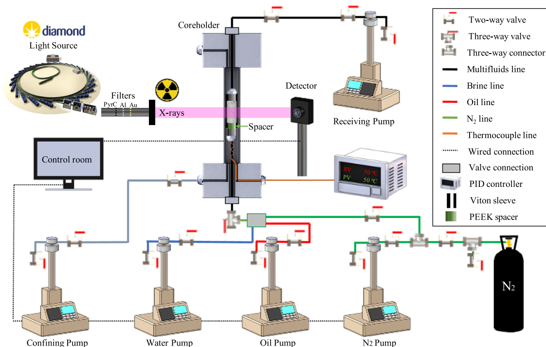
Figure 1. Schematic of the experimental apparatus comprising three injection pumps, a receiving pump, and a confining pump to maintain high fluid pressures. The sample is imaged using synchrotron X-rays.
