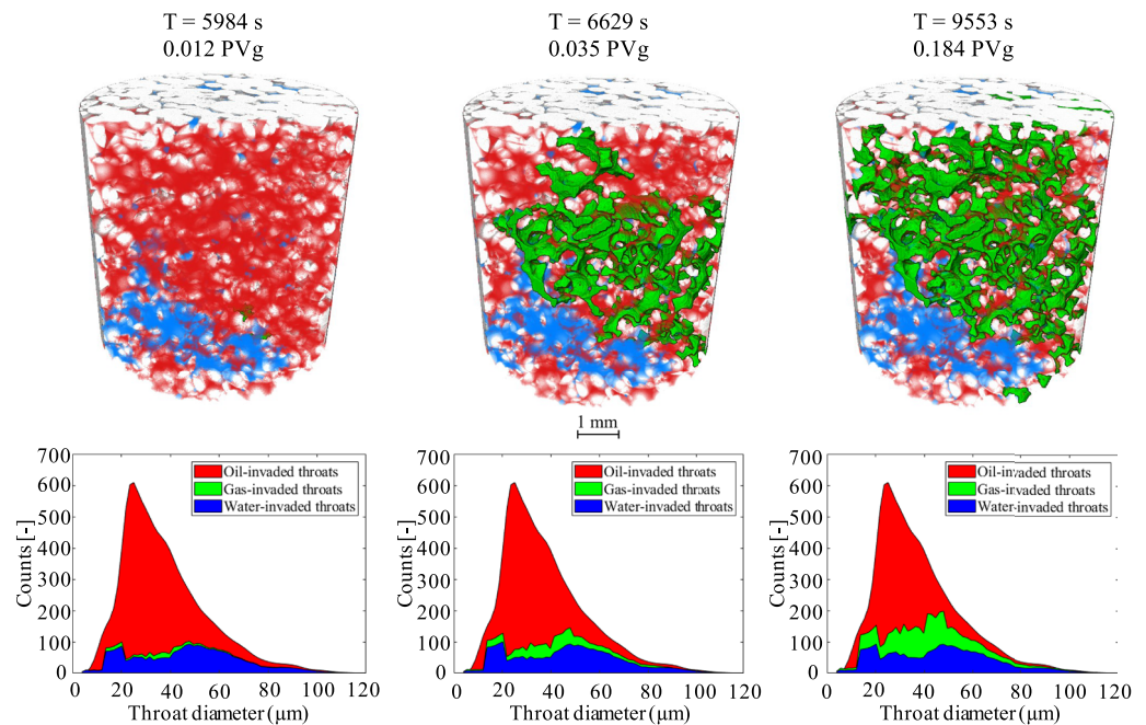
Figure 8. Top row: 3-D rendering of the rock (light gray), oil (red), water (blue), and gas (green) at different times during GI. Bottom row: area chart showing the distribution of throat size and their occupancy. PVg indicates the pore volumes of gas injected at each time step.
