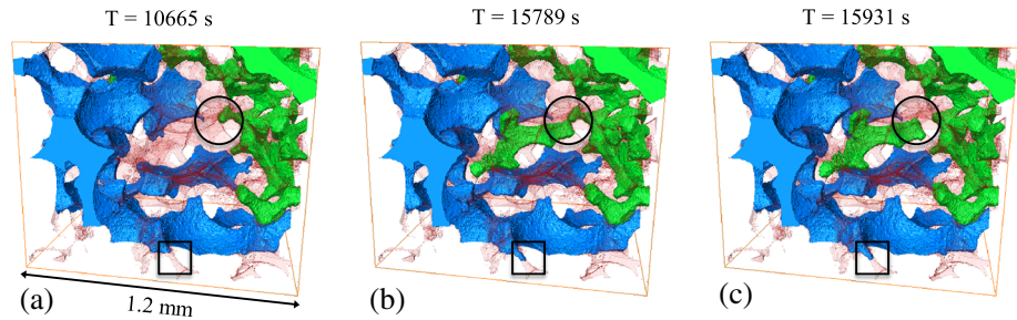
Figure 10. Three-dimensional representation of the fluids occupying the pores of a subvolume from the dynamic images, at three time steps (a), (b) and (c) during WF2. Water is blue, gas is green, and oil is in semitransparent red. In the circled throat, gas invasion is highlighted (b) with subsequent gas trapping by oil (c), while the square shows a signature of WF2: water invading a small throat as its pressure increased during injection.
