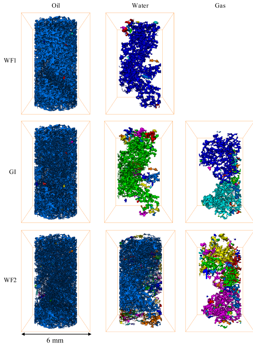
Figure 12. Connectivity of oil, water, and gas at the end of the first waterflooding (WF1), gas injection (GI), and second waterflooding (WF2). Different colors represent disconnected clusters of the same phase.
