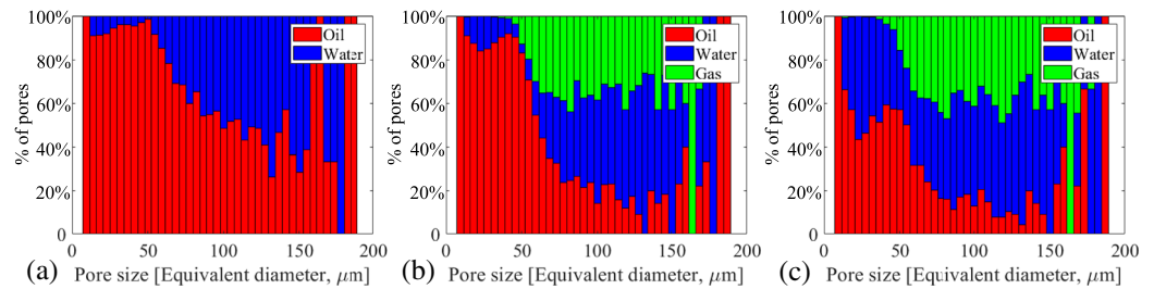
Figure 6. Pore occupancy at the end of (a) WF1, (b) GI, and (c) WF2.
