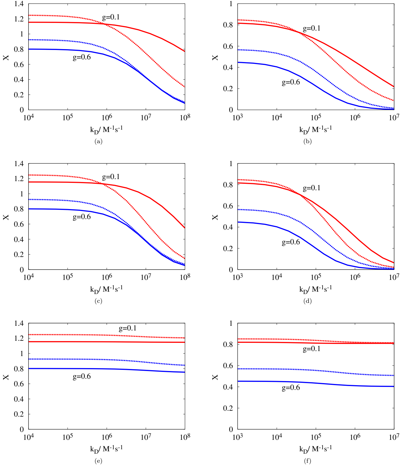
FIG. S16: The variation in specificity X_{\text{ss}} for a single-site system with the first phosphorylation site (dashed lines), and the additional specificity gained from adding the second site X - X_{\text{ss}} (solid lines), with increasing concentrations of bound enzyme/substrate complexes. It is clear that the loss of specificity associated with saturation is not, in these cases at least, overwhelmingly due to a reduced benefit from the second site rather than the first. We consider total molecule concentrations of (a,b) [A_0] = [B_0] = [K_0] = 1 \mu\text{M} , (c,d) [A_0] = [B_0] = 0.05 \mu\text{M} , [K_0] = 1 \mu\text{M} , and (e,f) [A_0] = [B_0] = 1 \mu\text{M} , [K_0] = 0.05 \mu\text{M} . In each figure we consider two fixed yields, g = 0.1 and g = 0.6 . In (a,c,e) we take P_{\text{on}} = 0.1 , and in (b,d,f) we use P_{\text{on}} = 0.9 . All other parameters are stated in the text.
