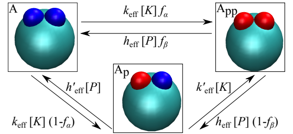
FIG. 3: Effective first-order description of the conversion of A between its phosphorylation states that results from the assumption of unsaturated kinetics. Arrows are labelled with effective rate constants.
