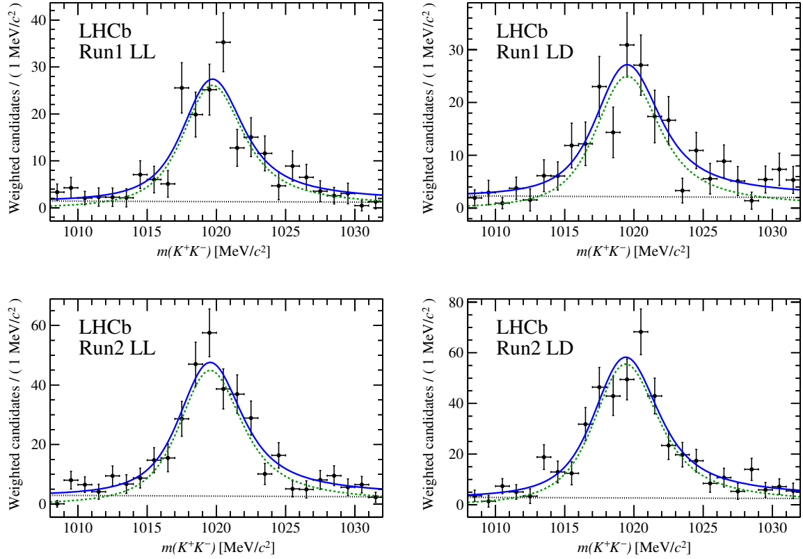
FIG. 4. Fits to the invariant-mass distribution m(K^+K^-) of B^0 \rightarrow \phi K_S^0 data weighted using the s Plot technique. The blue curve represents the complete model, the signal \phi component is given in green (dashed), and the background f_0(980) \rightarrow K^+K^- model is shown in black (dotted).
