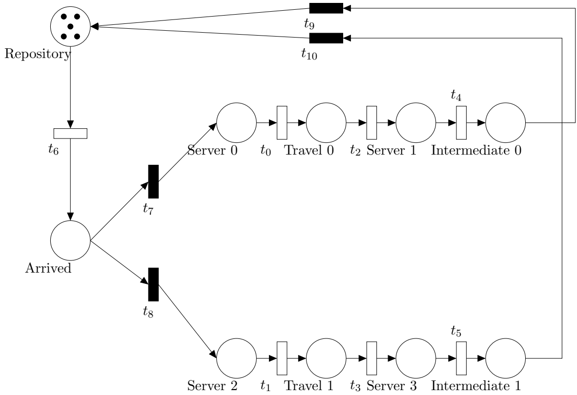
Figure 4.12: A complete overview of the initial structure of a PNPM model obtained at the end of the third stage of the processing pipeline for the set of location traces depicted in Figure 4.2. The immediate transitions t_7 and t_8 model the initial routing probability of the customer flow.
