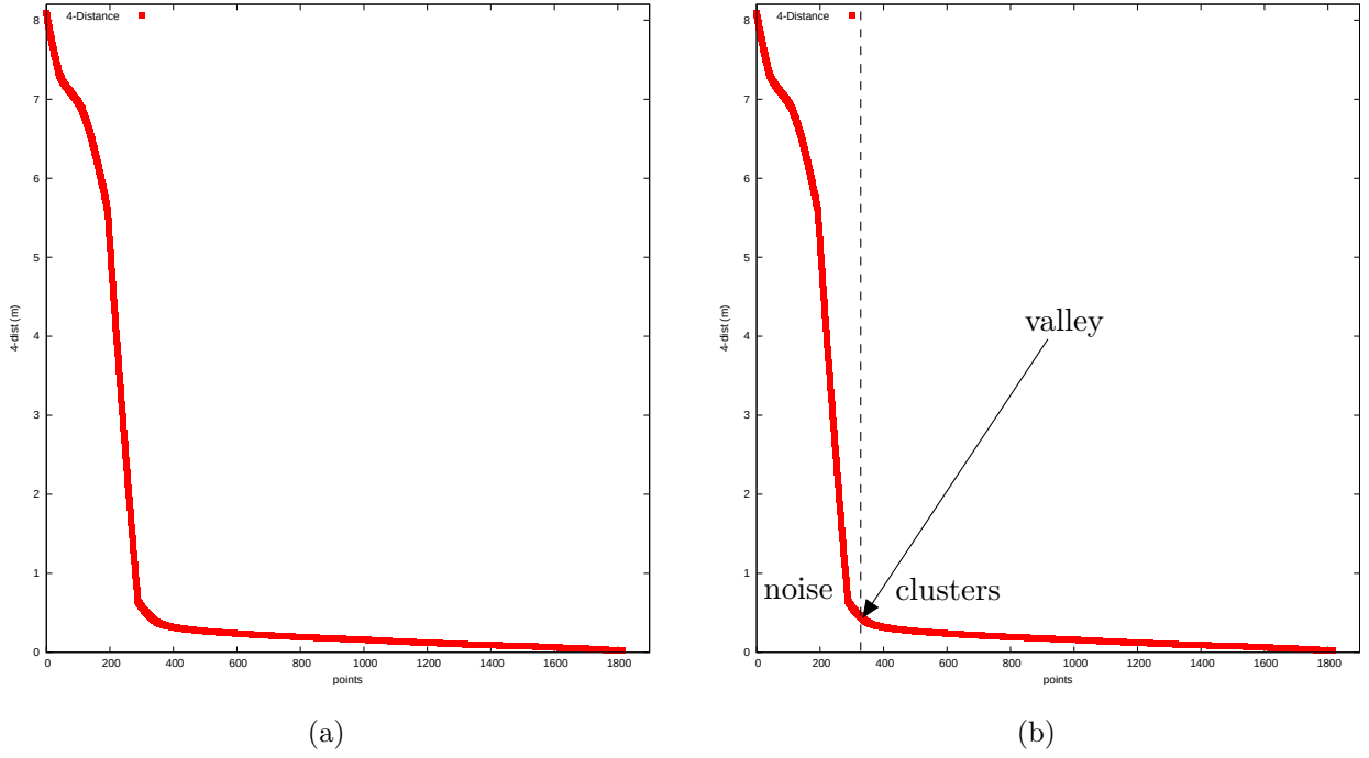
Figure 2.11: The sorted 4\text{-dist} graph of a sample dataset D (left) and Eps selection (right).
