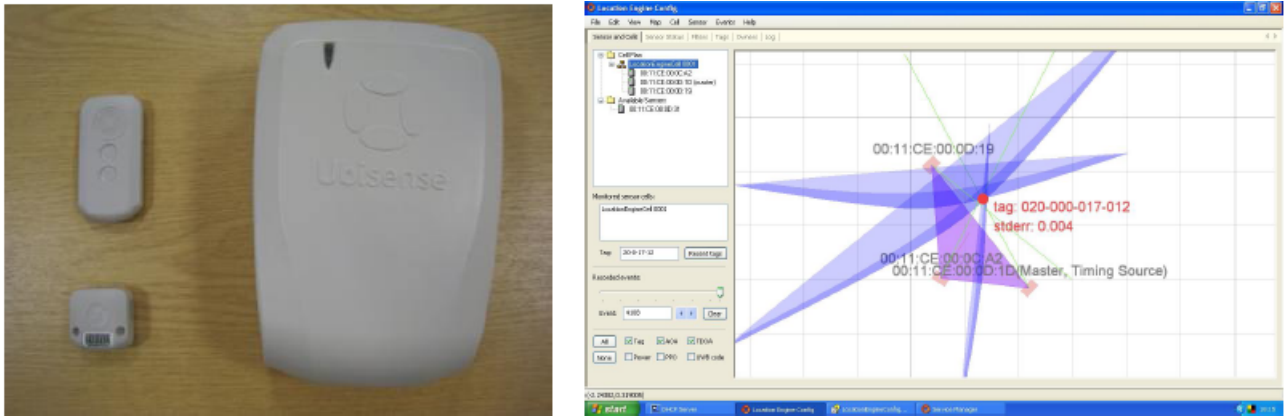
Figure 2.15: UWB-based sensors and tags (left) use a combination of angle-of-arrival and timed-difference-of-arrival triangulation schemes to enable high accuracy tag location tracking (right).
