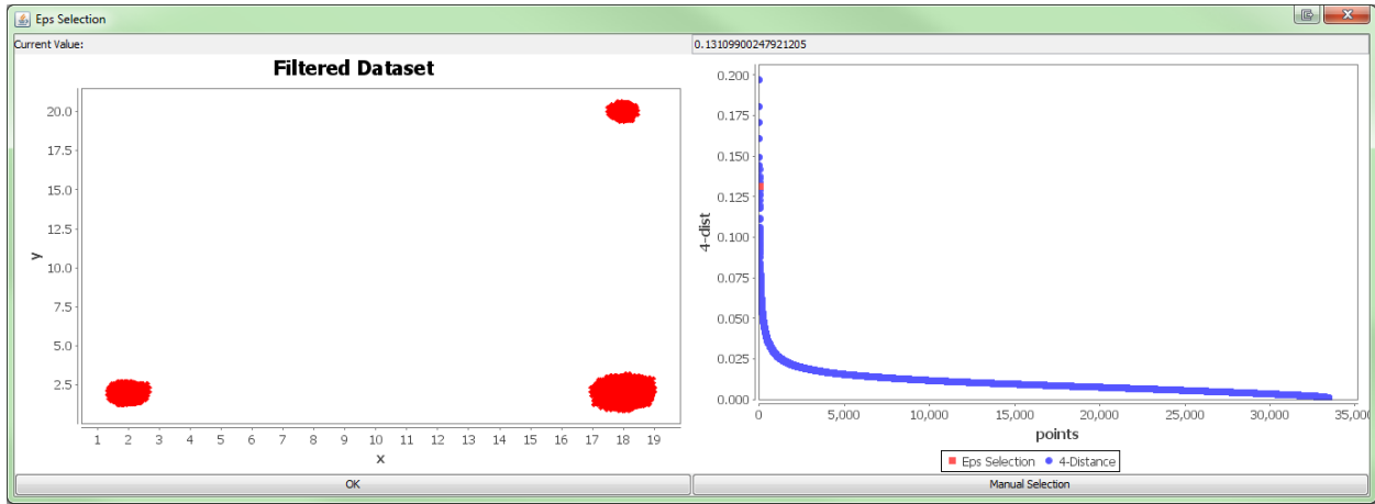
(a) The filtered dataset does not contain any noise points. The user should select the first 4\text{-dist} value.
