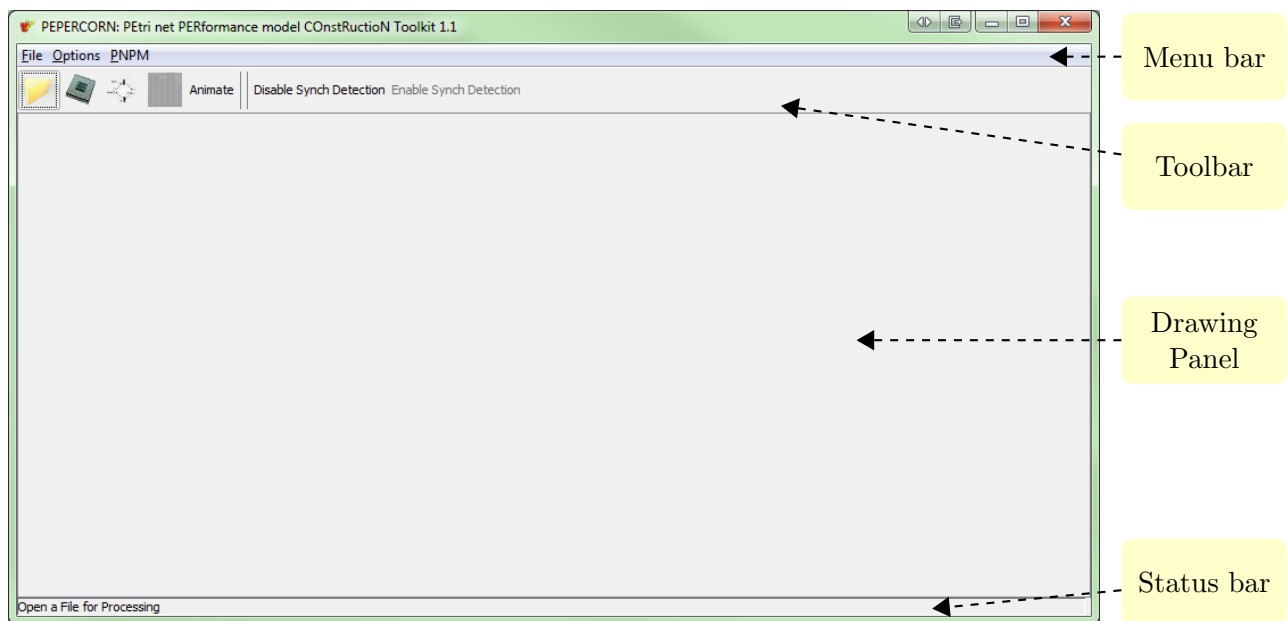
Figure 7.1: The main interface of PEPERCORN.
