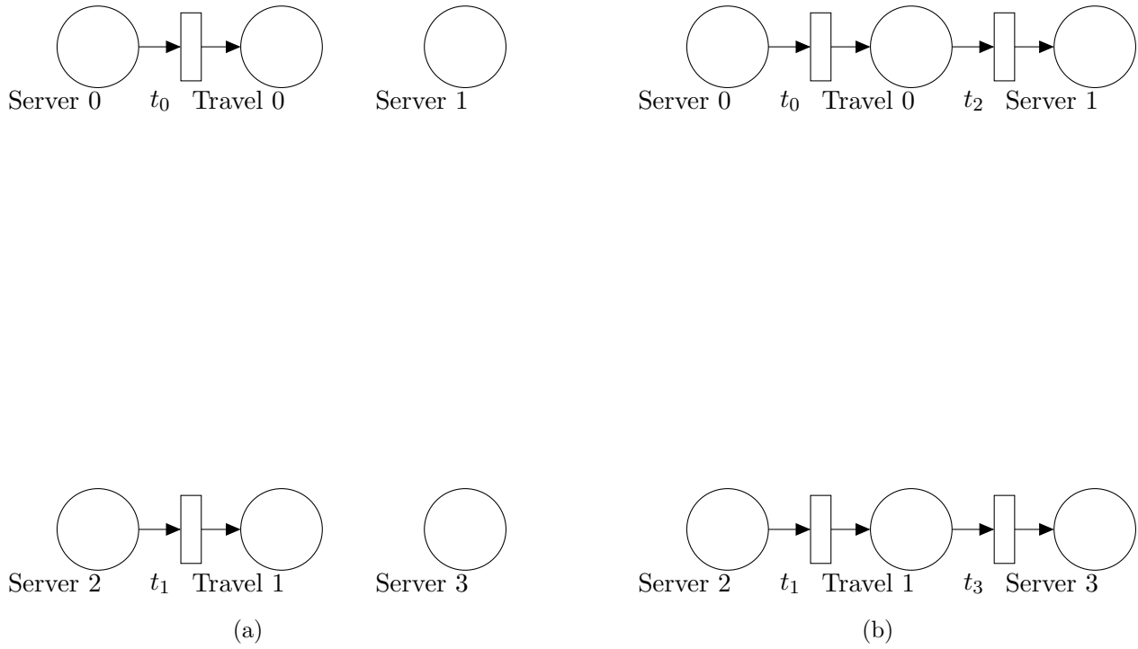
Figure 4.10: Addition of travel places between pairs of places representing service areas as well as transitions. Figure 4.10(a) shows the addition of service time transitions t_0, t_1 and Figure 4.10(b) the addition of travelling time transitions t_2, t_3 .
