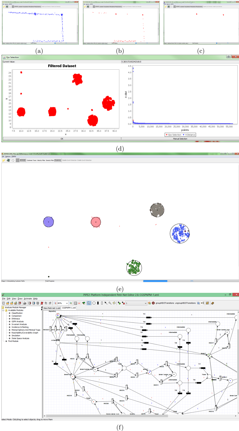
Figure 7.5: Figures 7.5(a), 7.5(b) and 7.5(c) show the animation of a customer's path and, the speed and density filters applied on that path respectively. Figures 7.5(d) and 7.5(e) show the Eps selection dialog and the clusters produced by the DBSCAN algorithm. Figure 7.5(f) shows the constructed PNPM as visualised in PIPE2 (in compact transition form).
