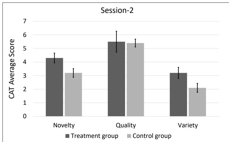
Figure 5: Results of CAT scores for ideas generated in two groups in session-2
