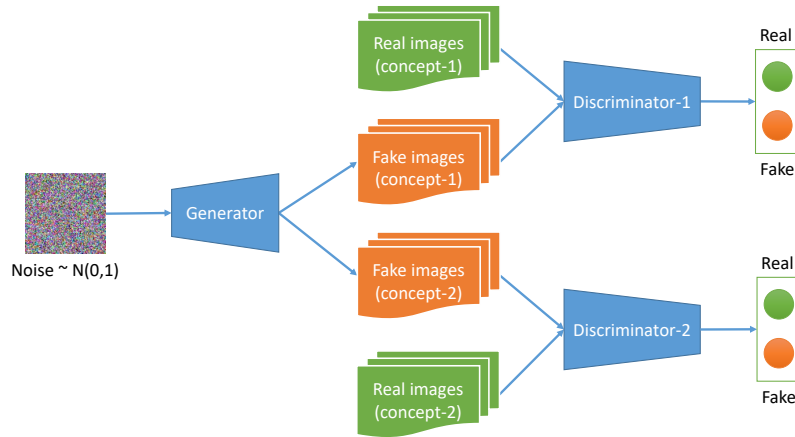
Figure 1: Generative adversarial networks model
