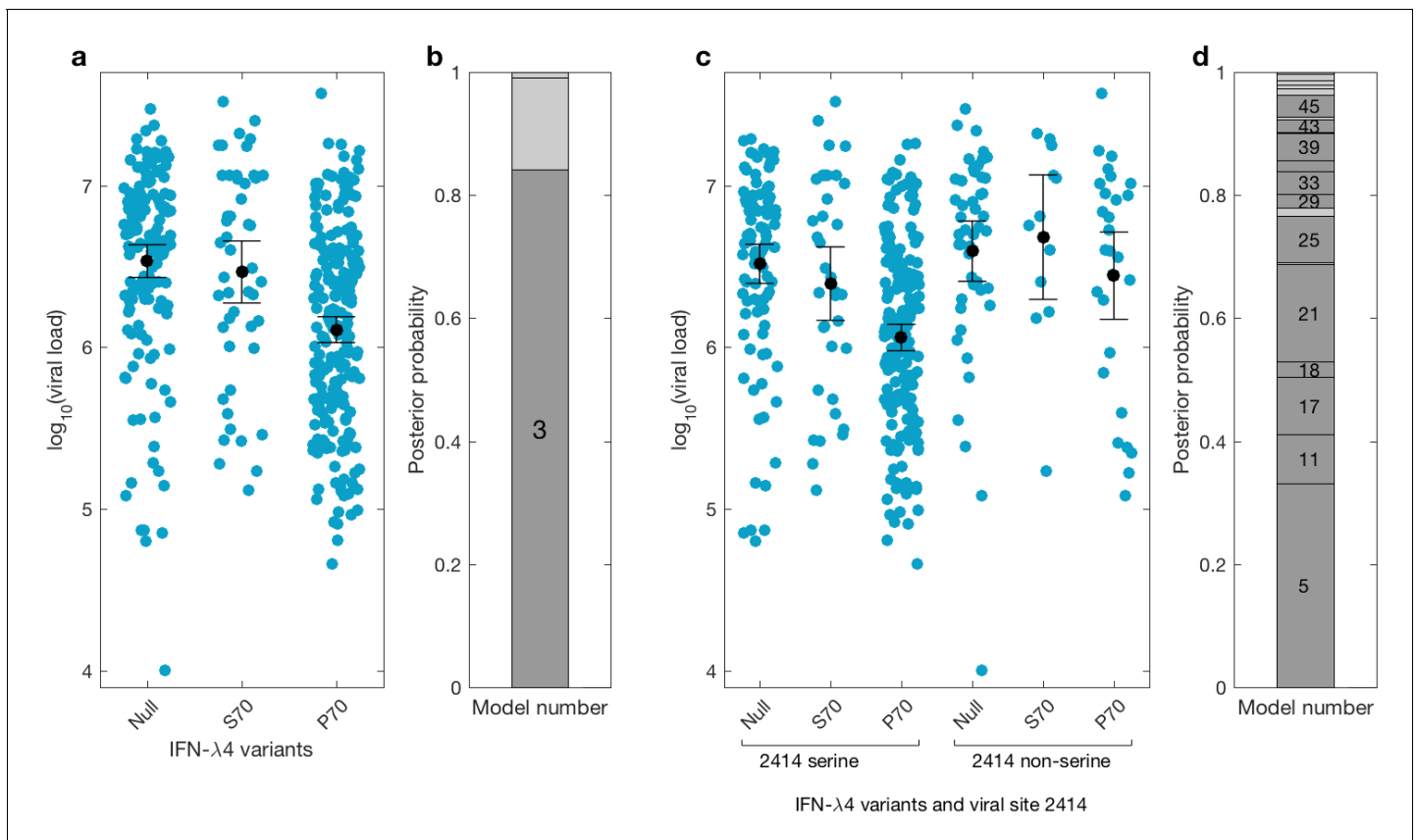
Figure 3. Bayesian model comparison of effect sizes of IFNL-λ4 variants on viral load in the BOSON cohort (N = 411). (a) Pretreatment viral load stratified by the host IFNL-λ4 variants. The black dots and lines indicate the mean and 95% confidence interval (CI) for each group. (b) The posterior probability of the five tested models from (a) stacked on top of each other (from model 1 to model 5; posterior probabilities of models 1, 2 and 5 are too small to be labelled on this plot). Models where the posterior probability is higher or lower than the prior probability are coloured as dark grey and light grey respectively. Only model 3 (as indicated) has a posterior probability bigger than its prior probability and it assumes that the mean viral load is identical in IFNL-λ4-Null and IFNL-λ4-S70 groups and different from the mean viral load of IFNL-λ4-P70 group. (c) Viral load stratified by the host IFNL-λ4 variants and the presence and absence of serine at the viral amino acid site 2414. The black dots and lines indicate the mean and 95% CI for each group. (d) The posterior probability of the 58 tested models from (c) stacked on top of each other (from model 1 to model 58; only models where the posterior probability is higher than the prior probability are labelled on this plot). Models where the posterior probability is higher or lower than the prior probability are coloured as dark grey and light grey respectively. Model 5 has the highest posterior probability and it assumes that the mean viral load is only different in 'IFNL-λ4-P70 + 2414 serine' group and identical in other groups.
