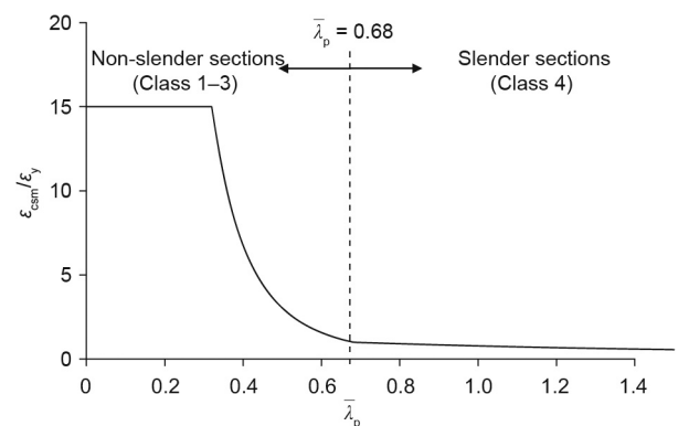
Fig. 6. CSM base curve: a continuous relationship between cross-section slenderness \bar{\lambda}_p and its deformation capacity \epsilon_{\text{CSM}}/\epsilon_y .
