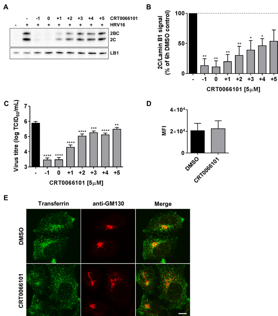
FIG 4 Effect of CRT0066101 on viral entry. (A) HeLa cells were infected with HRV16 (MOI of 20) for 6 h, and CRT0066101 (5 \mu M) was added at the following different time points: 1 h before infection (–1), during the 1-h virus infection period (0), and every hour after the time of virus adsorption (+1, +2, +3, +4, and +5). Cells extracts were prepared at the end of the 6-h replication period and analyzed by Western blotting with anti-2C and anti-LB1 antibodies. Uninfected cells and DMSO-treated cells infected for 6 h were used as controls. Data from a representative experiment from three independent repeats are shown. (B) 2C Western blots were scanned as described in Materials and Methods and quantified by using ImageJ. The mean 2C/LB1 ratio ( \pm SEM) is shown as a percentage of the value for the DMSO control from three independent experiments. (C) In parallel, virus was extracted from the cell lysates, and viral replication was quantified by endpoint titer determination (TCID 50 ). Results are the means ( \pm SEM) of data from three independent experiments, each done in triplicate. Differences between DMSO-treated cells (–) and the rest of the conditions in both panels B and C were estimated by using one-way ANOVA with Dunnett's post hoc test. *, P < 0.05 ; **, P < 0.01 ; ***, P < 0.001 ; ****, P < 0.0001 . (D) HeLa cells were grown on coverslips and pretreated with DMSO or CRT0066101 at 5 \mu M for 1 h at 37°C. Human transferrin conjugated to Alexa Fluor 488 was added at a 75- \mu g/ml final concentration, and cells were incubated at 37°C for 1 h in the presence of DMSO or CRT0066101. Cells were stained with an anti-GM130 antibody followed by an anti-mouse antibody coupled to Alexa Fluor 546 and analyzed by confocal microscopy. Transferrin quantification is shown as the mean fluorescence intensity (MFI) from multiple low-power images. For each experiment, images from five different low-power fields with approximately 250 cells per field were quantified by using ImageJ. Data shown are the means ( \pm SEM) from three independent experiments. No statistically significant difference between DMSO- and CRT0066101-treated cells was found by performing a two-tailed t test. (E) High-power images of HeLa cells showing internalized transferrin (green) and Golgi membrane (GM130) (red) staining from a representative experiment (bar = 10 \mu m).
