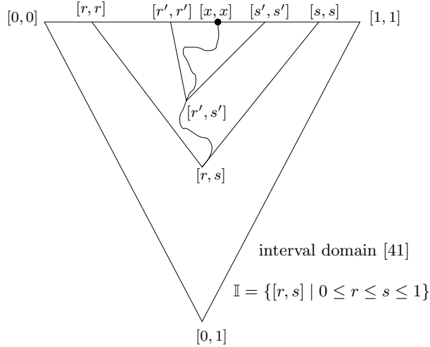
Figure 3: A schematic description of the interval domain and its order: [r, s] \leq [r', s'] iff (r \leq r' \text{ and } s' \leq s) .
