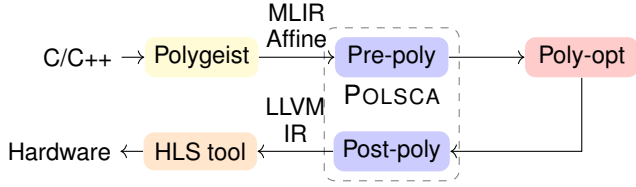
Fig. 7: The overall workflow of POLSCA. Our contributions are highlighted in the dashed region. Pre-poly and post-poly are the transformations described in Section IV.
