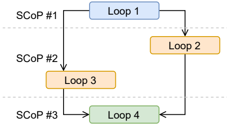
Fig. 4: Demonstrating the SCoP decomposition algorithm. In this particular example, we have 4 consecutive loops at the same depth, and there are interdependencies (arrows) among loop 1 and 2, 1 and 3, 2 and 4, 3 and 4. The minimum cuts required for SCoP covering loop 2 and 3 is 0, which will propagate through Eq. (1) and lead to the optimal solution as shown that uses 2 cuts (dashed horizontal lines).
