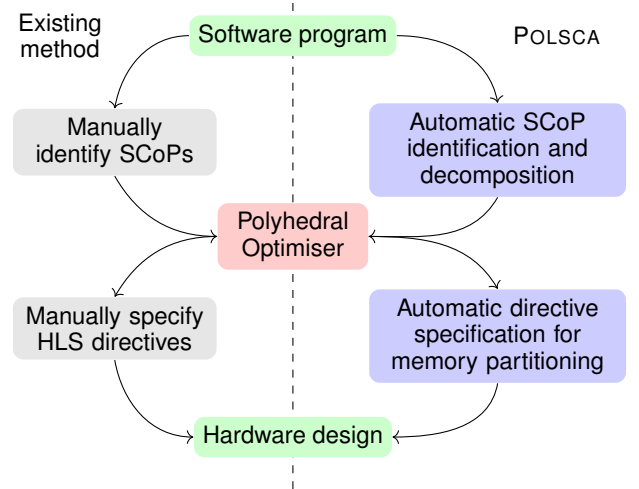
Fig. 1: Summary of our contributions (right) in polyhedral HLS compared with existing methods (left).
