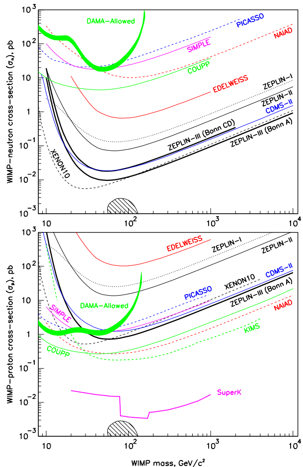
FIG. 1: Upper limits on pure WIMP-neutron and WIMP-proton SD cross-sections. In addition to ZEPLIN-III with both nn potentials, we show other xenon experiments in black: ZEPLIN-I [22], ZEPLIN-II [23] and XENON10 (Bonn A) [18, 19]. Additional curves are CDMS-II [24], COUPP [25], EDLEWEISS [26], KIMS [27], NAIAD [28], PICASSO [29] and SIMPLE [30]. The pure-proton indirect limit from Super-Kamiokande is also shown [31]. The DAMA evidence region interpreted as a nuclear recoil signal in a standard halo [7] is indicated in green. The hatched area is the tip of the 95% probability region for neutralinos in the Constrained Minimal Supersymmetric Standard Model (CMSSM) [32].
