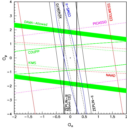
FIG. 2: Allowed regions in the a_n - a_p parameter space for 50 GeV WIMP mass.
