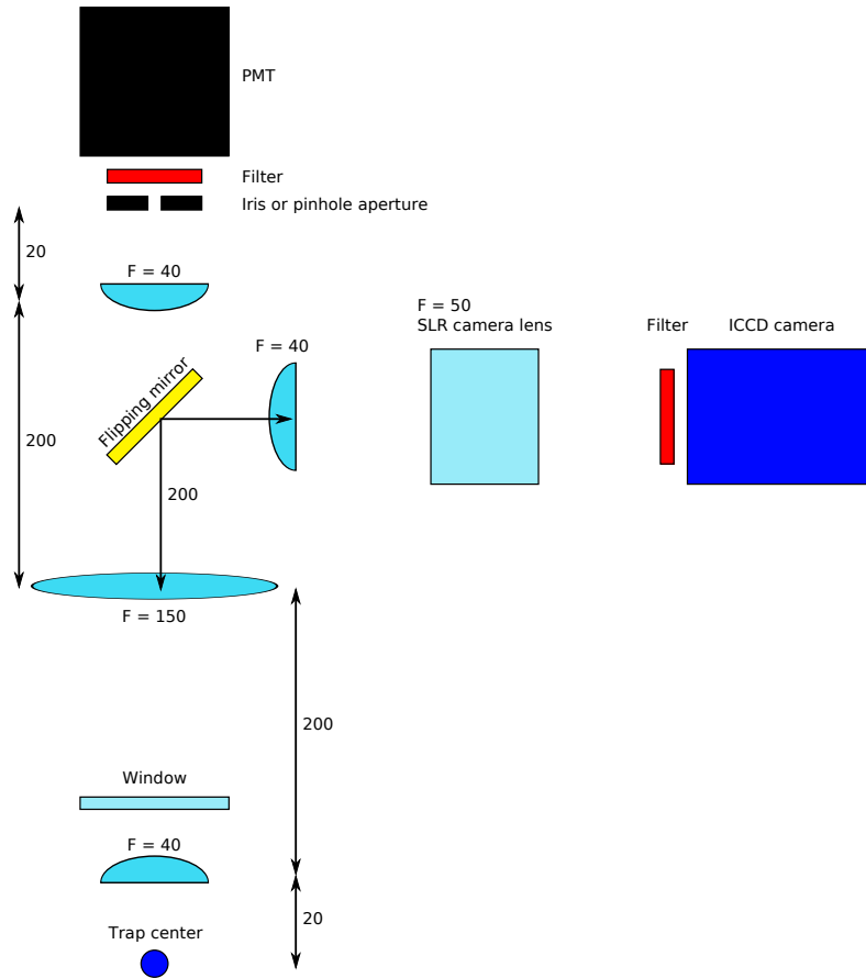
Figure 2.16: Schematic of the imaging system for fluorescence collection. All dimensions in mm.
