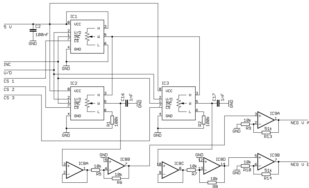
Figure 4.19: Partial schematic of voltage source generator.
