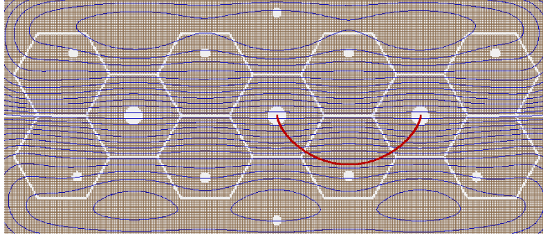
Figure 4.10: Example of an ion trajectory while moving from one trap to the next. Lines of equipotential in the mid-plane between the two boards are shown in blue. The x axis is horizontal while the y axis is vertical.
