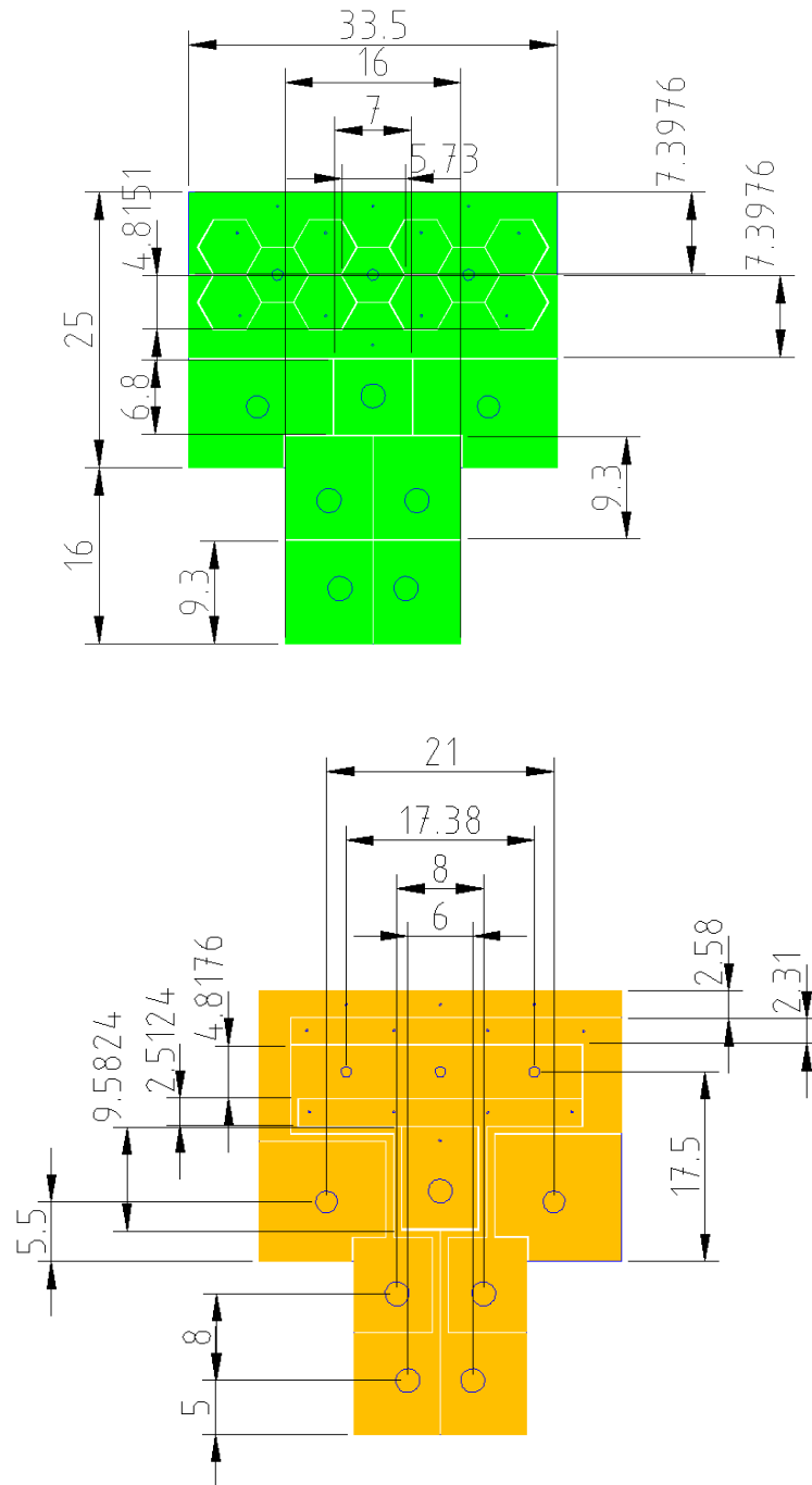
Figure 4.2: PCB trap board design to scale, with dimensions in mm. The green side faces into the trapping region, the orange side is the rear. The x axis is horizontal while the y axis is vertical. Note that a mirrored version is used for the opposing board.
