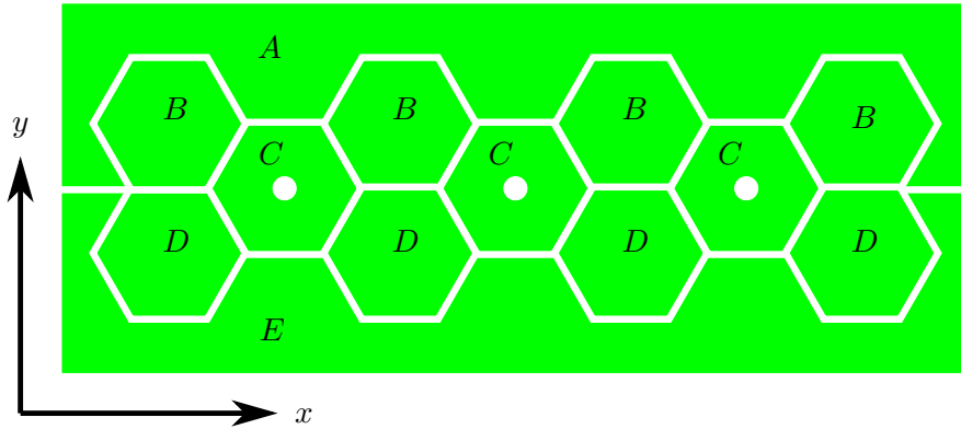
Figure 4.1: Upper part of the PCB trap board design, with electrodes labelled.
