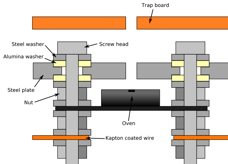
Figure 4.7: Schematic of the system used to hold the atomic beam oven in place. The electron beam filament is held in an identical way.
