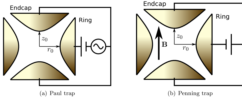
Figure 1.1: Schematic view of a Paul trap and a Penning trap. A cross section in the xz plane is shown. The traps have cylindrical symmetry about the z axis (vertical). The typical voltage polarities for trapping positive ions are shown.
