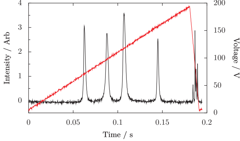
Figure 2.12: The transmission of a cavity (black) coupled to four lasers as the cavity length is scanned by scanning the voltage (red) of a piezoelectric crystal.
