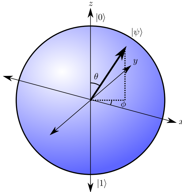
Figure 1.7: Bloch sphere representation of a qubit.
