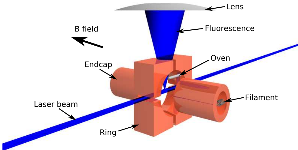
Figure 2.13: Schematic of the split-ring trap. Figure courtesy of H. Ohadi [52].
