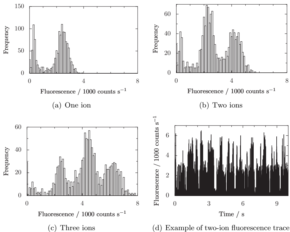
Figure 3.3: Histograms from 40 seconds of data collection with 30 ms time bins show discrete levels of fluorescence rate for small numbers of trapped ions. (d) shows ten seconds of fluorescence (10 ms time bins) from two ions; two levels of signal (plus the background level) can clearly be seen.
