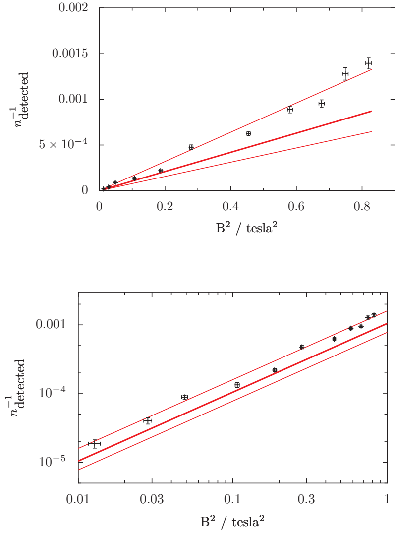
Figure 5.7: Normalised shelving rate. The theoretical prediction assuming a detection efficiency of 0.04 \pm 0.014\% is shown in red. Both linear and log-log scales are shown for clarity.
