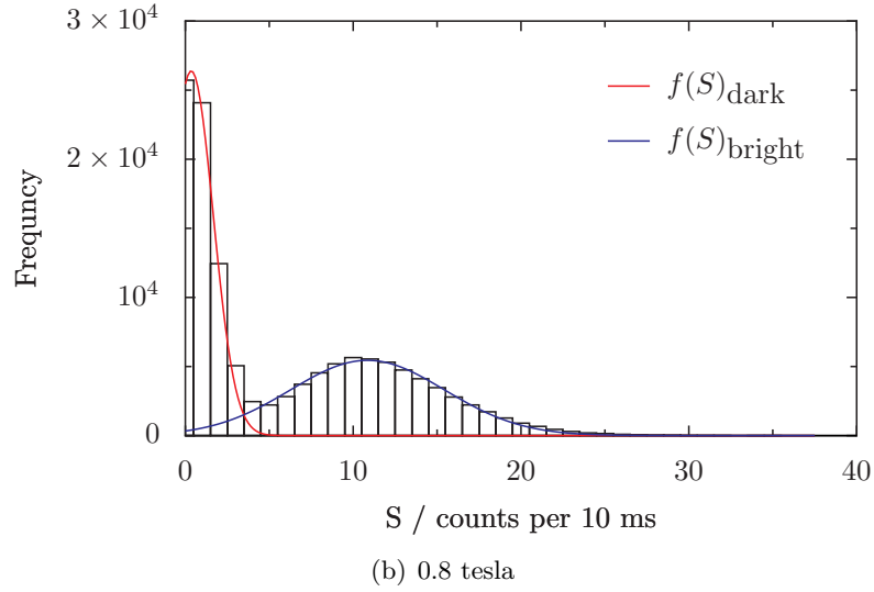
Figure 5.5: Distribution of fluorescence levels from a single \text{Ca}^+ ion. At high mean values, a Poisson distribution converges to a Gaussian distribution. The data has been fit to f(S) = f(S)_{\text{dark}} + f(S)_{\text{bright}} , where f(S)_{\text{dark}} and f(S)_{\text{bright}} are separate Gaussian functions.
