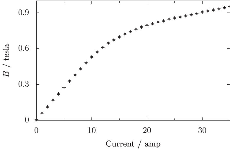
Figure 2.15: Magnetic field strength as a function of electromagnet coil current.
