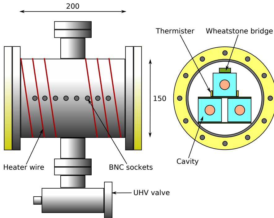
Figure 2.10: Vacuum chamber for housing the reference cavities. Dimensions in mm.
