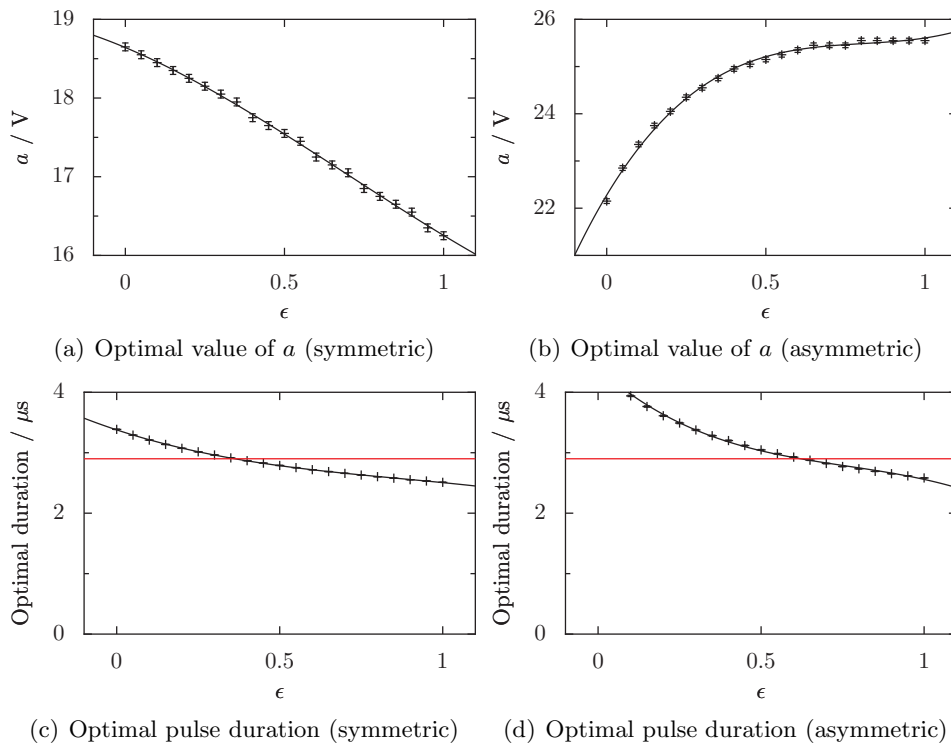
Figure 4.13: Simulated optimal voltage and timing parameters for B = 0.9 tesla. The true cyclotron period is also shown as a red line in (c) and (d).
