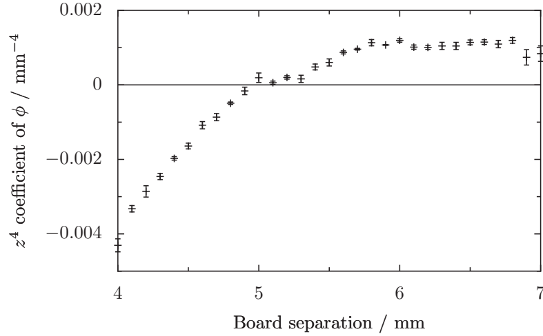
Figure 4.6: Quartic coefficient of the potential along the central axis of the PCB trap for -1 \leq z \leq 1 . The error bars show the uncertainty in the fit parameter.
