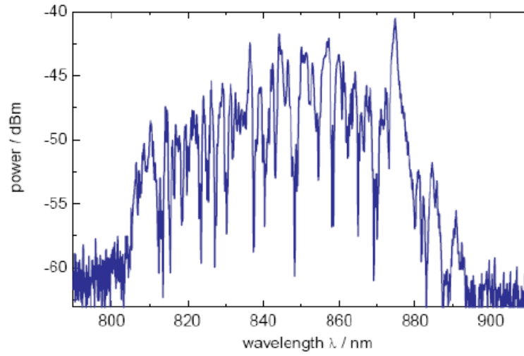
Figure 2.4: Emission Spectrum of an Eagleyard Photonics EYP-RWE-0870-06010-0750-SOT01-0000 laser diode without external feedback. Taken from [59].
