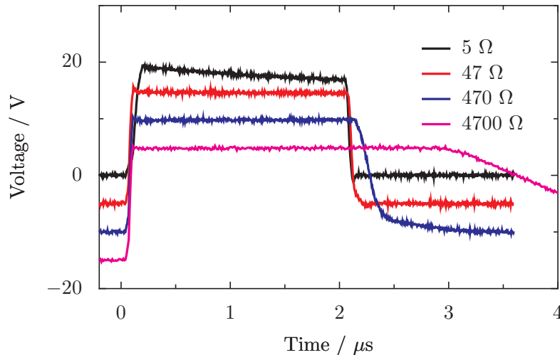
Figure 4.18: Example 20 volt pulses for various resistances, R2. Graphs are offset for clarity. The apparent voltage noise appears similar when measuring a clean 20 volt DC source, so the noise is most likely due to RF pickup and/or imperfections in the oscilloscope.
