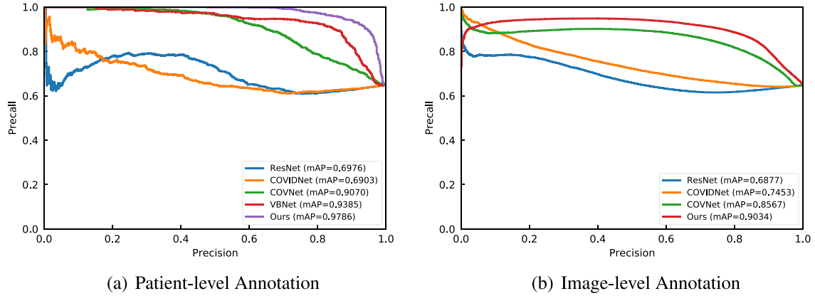
Fig. 12. The Precision–Recall (PR) curves of different compared methods.
