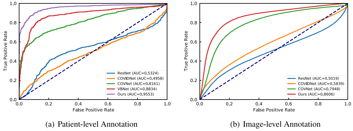
Fig. 11. The Receiver Operating Characteristic (ROC) curves of different compared methods.
