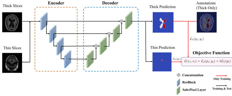
Fig. 9. Overview of our proposed XAI model for explainable segmentation. Here ResBlock represents the residual block proposed in the ResNet [165].
