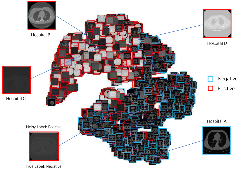
Fig. 14. T-SNE visualisation [182] of the learnt features from CT images. Original images are sampled from four different hospitals and represented in the figure. Besides, a falsely annotated image is drawn from the negative cluster.
