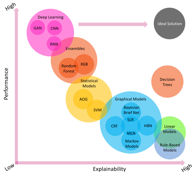
Fig. 5. Model explainability vs. model performance for widely used machine learning and deep learning algorithms. The ideal solution should have both high explainability and high performance. However, existing linear models, rule-based models and decision trees are more transparent, but with lower performance in general. In contrast, complex models, e.g., deep learning and ensembles, manifest higher performance while less explainability can be obtained. HBN: Hierarchical Bayesian Networks; SLR: Simple Linear Regression; CRF: Conditional Random Fields; MLN: Markov Logic Network; SVM: Support Vector Machine; AOG: Stochastic And-Or-Graphs; XGB: XGBoost; CNN: Convolutional Neural Network; RNN: Recurrent Neural Network; and GAN: Generative Adversarial Network.
