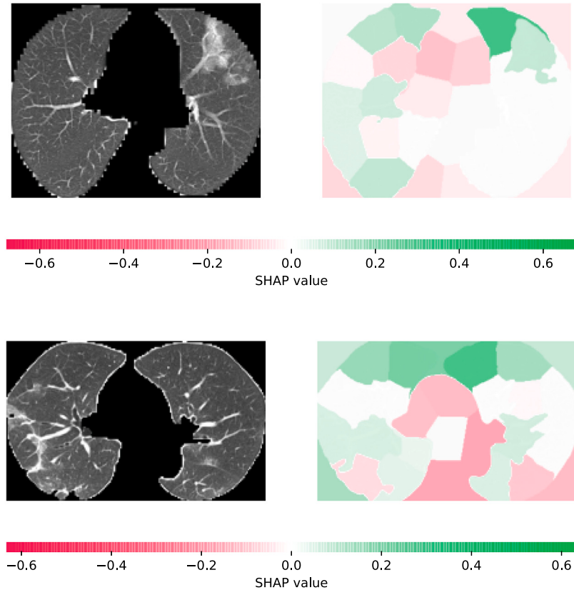
Fig. 16. The SHAP values for different super-pixels of the sampled images. We computed the SHAP values through the Kernel SHAP method [183]. The super-pixel with positive SHAP value indicates the positive impact to the positive prediction, while the negative value means that the super-pixel contributes to the negative prediction.
