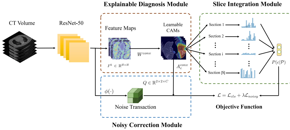
Fig. 8. The overview of our proposed model. P(c | S_i) denotes the probability of the Section S_i , and P(c | \mathcal{P}) represents the probability of the patient who is COVID-19 infected or not. Q \in \mathbb{R}^{2 \times 2 \times C} indicates the noise transaction from the probability of the true label P(y_c | I) to the noise label P(z_c | I) . Besides, \phi(\cdot) is a non-linear feature transformation function, which projects the feature into embedding space.
