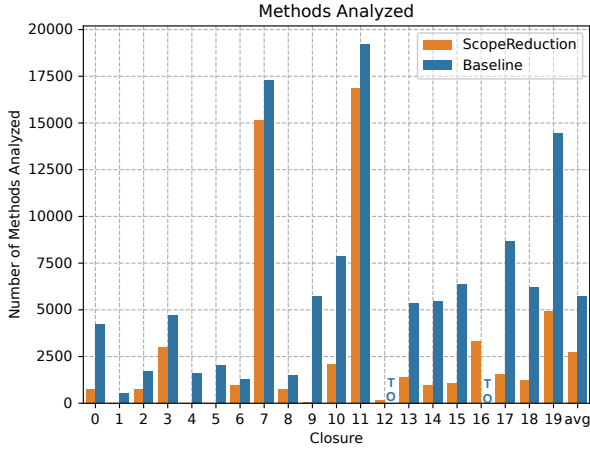
Figure 3: Number of methods analyzed, with and without scope-reduction analysis, for Maven closures. TO stands for
