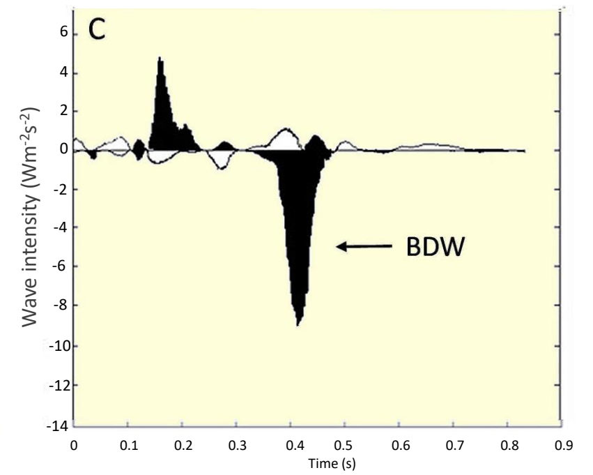
Wave intensity
