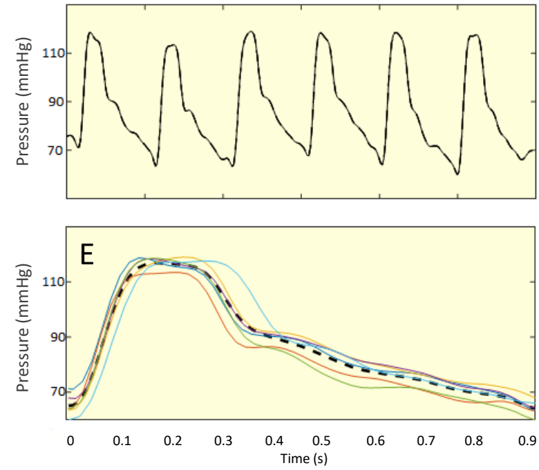
Central Pressure
