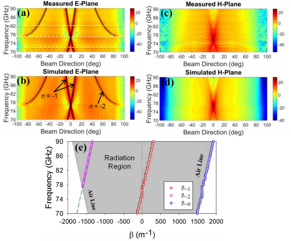
Figure 2. Experimental gain in dB for E-plane (a) and H-plane (c) as a function of angle and frequency. Simulated realized gain in dB for E-plane (b) and H-plane (d) as a function of angle and frequency. Dispersion diagram for modes n = 0 (blue circles), n = -1 (red circles) and n = -2 (pink circles) extracted from the measured beaming direction (e). Gray area indicates the fast wave or radiation region. Green dashed lines correspond to the analytically calculated phase constants.
