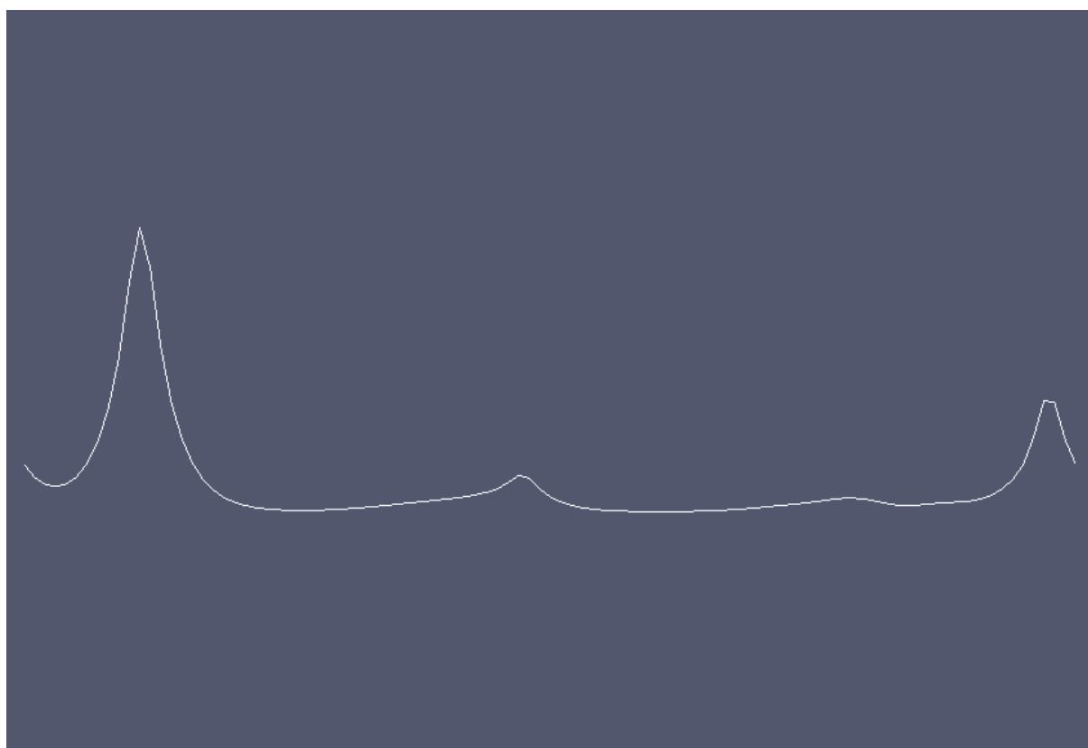
Figure3: Solution at t = 5.3 .
