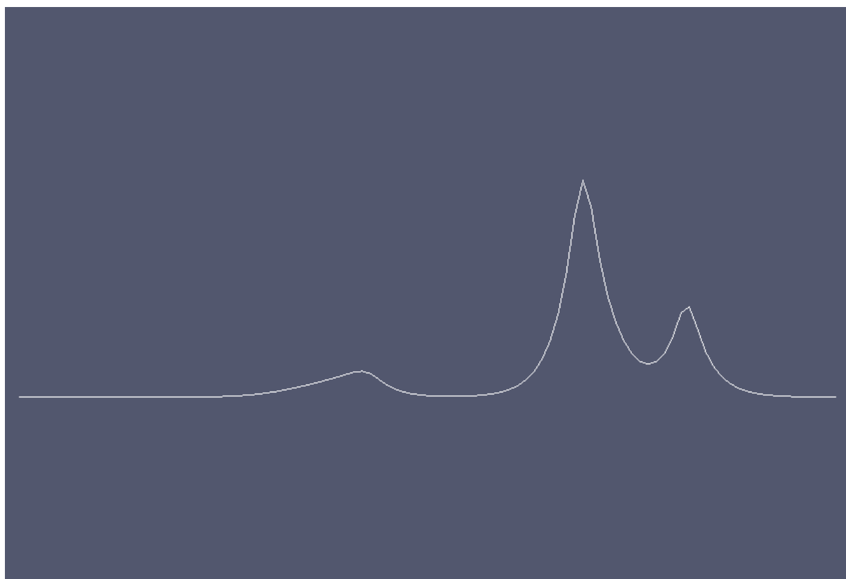
Figure2: Solution at t = 2.5 .
