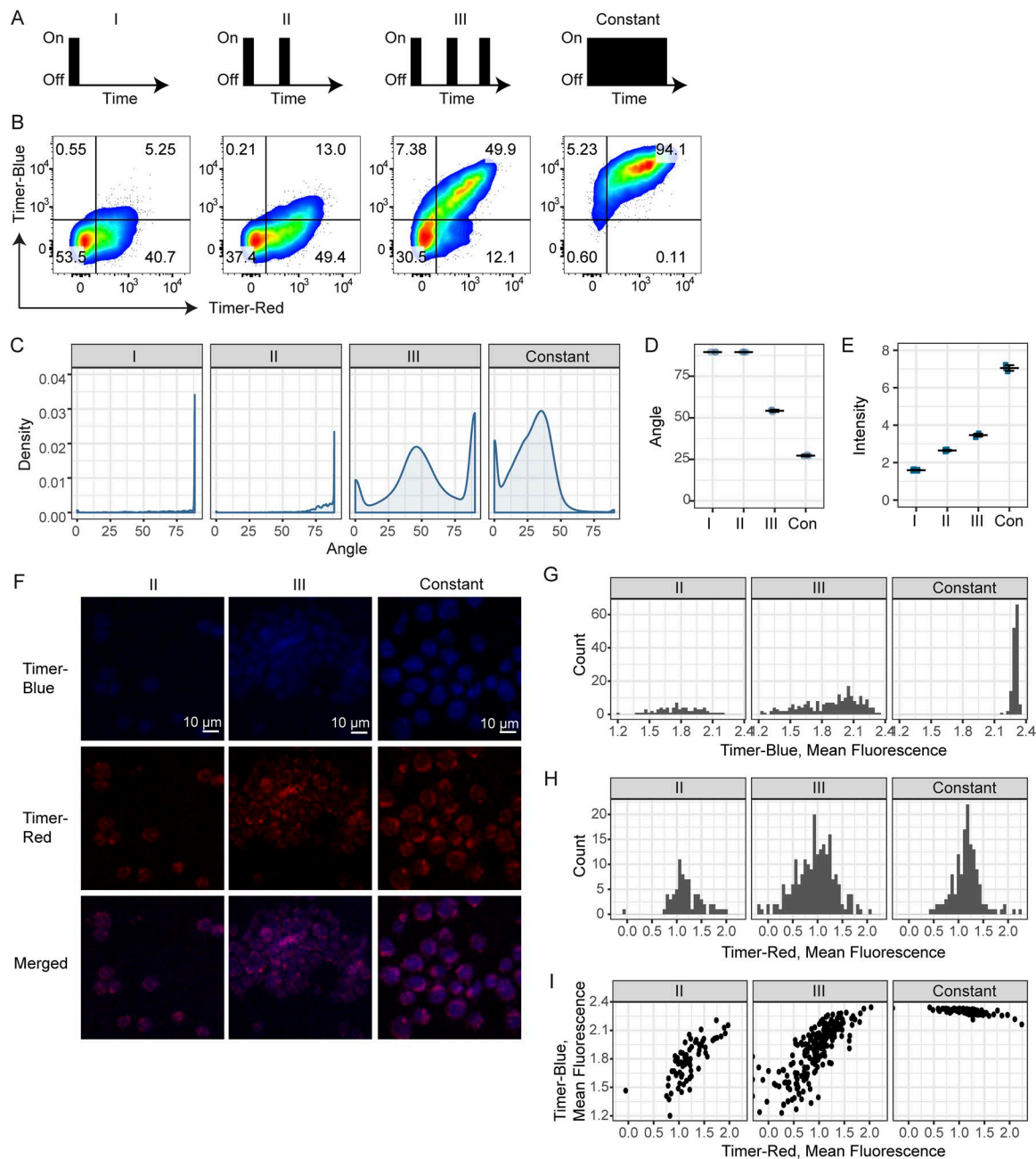
Figure 4. Nr4a3 -Tocky captures the frequency domain of TCR signaling. (A–I) T cells from OTII Nr4a3 -Tocky mice were cultured with T cell-depleted splenocytes. (A) T cells were stimulated with 1 \mu M Ova as follows: 4-h stimulation, then rested for 48 h (I); 4-h stimulation, 20-h rest, 4-h stimulation, and 24-h rest (II); 4-h stimulation, 20-h rest, 4-h stimulation, 20-h rest, and 4-h stimulation (III); or 2-d constant (Con) stimulation. During resting stages, cells were incubated with 100 U/ml recombinant IL-2 and 20 \mu g/ml anti-MHC II and washed before and after stimulations. (B) Cells were then harvested and CD4 + OTII T cells analyzed for Timer-blue versus Timer-red fluorescence expression by flow cytometry. (C) Displayed are the Timer Angle distributions for the four culture conditions. (D and E) Shown are the mean Timer Angle (D) or Timer Intensity (E) within the four different cultures. Error bars represent mean \pm SD; n = 3 culture triplicates. (F) Confocal microscopy analysis of OTII Nr4a3 -Tocky stimulated with various frequencies. The same cell samples used in A–D were analyzed by confocal microscopy. Bars, 10 \mu m. (G and H) Histogram showing the mean fluorescence intensity of Timer-blue (G) or Timer-red fluorescence (H) in single cells by microscopic image analysis. (I) 2D plots of the mean fluorescence intensities of Timer-blue and Timer-red fluorescence in single cells by microscopic image analysis. Cells were identified as regions of interest, and mean fluorescence intensities were measured and logged. See Fig. S2 and Materials and methods for details.
