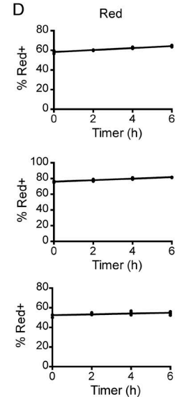
Figure 2. Antigen-receptor ligation induces Timer proteins in B and T cell subsets from Nr4a3 -Tocky mice. (A) Construct for generating Nr4a3 -Tocky BAC transgenic mice. (B) Splenocytes from Nr4a3 -Tocky mice were activated for 20 h with either 10 \mu g/ml of soluble goat anti-mouse IgM (for CD19 + B cells) or 2 \mu g/ml plate bound anti-CD3 (for CD4 + and CD8 + T cells). Cells were then incubated with 100 \mu g/ml cycloheximide to inhibit new protein translation and the decay of blue fluorescence measured over time by flow cytometry. Shown is Timer-blue versus Timer-red fluorescence in CD19 + B cells (top), CD4 + T cells (middle), or CD8 + T cells (bottom) at the indicated time points. (C and D) Summary data of the percentage of cells blue + (C) or red + (D) cells in the cultures. Linear regression by Pearson's correlation; n = 3 culture triplicates. Data are representative of two independent experiments.
