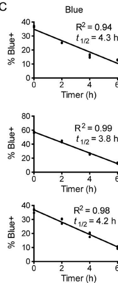
Figure 2. Antigen-receptor ligation induces Timer proteins in B and T cell subsets from Nr4a3 -Tocky mice. (A) Construct for generating Nr4a3 -Tocky BAC transgenic mice. (B) Splenocytes from Nr4a3 -Tocky mice were activated for 20 h with either 10 \mu g/ml of soluble goat anti-mouse IgM (for CD19 + B cells) or 2 \mu g/ml plate bound anti-CD3 (for CD4 + and CD8 + T cells). Cells were then incubated with 100 \mu g/ml cycloheximide to inhibit new protein translation and the decay of blue fluorescence measured over time by flow cytometry. Shown is Timer-blue versus Timer-red fluorescence in CD19 + B cells (top), CD4 + T cells (middle), or CD8 + T cells (bottom) at the indicated time points. (C and D) Summary data of the percentage of cells blue + (C) or red + (D) cells in the cultures. Linear regression by Pearson's correlation; n = 3 culture triplicates. Data are representative of two independent experiments.
