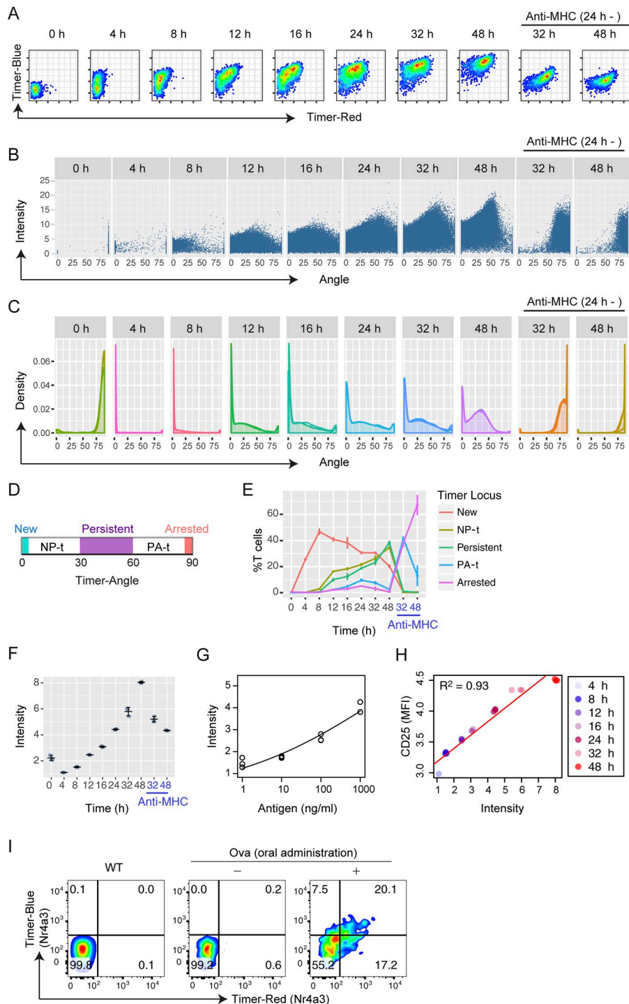
Figure 3. Nr4a3-Tocky reveals the time domain of TCR signal-triggered activation and differentiation events. (A) Flow cytometric analysis of blue and red Timer raw fluorescence in antigen-stimulated OT-II Nr4a3-Tocky T cells. T cells were stimulated for the indicated time points with 1 \mu M Ova peptide. In some cultures, anti-MHC II antibodies were added at 24 h to terminate TCR signaling. (B) Trigonometric-transformed data from A. Individual cells are plotted against Timer Angle and Timer Intensity. (C) Density plot of Timer Angle from the transformed data. (D) The designation of the five Timer loci by Timer Angle \theta as follows: New ( \theta = 0^\circ ), NP-t ( 0^\circ < \theta < 30^\circ ), Persistent ( 30^\circ \leq \theta < 60^\circ ), PA-t ( 60^\circ \leq \theta < 90^\circ ), and Arrested ( \theta = 90^\circ ). (E) Timer Locus analysis to show the frequency of cells within the five Timer loci defined in C. (F) Summary of Timer Intensity in the cultures from A over time. (G) Dose-response curve of Timer Intensity on stimulation with titrated doses of Ova peptide (antigen). OT-II Nr4a3-Tocky T cells were stimulated for 22 h in the presence of 1, 10, 100, or 1,000 nM Ova peptide and APCs. Data were fitted to a dose-response curve with a statistical significance by a lack-of-fit test ( P = 0.014 ). (H) Scatter plot of Timer Intensity versus cell surface CD25 expression. Linear regression analysis showed a strong correlation ( R^2 = 0.93 ). See legend for sample identities. (I) CD4 + T cells from OT-II TCR transgenic Nr4a3-Tocky mice were adoptively transferred into CD45.1 congenic mice, which were fed Ova or control for 3 d. CD45.2 + CD45.1 + CD4 + OT-II Nr4a3-Tocky T cells within mesenteric lymph nodes were analyzed for Timer expression. Error bars represent mean \pm SD; n = 3 culture triplicates. Data are representative of at least two independent experiments.
