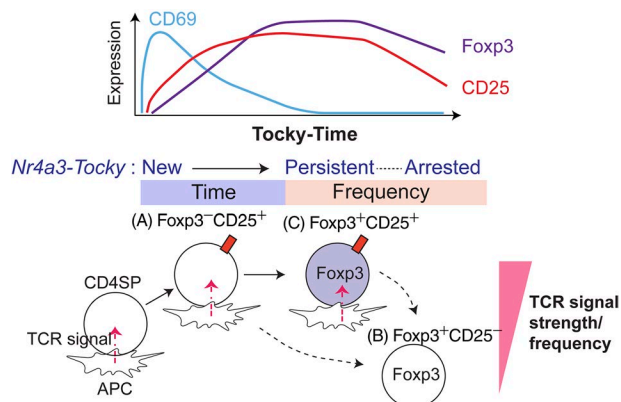
Figure 7. Model for the influence of TCR signaling dynamics on thymic Treg cell differentiation.
