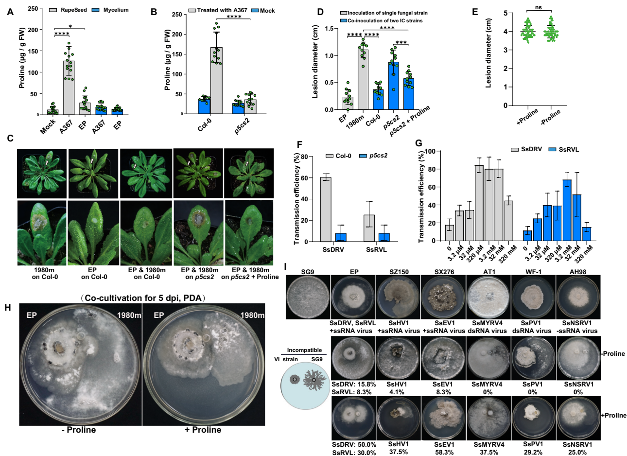
Fig. 3 | Plant-derived proline increases upon S. sclerotiorum infection and promotes mycovirus transmission. A Proline content of oilseed rape plants inoculated by HAVs-free virulent strain Ep-IPNA367 (A367) and HAVs-infected hypovirulent strain Ep-IPN (EP) at 24 hpi, and of Ep-IPNA367 and Ep-IPN mycelia ( n = 15 ). B Proline content of A. thaliana Col-0 wildtype and p5cs2 mutant inoculated by Ep-IPNA367 at 24 hpi ( n = 11 ). C Virulence assay of strains 1980m, Ep-IPN, and Ep-IPN and 1980m co-inoculation (Ep & 1980m) on A. thaliana Col-0 wildtype and p5cs2 mutant, and virulence assay of Ep & 1980m co-inoculation on the p5cs2 mutant following spraying with exogenous proline (36 hpi, 20 °C) ( n = 14 ). The lesions indicated by white arrows in the upper panel were enlarged in the lower panel. D Diameters of lesions caused by Ep-IPN and 1980m co-culture on A. thaliana Col-0 wildtype, p5cs2 mutant, and p5cs2 mutant plus proline (36 hpi, 20 °C) ( n = 11 ). E Diameters of lesions caused by 1980m with or without proline on oilseed rape (72 hpi, 20 °C), illustrating that proline addition does not induce plant resistance to S. sclerotiorum infection ( n = 57 ). F Transmission efficiency of two mycoviruses, SsDRV and SsRVL, from Ep-IPN to 1980m on A. thaliana Col-0 wildtype and p5cs2 mutant ( n = 3 for independent experiments, N = 8 for co-cultures). G Transmission efficiency of two mycoviruses, SsDRV and SsRVL, from Ep-IPN to
