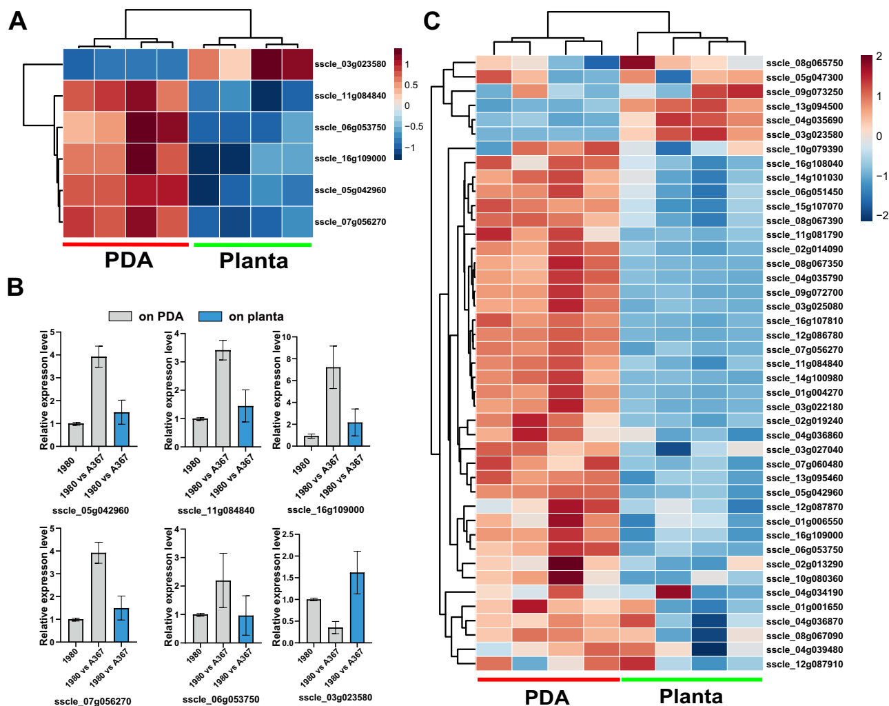
Fig. 2 | Plant suppresses expression of fungal G protein and vic-related genes upon S. sclerotiorum infection. A Expression cluster analysis of S. sclerotiorum genes encoding G protein subunits in 1980 and Ep-IPN co-cultures in vitro and in planta. B Expression levels of genes encoding G protein subunits in 1980 alone, and 1980 and Ep-IPN co-culture in vitro and in planta. Data are presented as mean \pm SD, two-tailed Student's t test. n = 3 biologically repetitions. C Expression cluster
