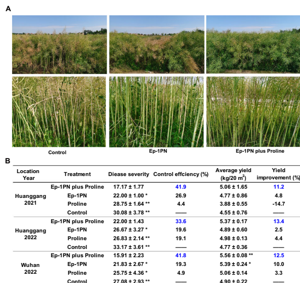
Fig. 5 | Proline enhances the biological efficacy of HAVs against Sclerotinia stem rot of oilseed rape and improves yield. A Symptoms of Sclerotinia stem rot on oilseed rape after spraying with hyphal fragment suspensions of Ep-1PN with and without proline. In the upper panel, grayish-yellow colors signify diseased plants; in the lower panel, grayish-yellow discoloration of stems is evident and caused by S. sclerotiorum . B Application of Ep-1PN with and without proline improved yield and suppressed stem rot in field experiments as compared to controls (proline and
