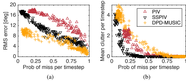
Fig. 13. The effect of varying the estimate acceptance threshold on the relationship between (a) RMS error and miss rate, and (b) clutter rate and miss rate for each algorithm ( \Delta : PIV, \nabla : SSPIV, + : DPD-MUSIC).
