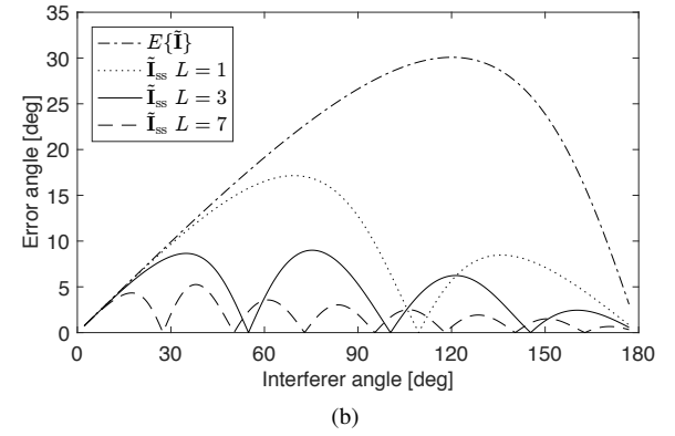
Fig. 2. Error in E\{\tilde{\mathbf{I}}\} and \tilde{\mathbf{I}}_{ss} for for L = \{1, 3, 7\} as function of \angle(\mathbf{x}_1, \mathbf{x}_2) with (a) SIR 20 dB and (b) SIR 3 dB.
