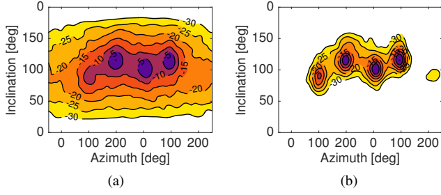
Fig. 15. Smoothed histogram of (a) PIVs and (b) SSPIVs for observation interval at 14 s in experiment 1. Contours indicate histogram values in dB with respect to maximum value. Colormap is the same in both plots.
