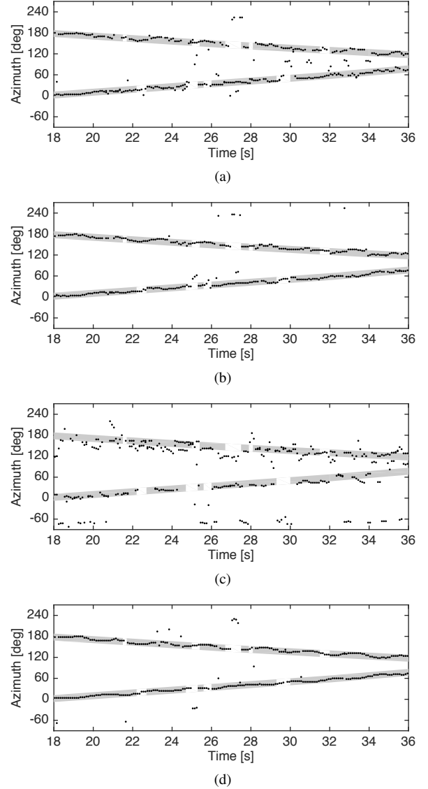
Fig. 17. Estimated DOAs as a function of time for (a) PIV, (b) SSPIV (c) PWD-SRP and (d) DPD-MUSIC using a 0.25 s observation interval for two moving sources. Grey lines indicate ground truth trajectory and voice activity.
