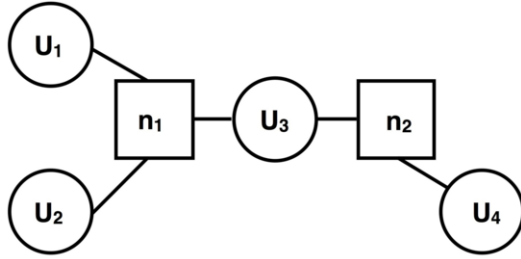
Figure 1. An example of four UAVs ( u_1 – u_4 ) interacting via a max-sum factor graph. Trees are grown for n_1 and n_2 .
