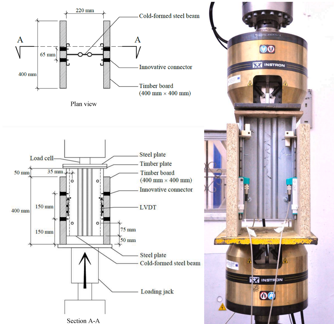
Fig. 9. Push-out test setup.
