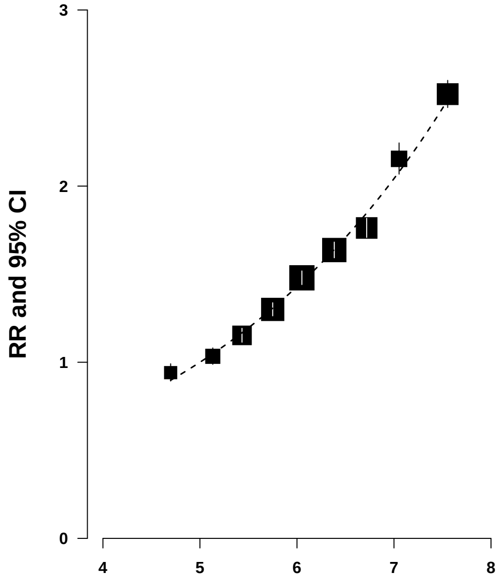
Arithmetic scale: curvilinear association
