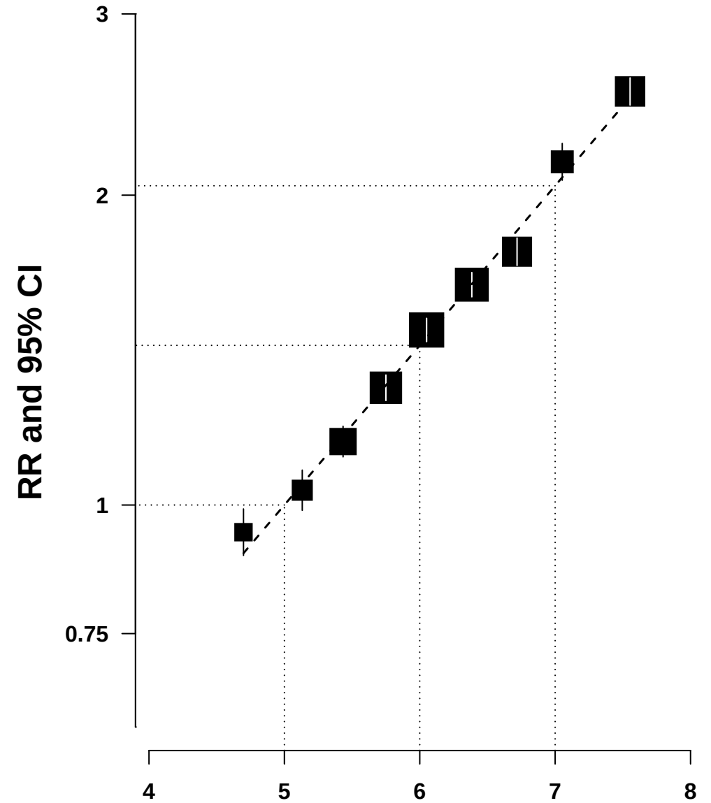
Logarithmic scale: linear association
