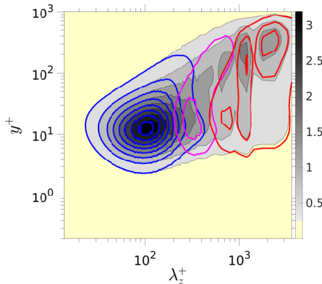
FIGURE 1. Premultiplied spanwise spectral maps for the streamwise turbulent fluctuations: grey contours represent the total field; blue, magenta and red iso-lines represent, respectively, sub-spectra for small-scale (SS), intermediate-scale (IS) and large-scale (LS) fluctuations.
