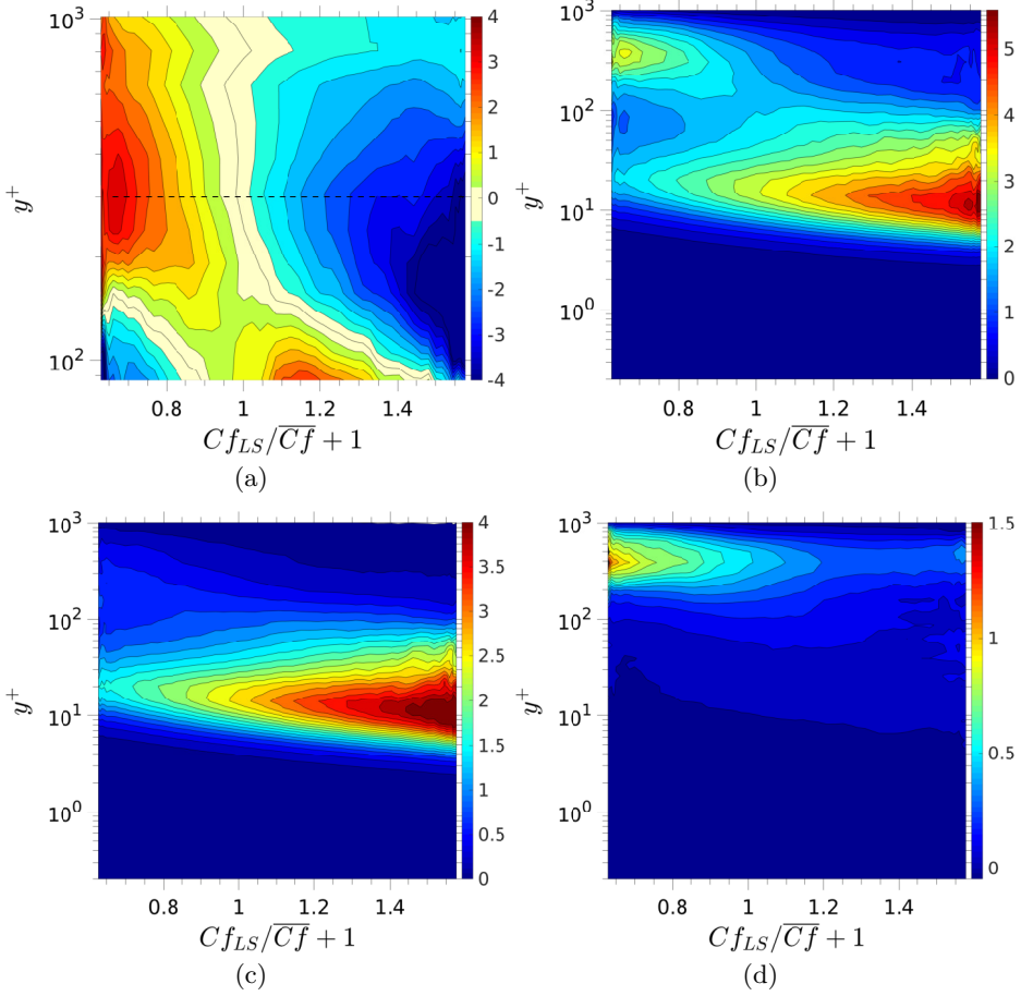
FIGURE 10. Alternative forms of the conditional production rates of the streamwise stress: (a) wall-normal gradient of the incremental large-scale velocity profile, conditional on Cf_{LS} , \frac{d(\overline{U}^+|_{Cf_{LS}} - \overline{U}^+|_{Cf_{LS}=0})}{dy^+} , (b) Production driven by the total shear stress, y^+ \times -\overline{uv}^+ \frac{d\overline{U}^+}{dy^+}|_{Cf_{LS}} , (c) Production driven by the small-scale shear stress, y^+ \times -\overline{u_{SS}v_{SS}}^+ \frac{d\overline{U}^+}{dy^+}|_{Cf_{LS}} and (d) Production driven by the large-scale shear stress, y^+ \times -\overline{u_{LS}v_{LS}}^+ \frac{d\overline{U}^+}{dy^+}|_{Cf_{LS}}
