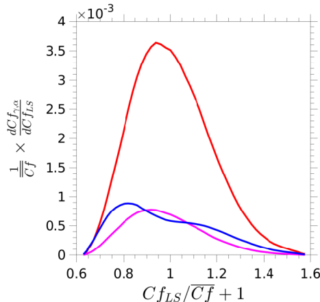
FIGURE 16. Contributions of wall-normal-integrated Cf_{LS} -wise gradients of different fragments, associated with \overline{u_\gamma u_\alpha} , to the skin friction via the RD relationship; red line: small-scale contribution; blue line: large-scale contribution; magenta line: intermediate scale contribution; the red and blue lines arise, respectively, from the y -wise integration of maps (c) and (d) in figure 13.
