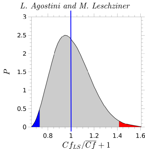
FIGURE 3. PDF of large-scale skin-friction fluctuations; the blue and red regions represents areas of 1.5% extreme negative and positive events, respectively.
