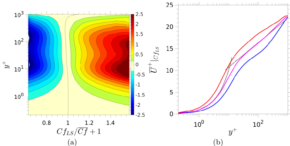
FIGURE 6. Conditional mean-velocity: (a) map of the conditional increment in the mean velocities ( \overline{U'}^+|_{Cf_{LS}} = \overline{U}^+|_{Cf_{LS}} - \overline{U}^+ ); (b) profiles of conditional mean velocity of \overline{U}^+|_{Cf_{LS}} determined over the extreme \pm 1.5\% events of the tails of the PDF in figure 3 and around the condition Cf_{LS} = 0 events, conveyed by the red, blue and magenta lines, respectively.
