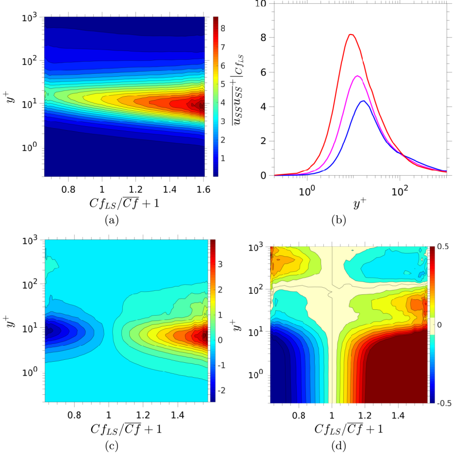
FIGURE 8. Correlation of small-scale and large-scale motions: (a) map of conditional streamwise small-scale stress \overline{u_{SS}u_{SS}^+}|_{Cf_{LS}} ; (b) profiles of conditional streamwise small-scale stress \overline{u_{SS}u_{SS}^+}|_{Cf_{LS}} averaged over the 1.5% lowest, highest and weakest Cf_{LS} events, conveyed by the blue, red and magenta lines, respectively; (c) map of increment of conditional streamwise small-scale stress \overline{u_{SS}u_{SS}^+}|_{Cf_{LS}} - \overline{u_{SS}u_{SS}^+}|_{Cf_{LS}=0} ; (d) map of normalised increment of conditional streamwise small-scale stress (\overline{u_{SS}u_{SS}^+}|_{Cf_{LS}}) / (\overline{u_{SS}u_{SS}^+}|_{Cf_{LS}=0}) - 1 .
