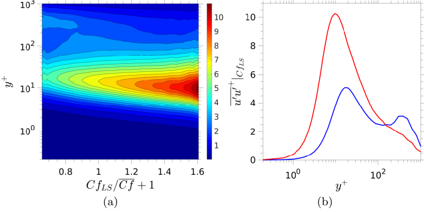
FIGURE 4. Properties of streamwise stress \overline{uu}^+|_{Cf_{LS}} : (a) map of stress derivative \overline{uu}^+|_{Cf_{LS}} across (Cf_{LS}, y^+) plane (equation 4.7); (b) wall-normal profiles of the conditional streamwise stresses obtained by integrating equation 4.7 over the blue and red 1.5% tails in figure 3.
