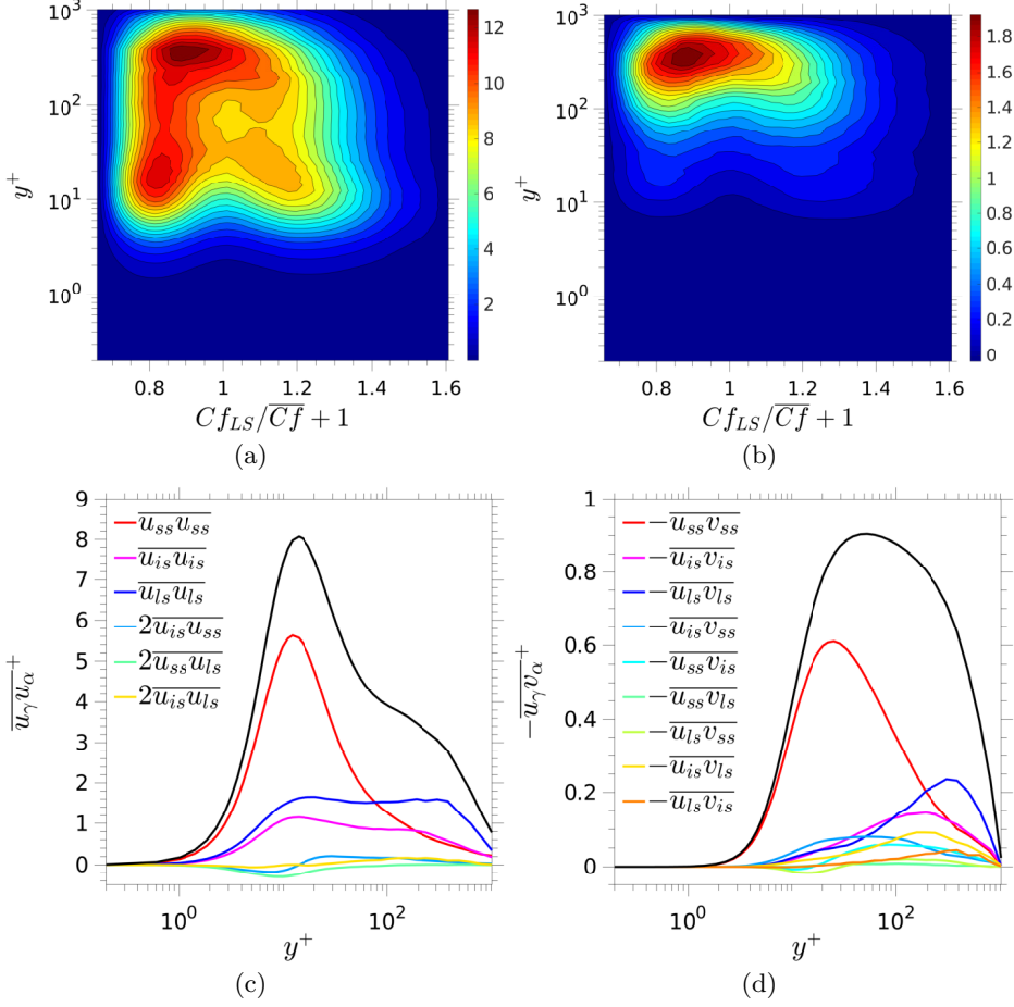
FIGURE 7. Contribution of large-scale turbulent stresses to the respective total levels: (a) map of Cf_{LS} -wise gradient of large-scale streamwise stress, \frac{du_{LS}u_{LS}^+}{dCf_{LS}} ; (b) map of Cf_{LS} -wise gradient of large-scale shear stress -\frac{du_{LS}v_{LS}^+}{dCf_{LS}} ; (c) wall-normal profiles of scale-wise contributions to streamwise stress; (d) wall-normal profiles of scale-wise contributions to shear stress.
