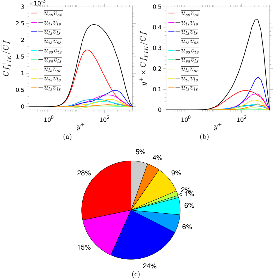
FIGURE 12. Contribution of different scales to the skin friction via the FIK identity: (a) contribution of different shear-stress fragments to the integrand in the FIK identity; (b) same as (a), but premultiplied by y^+ ; (c) contributions of different scales to Cf ; the grey segment represents the viscous part, i.e. the leading term in equation 4.8).
