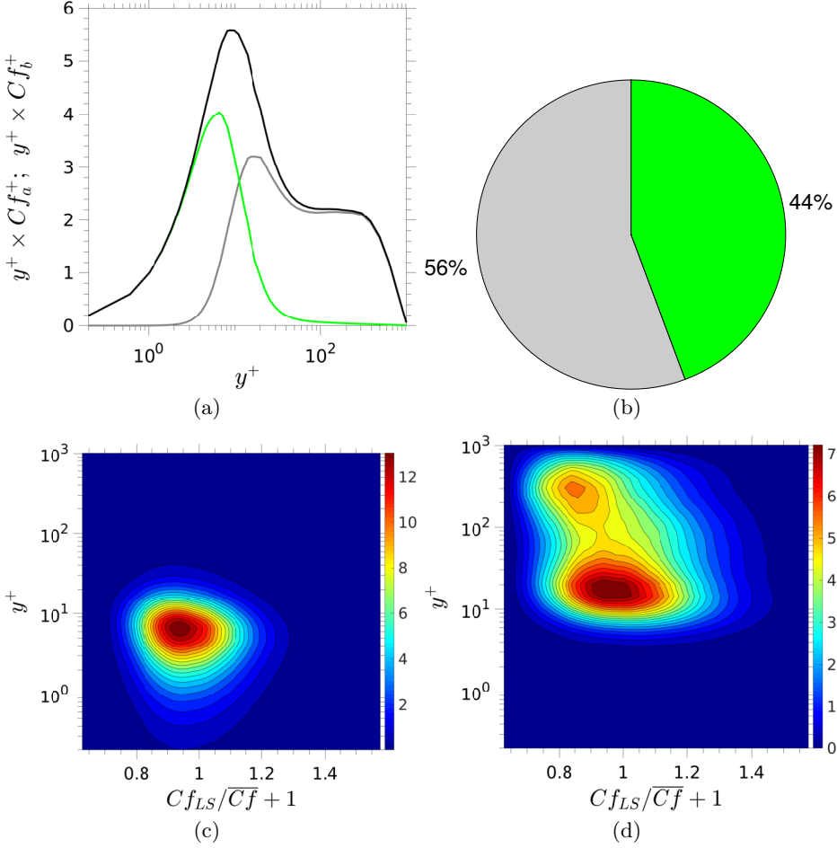
FIGURE 14. (a) Contributions of viscous and turbulent terms to the skin friction as derived from the RD relationship; (a) wall-normal profiles of pre-multiplied integrands Cf_a^+ and Cf_b^+ in equation 4.9; (b) contribution of viscous and turbulent terms to the skin friction (i.e. integrals of Cf_a^+ and Cf_b^+ ; (c) map of y^+ \times \frac{dCf_a^+}{dCf_{LS}} , (d) map of y^+ \times \frac{dCf_b^+}{dCf_{LS}} .
