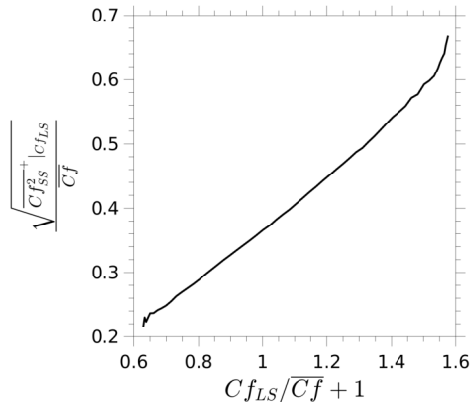
FIGURE 9. Standard deviation of small-scale skin-friction fluctuations conditional on large-scale skin-friction fluctuations.
