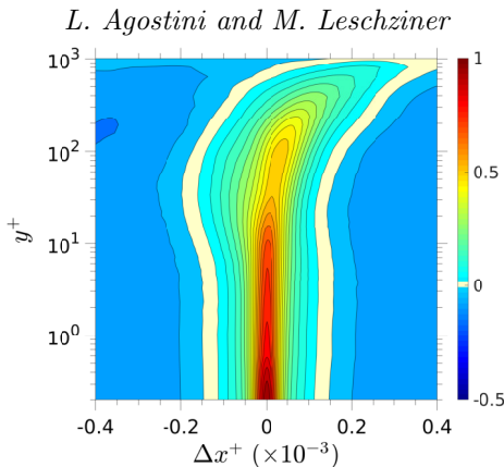
FIGURE 5. Map of two-point correlation between Cf_{LS} and u_{LS}(y^+) in the (y^+, \Delta x) plane, with y = 0 the reference point.
