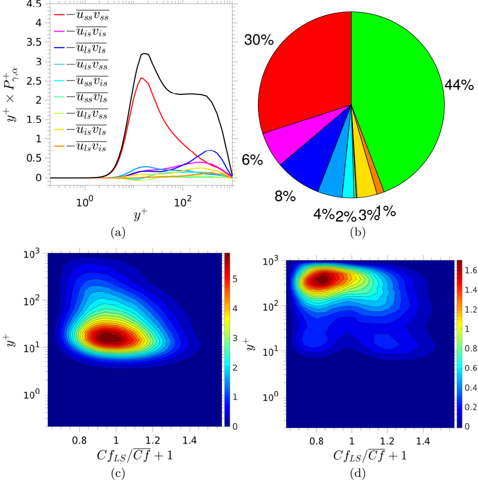
FIGURE 15. Contributions of scale-related turbulent shear-stress fragments to the skin friction via the RD relationship; (a) wall-normal profiles of scale-specific pre-multiplied production contributions to the integrand Cf_b^+ in equation 4.9; (b) contribution of fragments to the skin friction; (c) map of y^+ \times \frac{dCf_{b,SS}^+}{dCf_{LS}} associated with the small-scale shear-stress fragment; (d) map of y^+ \times \frac{dCf_{b,LS}^+}{dCf_{LS}} associated with the large-scale shear-stress fragment.
