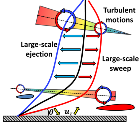
FIGURE 17. Conceptual schematic of the effects of large-scale fluctuations on the strain rate and consequent amplification/attenuation of near-wall and outer-layer turbulence
