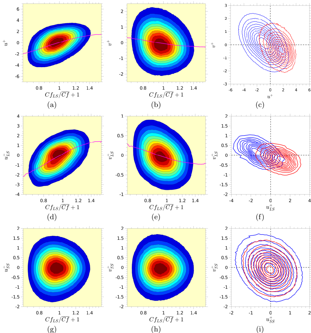
FIGURE 11. PDFs of turbulent-velocity fluctuations at y^+ \approx 300 : (a) joint PDF P(u^+, Cf_{LS}) ; (b) joint PDF P(v^+, Cf_{LS}) ; (c) joint PDFs P(u^+, v^+) derived from joint PDF P(u^+, v^+, Cf_{LS}) at the extreme positive and negative 5% of the Cf_{LS} tails; magenta lines in (a) and (b) are loci of the conditional averages \overline{U'}^+|_{Cf_{LS}} and \overline{V'}^+|_{Cf_{LS}} , respectively; (d)(g), (e)(h) and (f)(i) correspond to (a),(b) and (c), respectively, but pertain to the large scale and small-scale fluctuations, respectively.
