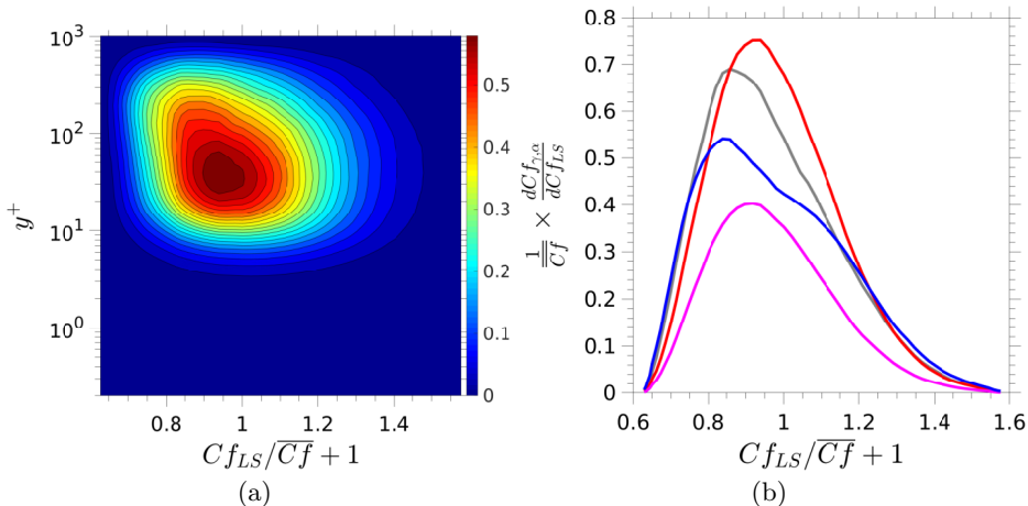
FIGURE 13. Conditional contributions to the skin friction via the FIK identity: (a) Wall-normal distribution of the Cf_{LS} -wise gradient of skin friction, \frac{dCf_{FIK}}{dCf_{LS}} ; (b) wall-normal-integrated Cf_{LS} -wise gradients of contributions of different scales, associated with \overline{u_\gamma u_\alpha} , to Cf (i.e. the y^+ -integral of the field in map (a)); colours of lines correspond to the those in figure 12, except for the grey line, which represents the sum of all other contributions (i.e. mixed-scale terms).
