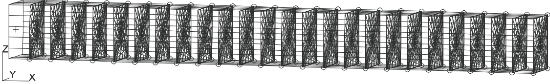
Figure 2: FEM model for L = 10 and h = 1 , showing rigid links (RBE3) to interpolate sectional displacements/rotations on nodes along centre line.
