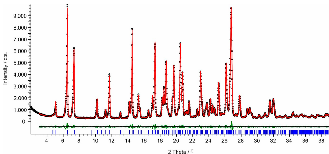
Figure 5. For the hkl reflections ( R_{wp} = 3.91\% ) between the reflection PEXRD data of CARB/TELZ with a model consisting of the cell parameters derived from indexing. Black dots indicate raw data, while the red line indicates the calculated model. The difference pattern is shown in green. Tick marks (blue) are the 2\theta positions for the hkl reflections Pawley fit.
