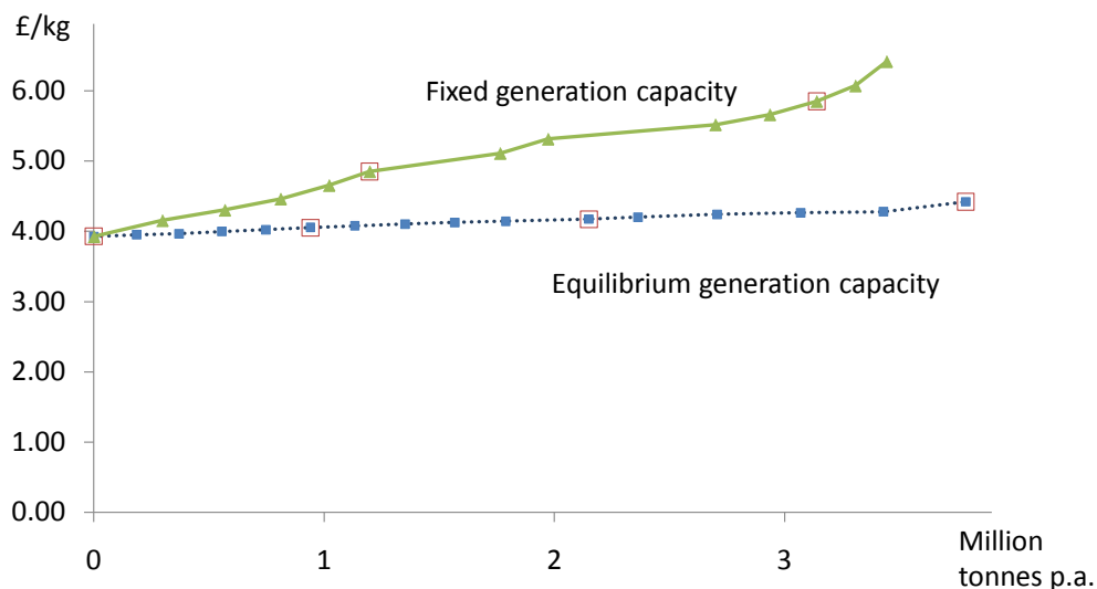
Figure 5: Hydrogen supply curves
