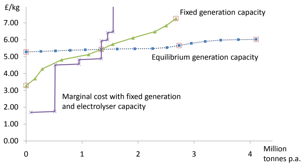
Figure 6: Supply curves for hydrogen: higher electrolyser costs
