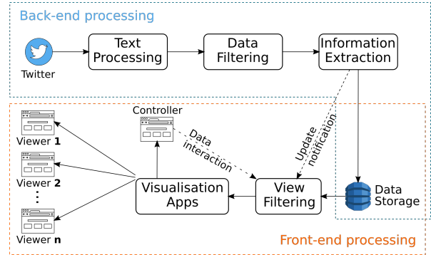
Figure 1: The system architecture of the Twitter Observatory
