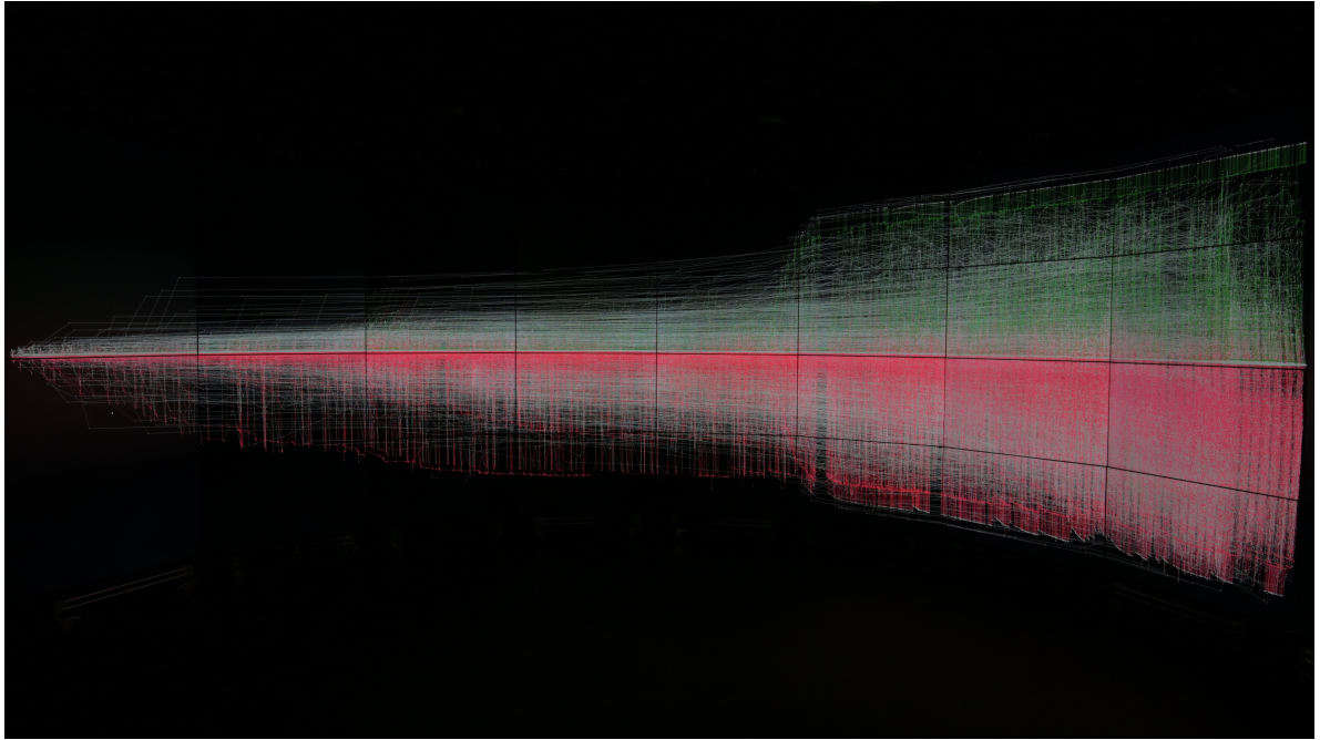
Figure 2: Photograph of the result of displaying a timeline with polarisation of tweets for the Brexit referendum dataset rendered in a 15360x4320 resolution
