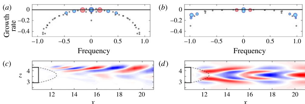
FIGURE 10. DMD results for (a,c) the unforced flow and (b,d) the flow with feedback control. (a,b) Shows the frequencies and growth rates of the DMD modes scaled by their optimum amplitudes; (c,d) is a top view of the spatial structure of the most dynamically represented modes (red markers on the frequency versus growth rate figure) at (a,c) St_h = 0.16 for unforced flow and (b,d) St_h = 0.13 for the flow with feedback control.
