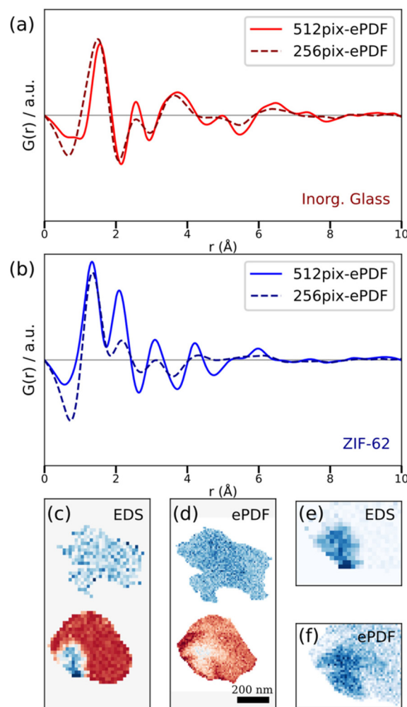
Fig. 5 STEM-ePDF analysis of a second example of the a_9\text{ZIF-62} and 0.67[(\text{Na}_2\text{O})_{0.9}(\text{P}_2\text{O}_5)] - 0.33[(\text{AlO}_{3/2})[\text{AlF}_{31.5}]] inorganic glass composite material. (a) and (b) Comparisons of area-averaged reduced ePDF profiles obtained using a 512 \times 512 pixel detector, for particles shown in Fig. 2–4 and using a 256 \times 256 pixel detector, for particles shown in (c)–(d), for (a) the inorganic glass and (b) a_9\text{ZIF-62} . (c) EDS map of Al (red) and Zn (blue) from the dataset, taken after the STEM-ePDF data. An NMF-PCA algorithm was applied for denoising the EDS spectra. 85 (d) The ICA maps corresponding to reduced ePDF components for the inorganic glass (red) and a_9\text{ZIF-62} (blue). (e) and (f) contrast-adjusted images of the small inclusion of a_9\text{ZIF-62} on the lower particle for (e) EDS and (f) ePDF analyses.
