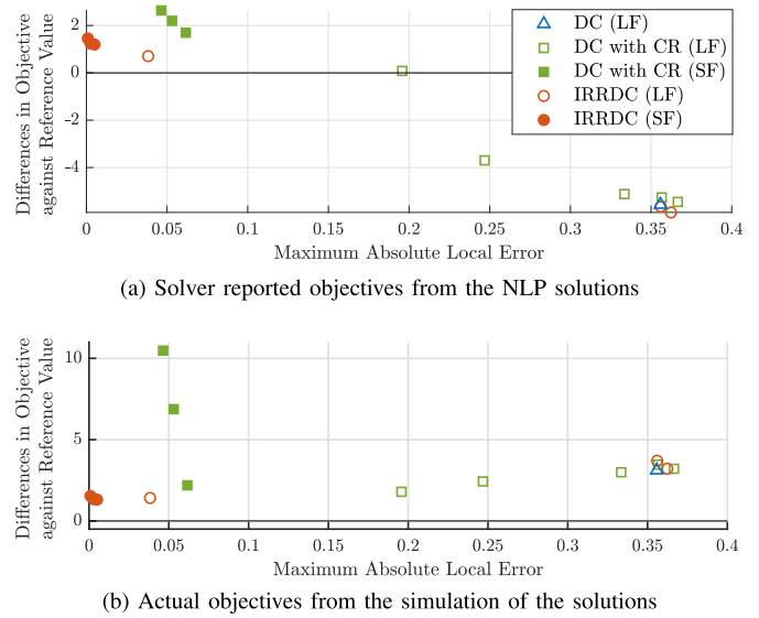
Fig. 2. IRRDC compared to DC with CR for the suppression of singular arc fluctuations when using different regularization weights. Reference objective is -18550.9 from [2, Ex. 4.9]. Solutions are also labeled as large fluctuations (LF) or suppressed fluctuations (SF) depending on whether large fluctuations can be visually observed inside the singular arc.
