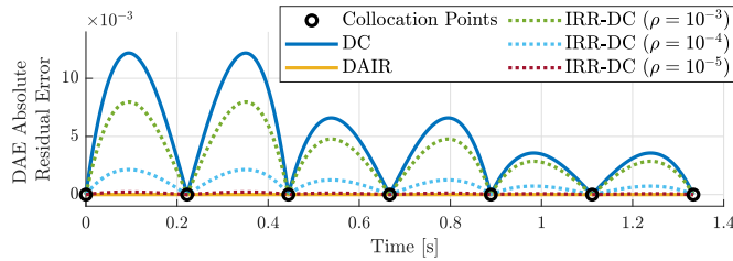
Fig. 3. Comparison of residual error for the algebraic constraint in the ventilator control problem.
