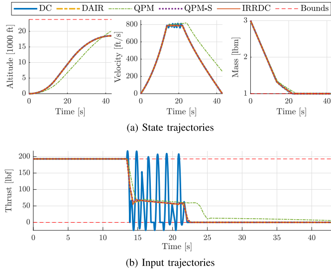
Fig. 1. Numerical solution to the Goddard rocket problem.
