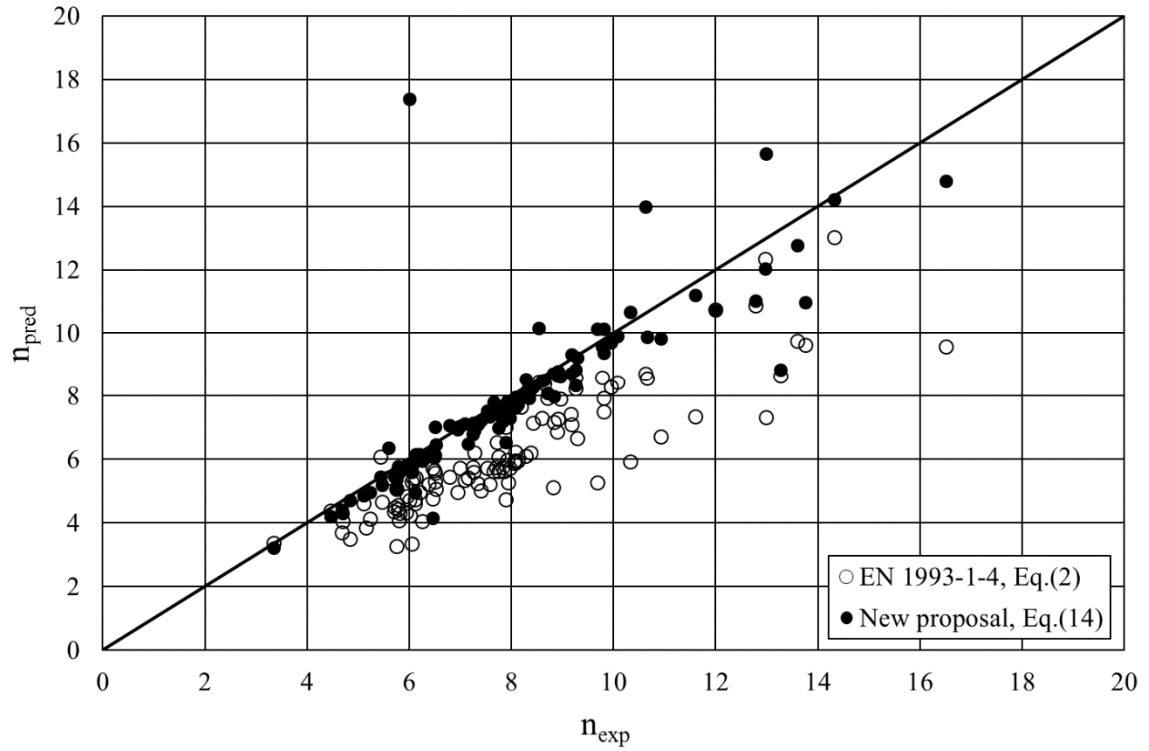
Figure 11. Prediction of strain hardening parameter n for duplex and lean duplex stainless steels.
