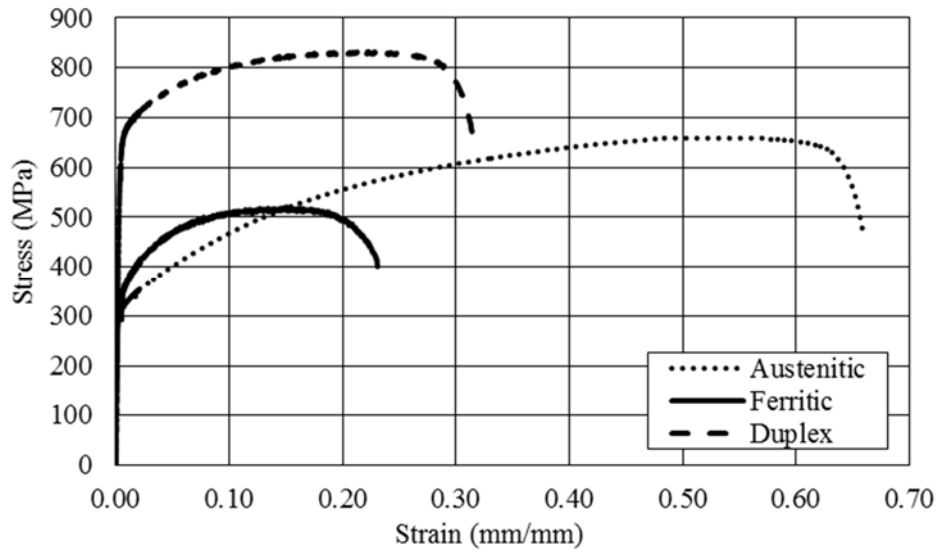
Figure 4. Measured stress-strain curves for each of the studied stainless steel grades.
