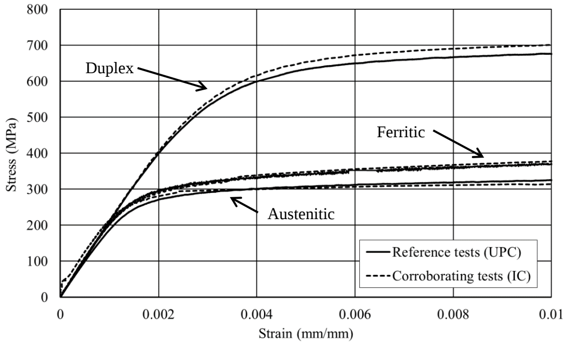
Figure 6. Comparison of measured stress-strain curves up to 1% strain for the three stainless steel families.
