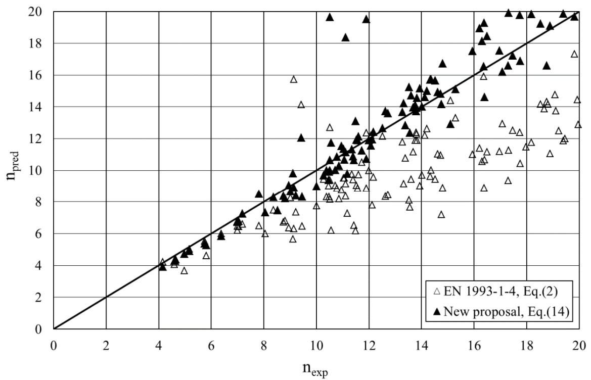
Figure 10. Prediction of strain hardening parameter n for ferritic stainless steels.
