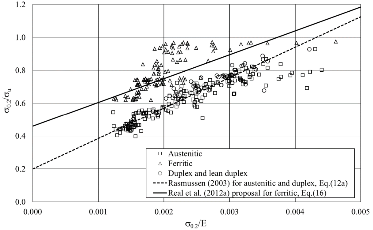
Figure 13. Assessment of ultimate strength \sigma_u for different stainless steel families.
