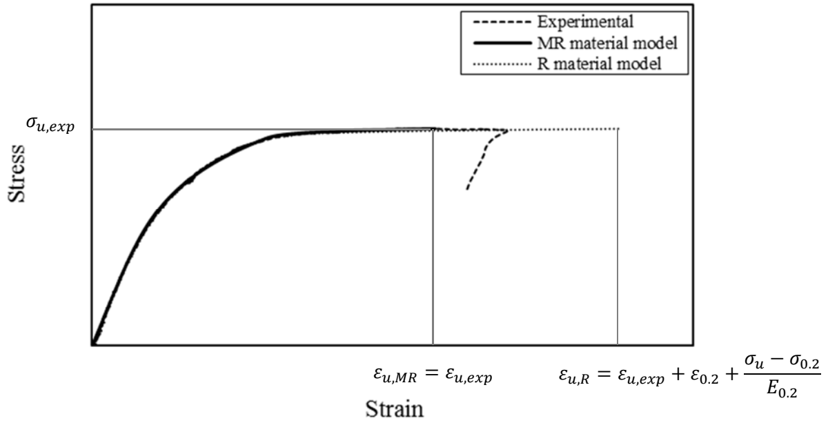
Figure 8. Comparison of Mirambell-Real (MR) and Rasmussen (R) material models with an experimental ferritic stainless steel stress-strain curve.
