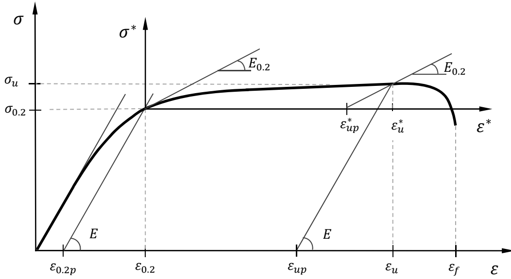
Figure 1. Typical stress-strain curve with definitions of key material parameters.
