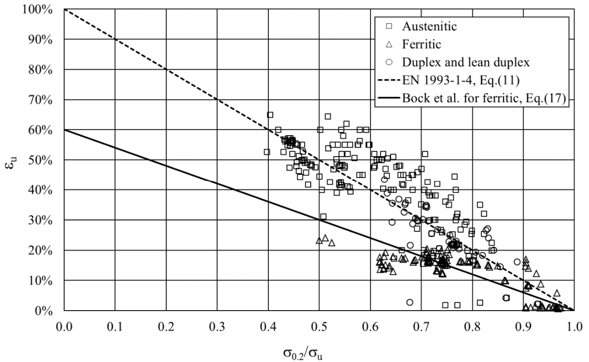
Figure 14. Assessment of ultimate strain \varepsilon_u for different stainless steel families.
