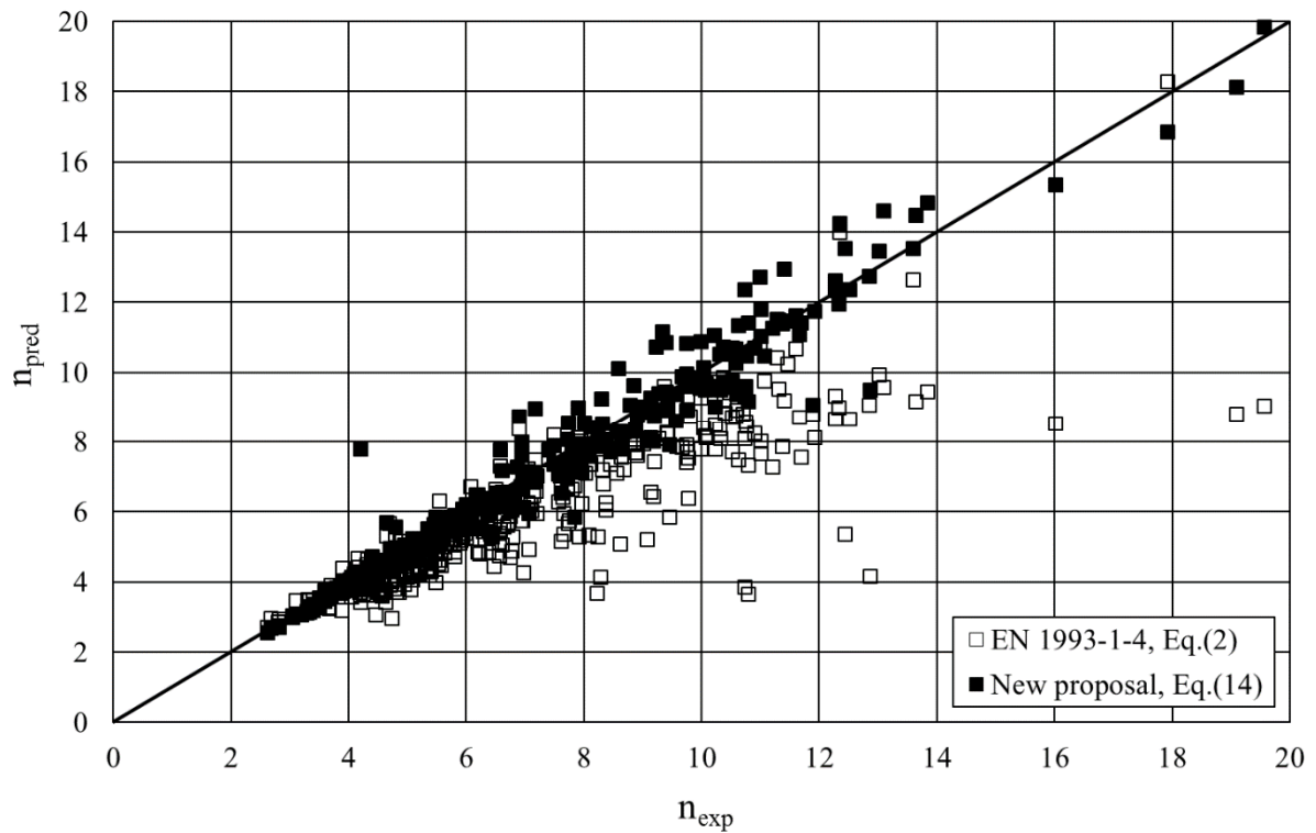
Figure 9. Prediction of strain hardening parameter n for austenitic stainless steels.
