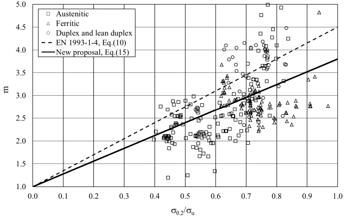
Figure 12. Assessment of strain hardening parameter m for different stainless steel families.
