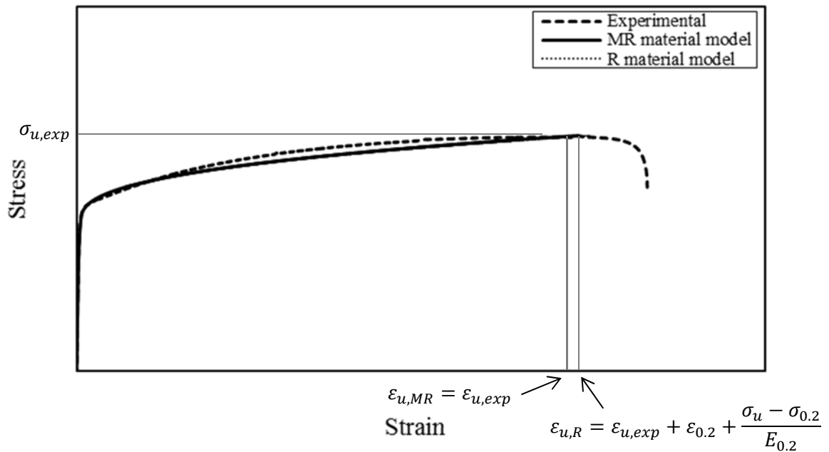
Figure 7. Comparison of Mirambell-Real (MR) and Rasmussen (R) material models with an experimental austenitic stainless steel stress-strain curve.
