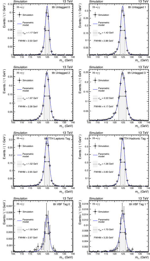
Figure A.3: The signal models for the t\bar{t}H process, evaluated at m_H = 125 GeV, obtained after application of the SSF interpolation method for the DCB+1G parametrisation of the simulated mass points. The \sigma_{\text{eff}} (half the width of the narrowest interval containing 68.3% of the invariant mass distribution) and the FWHM (the width of the distribution at half of the maximum value) are also shown. Note that the fits here maybe differ slightly from those in shown Figure 6.1, which were produced by fitting the m_H = 125 GeV samples only.
