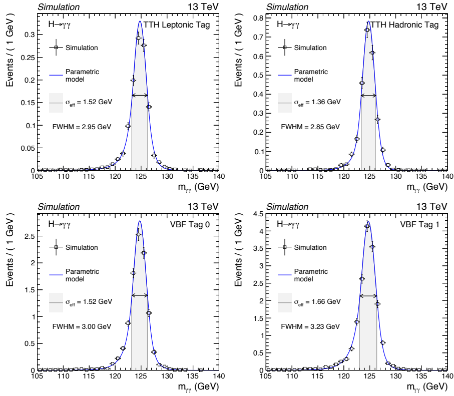
Figure 6.9: The signal models for the VBF-tagged and ttH-tagged analysis categories for m_H = 125 \text{ GeV} , obtained by summing the contributions from each production process according to their \epsilon \times A . The \sigma_{\text{eff}} (half the width of the narrowest interval containing 68.3% of the invariant mass distribution) and the FWHM (the width of the distribution at half of the maximum value) are also shown.
