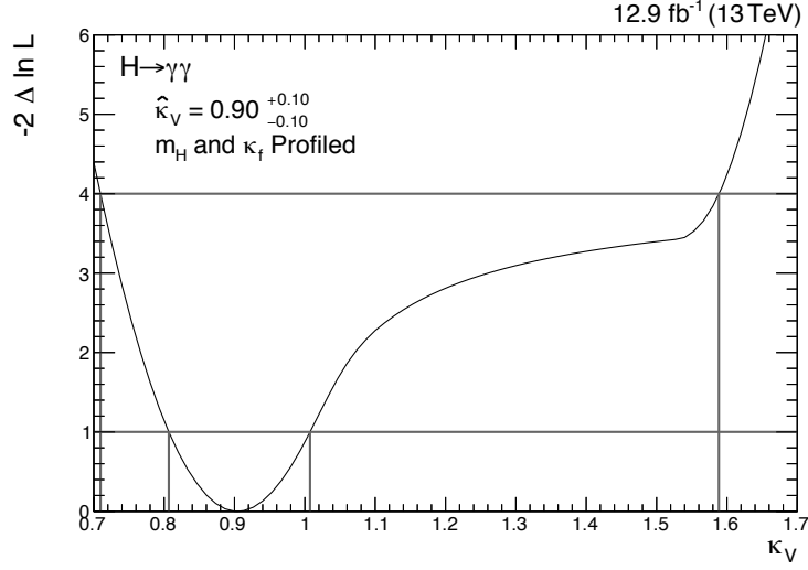
(a) 2 \Delta NLL scan of \kappa_V , profiling \kappa_f and m_H
