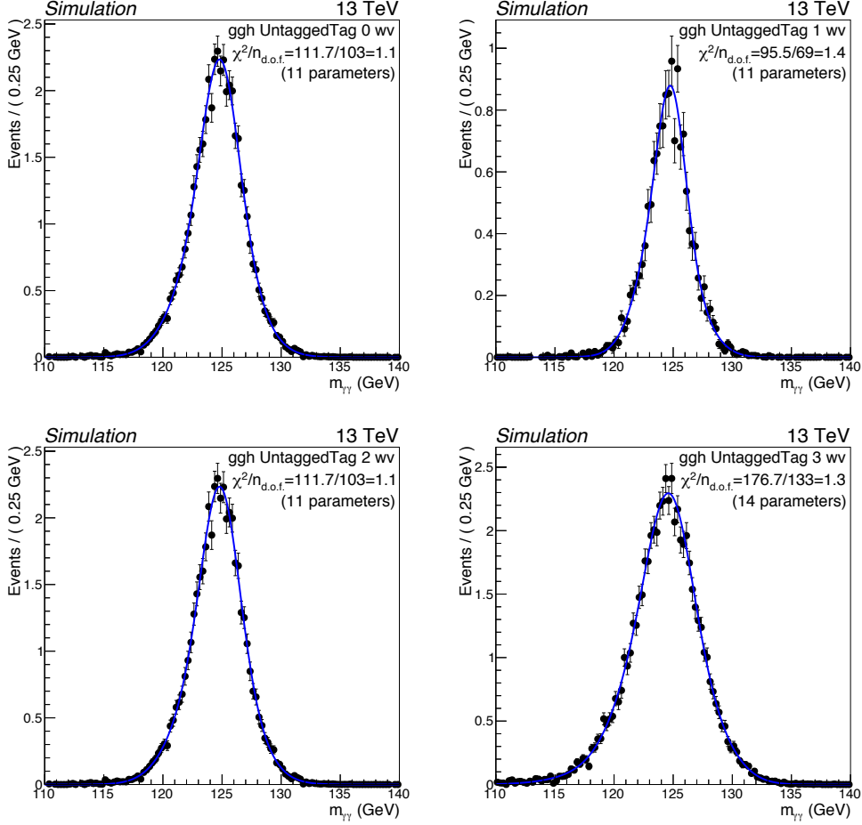
(a) WV fits with functional form: Sum of Gaussians
