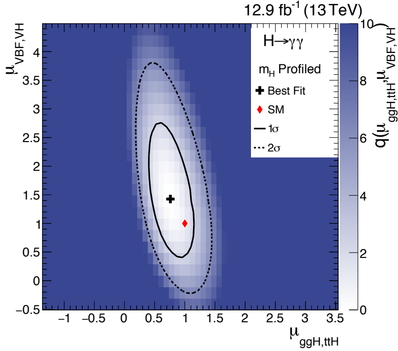
Figure 7.7: The result of a two-dimensional 2\Delta\text{NLL} scan of the \mu_{\text{ggH,ttH}} and \mu_{\text{VBF,VH}} components of the signal strength. The red diamond indicates the SM expectation, while the black cross shows the location of the best-fit point. The measurement is consistent with the SM within the uncertainty contours, which are shown in solid and dashed lines for the 1\sigma and 2\sigma uncertainties respectively. The value of m_H was profiled in the scan. The x -axis and y -axis are set to the same scale to show the difference in the sensitivity for \mu_{\text{ggH,ttH}} and \mu_{\text{VBF,VH}} .
