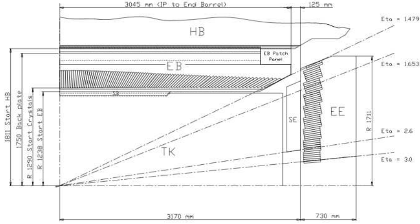
Figure 3.5: Schematic cross-section of one quadrant of the ECAL, showing the arrangement of crystals in the ECAL barrel and endcaps. The shower detector (SE, referred to as ES in the text) is also visible, as is the hadron calorimeter barrel (HB) and the tracker (TK) [53].
