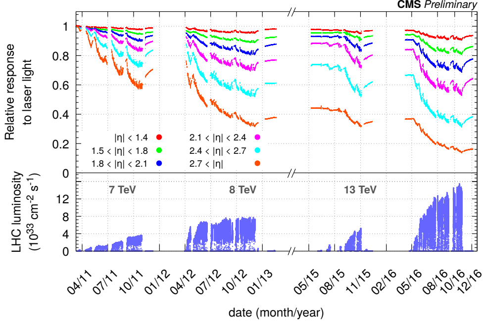
Figure 3.7: The response of the CMS ECAL lead tungstate crystals is shown as a function of time, and for different pseudorapidity ranges. The crystal response decreases as data are collected, due to transparency loss caused by exposure to radiation, and recovers during spontaneous annealing at times when no beams are presented [56].
