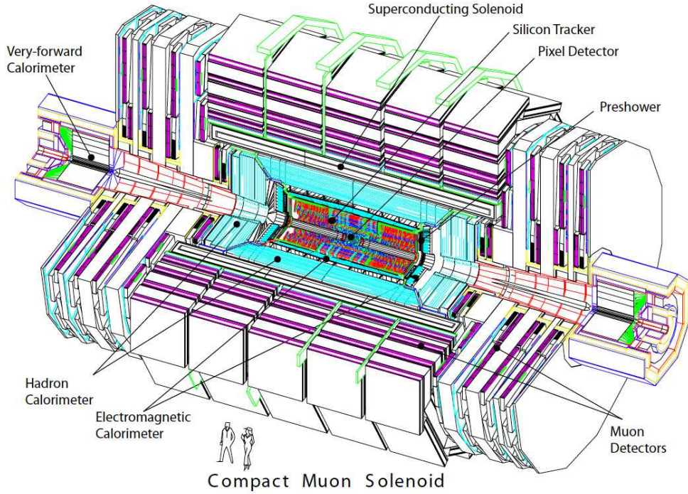
Figure 3.3: A cutaway diagram of the CMS detector, showing the main components and subdetectors, which are described in Section 3.2 [50].
