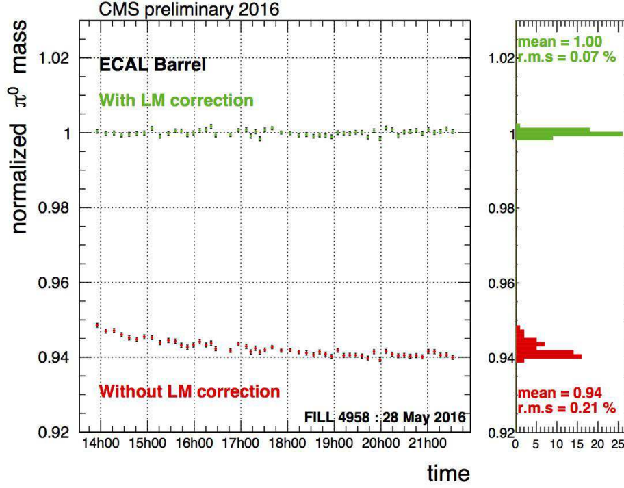
Figure 3.8: The normalised value of the invariant mass of the \pi^0 particle in its decay to photons, as measured by the CMS ECAL barrel, with and without the Laser Monitoring (LM) corrections for crystal transparency loss. This example, from a period of less than one day, shows the degradation of the response of the lead tungstate crystals, even over a period of hours [56].
