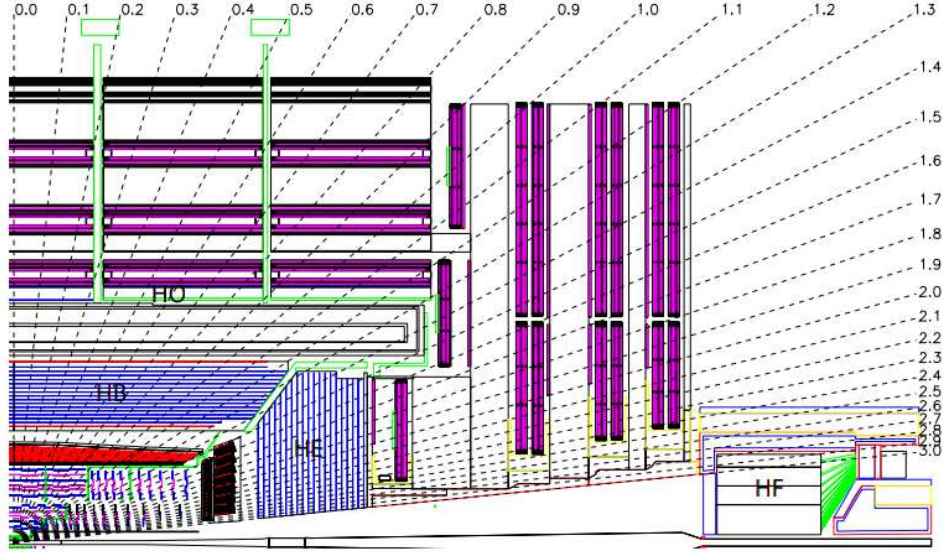
Figure 3.9: Schematic cross-section of one quadrant of the HCAL, showing the arrangement of the various components of the subdetector: The HB and HE surrounding the ECAL, with the HF at high \eta and the HO just outside of the solenoid [47].
