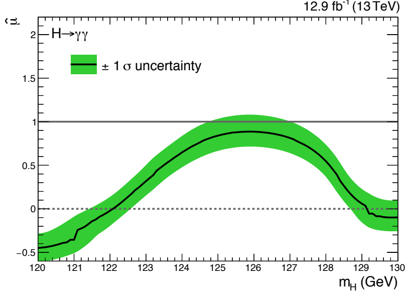
Figure 7.6: The best-fit signal strength for fixed values of m_H in the 120-130 GeV range, where the m_H parameter is fixed in the fitting procedure. The green bands show the \pm 1\sigma uncertainty obtained by finding the crossing with 2\Delta\text{NLL} = 1 . The discontinuities at m_H = 121.1 GeV and m_H = 129.2 GeV occur because at these points, the best-fit function in the discrete profiling method changes, leading to a slight jump in the measured signal strength.
