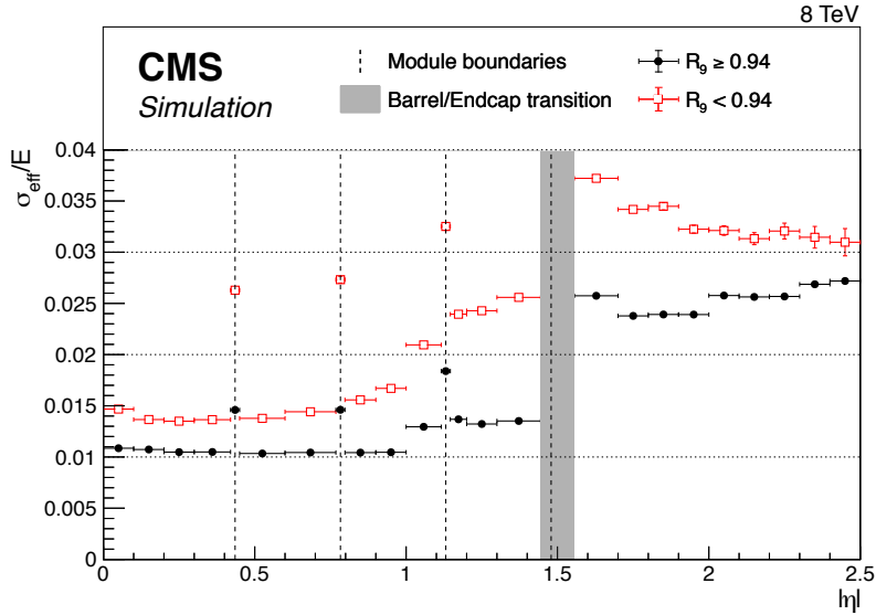
Figure 3.6: The relative energy resolution of individual simulated \text{H} \rightarrow \gamma\gamma photons in Run 1 as a function of |\eta| , shown separately for unconverted photons (black circles, R_9 \geq 0.94 ) and converted photons (open red squares, R_9 < 0.94 ). The vertical lines represent the boundaries between the ECAL modules in the barrel, while the grey band indicates the transition region between the EB and the EE, where photons are not reconstructed [54]. The R_9 variable is defined in Section 4.3.2.
