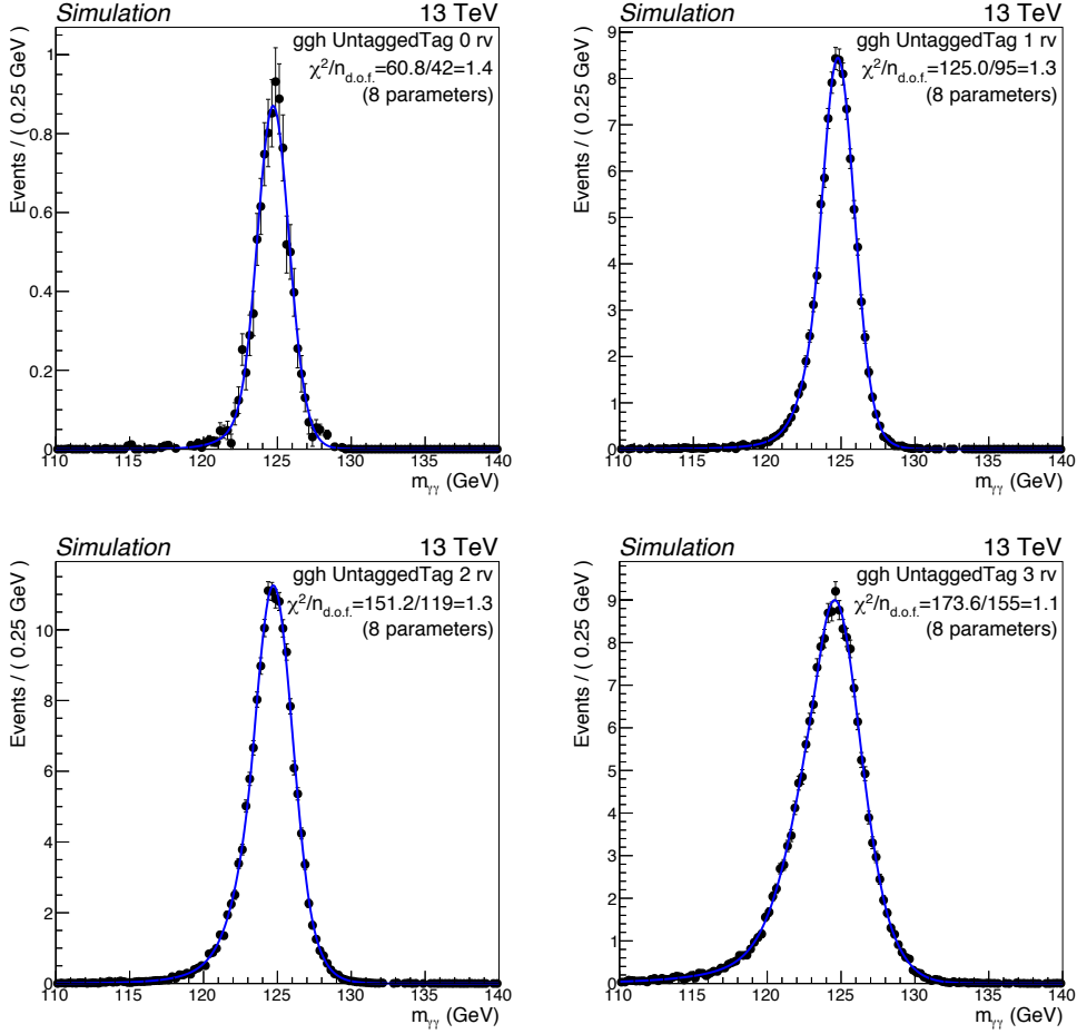
(a) RV fits with functional form: DCB+1G
