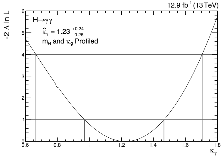
(b) 2 \Delta NLL scan of \kappa_\gamma , profiling \kappa_g and m_H
