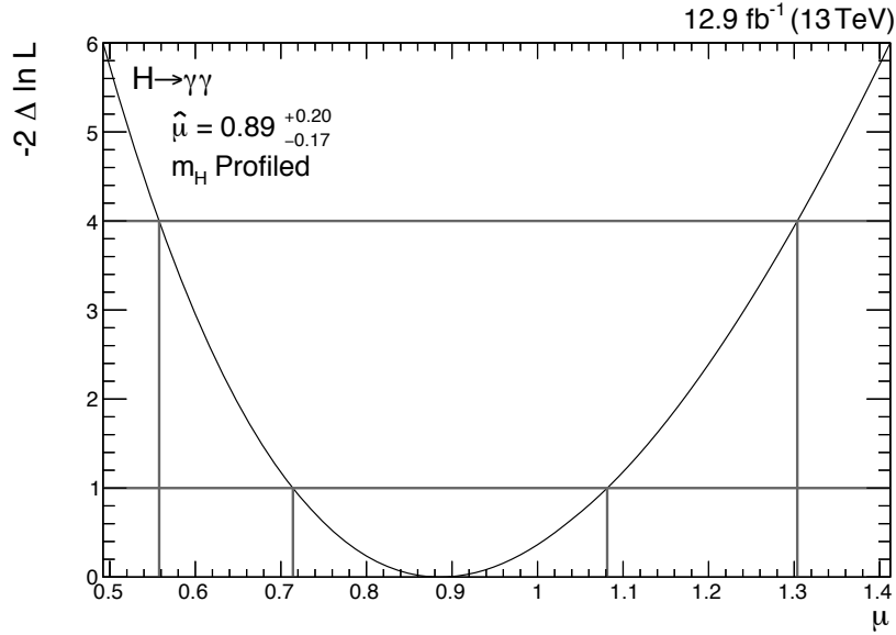
Figure 7.5: The 2\Delta\text{NLL} scan of the overall signal strength for a Higgs boson decaying to two photons. The mass of the Higgs boson is profiled in the fit. The 1\sigma and 2\sigma uncertainties correspond to the crossings with 2\Delta\text{NLL} = 1 and 2\Delta\text{NLL} = 4 .
