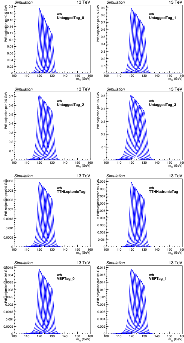
Figure A.9: The m_H -dependence of the signal models for the WH process for each of the categories is shown. Each curve shows the signal model for a given value of m_H . The contributions from the RV and WV components of each model were interpolated between the samples for different m_H using the SSF method, and summed together according to their relative event content.
