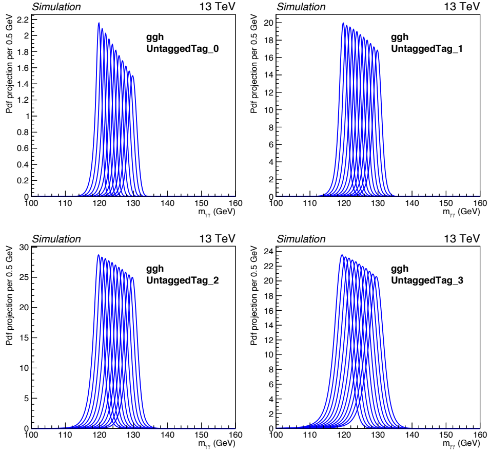
Figure 6.6: The m_H -dependence of the signal models for the ggH process for each of the Untagged categories is shown. Each curve shows the signal model for a given value of m_H . The contributions from the RV and WV components of each model were interpolated between the samples for different m_H using the SSF method, and summed together according to their relative event content.
