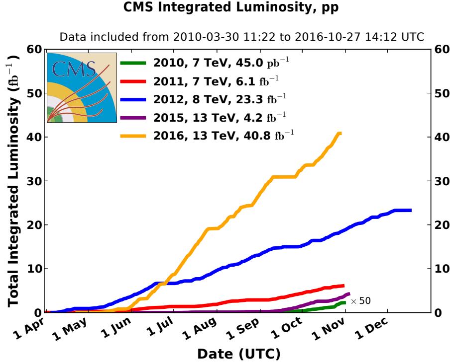
Figure 3.2: Overview of the integrated luminosity delivered by the LHC throughout its operation until the time of writing, as recorded by CMS [45].
