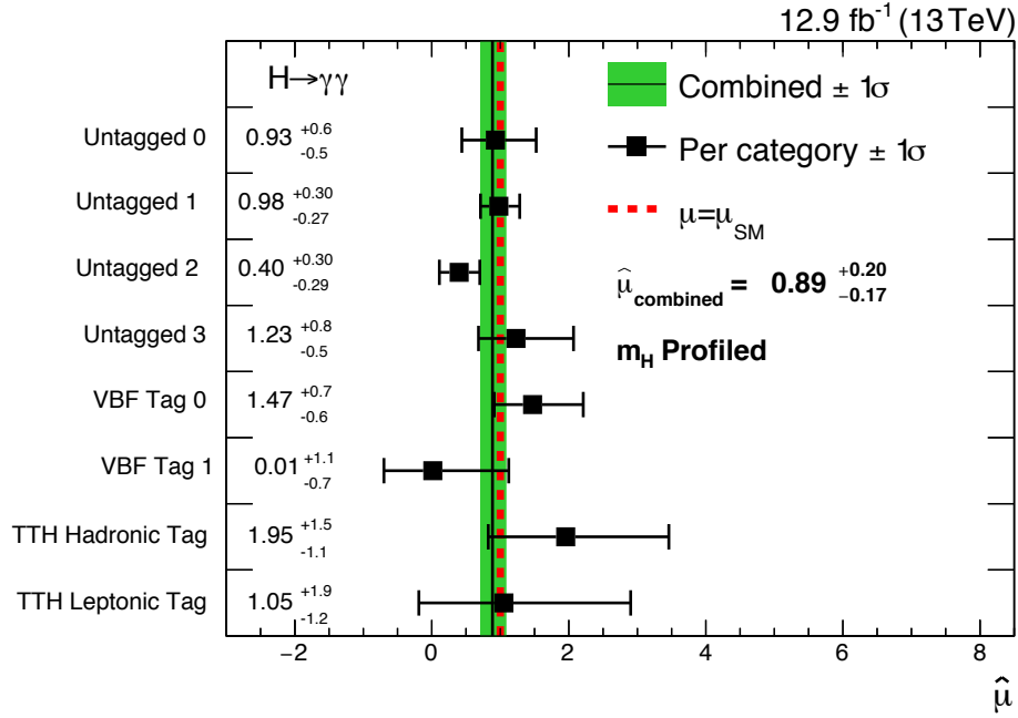
Figure 7.9: The measurements of the per-category signal strengths, obtained by performing 2\Delta\text{NLL} scans of each one while profiling the others. In each case m_H is also profiled in the fit. The vertical black line and green bands represent the measurement of the overall signal strength \mu , and the SM expectation is shown in the vertical red dashed line. The per-category signal strengths do not have a direct physical interpretation, and this result is a check that no particular category is introducing a large bias into the overall measurement.
