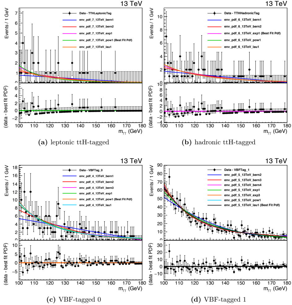
Figure A.11: The set of candidate functions chosen to parametrise the background using the discrete profiling method in the VBF and ttH categories. For each category, all candidate functions give acceptable agreement with the data, but can lead to large variations in the predicted number of events in the region of interest between 120 and 130 GeV. The resulting uncertainty in the choice of parametrisation is handled by the discrete profiling method.
