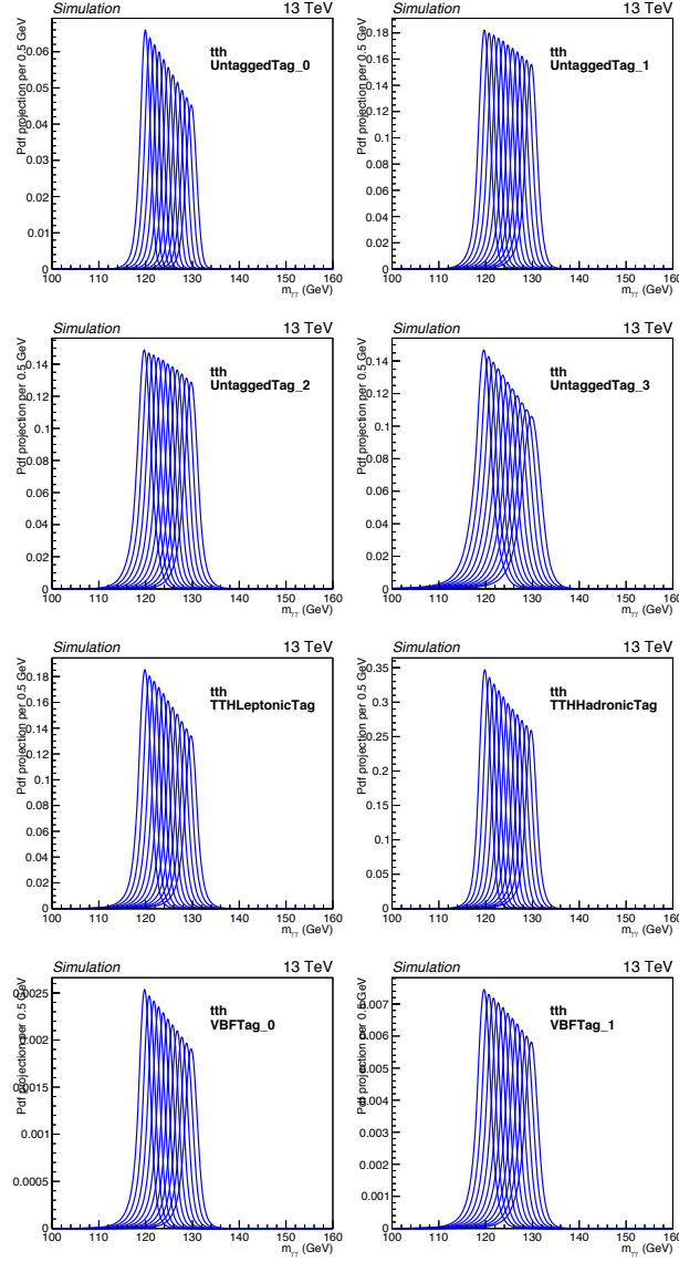
Figure A.8: The m_H -dependence of the signal models for the t\bar{t}H process for each of the categories is shown. Each curve shows the signal model for a given value of m_H . The contributions from the RV and WV components of each model were interpolated between the samples for different m_H using the SSF method, and summed together according to their relative event content.
