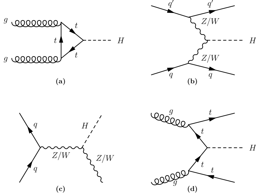
Figure 2.1: Higgs production modes at the LHC: (a) gluon-gluon fusion, via a loop of top quarks, (b) vector boson fusion, with associated quark production, (c) associated vector boson production with either the Z or W boson and (d) top quark fusion with associated top quark production.
