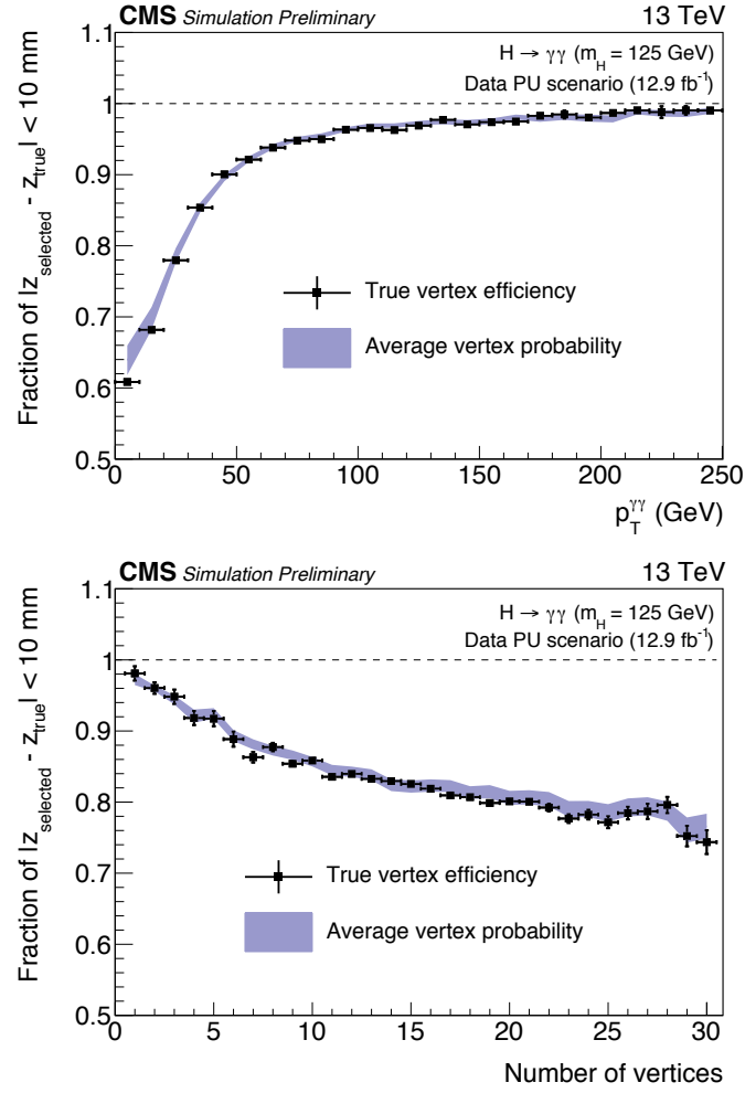
Figure 4.3: The efficiency to select a vertex within 1 cm of the true vertex in simulated H \rightarrow \gamma\gamma events as a function p_T and the number of vertices in the event. The estimated probability that the vertex is chosen within 1 cm is superimposed. The uncertainty on the vertex-finding probability is determined using Z \rightarrow \mu^-\mu^+ events. The simulation is reweighted such that the distribution of the number of vertices and the width of the interaction region matched in data and simulation [2].
