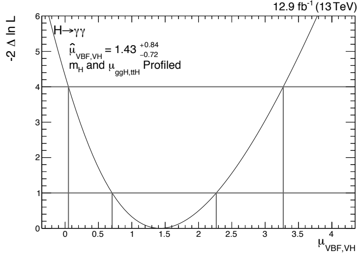
(a) 2 \Delta NLL scan of \mu_{\text{VBF,VH}} , profiling \mu_{\text{ggH,ttH}} and m_H
