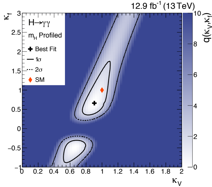
(a) 2ΔNLL scan of \kappa_f versus \kappa_V
