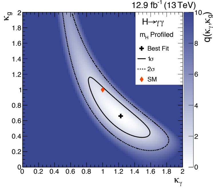
(a) 2ΔNLL scan of \kappa_\gamma versus \kappa_g
