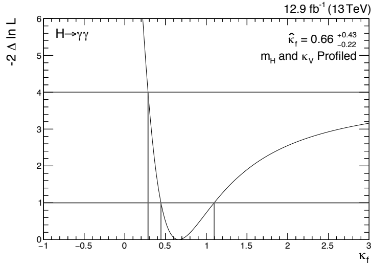
(b) 2 \Delta NLL scan of \kappa_f , profiling \kappa_V and m_H
