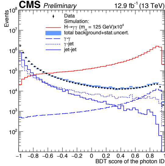
Figure 4.1: The BDT_{\gamma ID} output score for the lower-scoring photon in each diphoton pair in the range 100 < m_{\gamma\gamma} < 180 GeV for data and simulation. The simulation is composed of signal ( H \rightarrow \gamma\gamma photons with m_H = 125 GeV) and background, which has been split into \gamma\gamma , \gamma -jet and jet-jet components. The sum of the background components has been scaled to the number of events in data [2].
