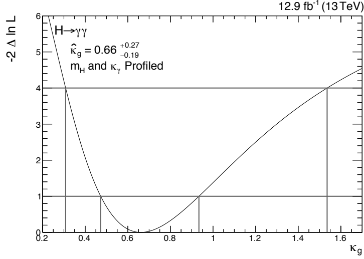
(a) 2 \Delta NLL scan of \kappa_g , profiling \kappa_\gamma and m_H
