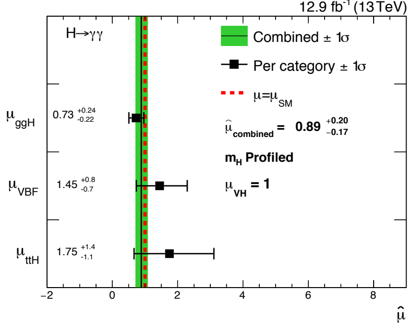
Figure 7.8: The measurements of the per-process signal strengths \mu_{ggH} , \mu_{VBF} , \mu_{ttH} , obtained by performing 2\Delta NLL scans of each one while profiling the others. In each case m_H is also profiled in the fit, and \mu_{VH} = 1 is imposed since this analysis does not include any categories specifically targeting the VH process. The vertical black line and green bands represent the measurement of the overall signal strength \mu , and the SM expectation is shown in the vertical red dashed line.
