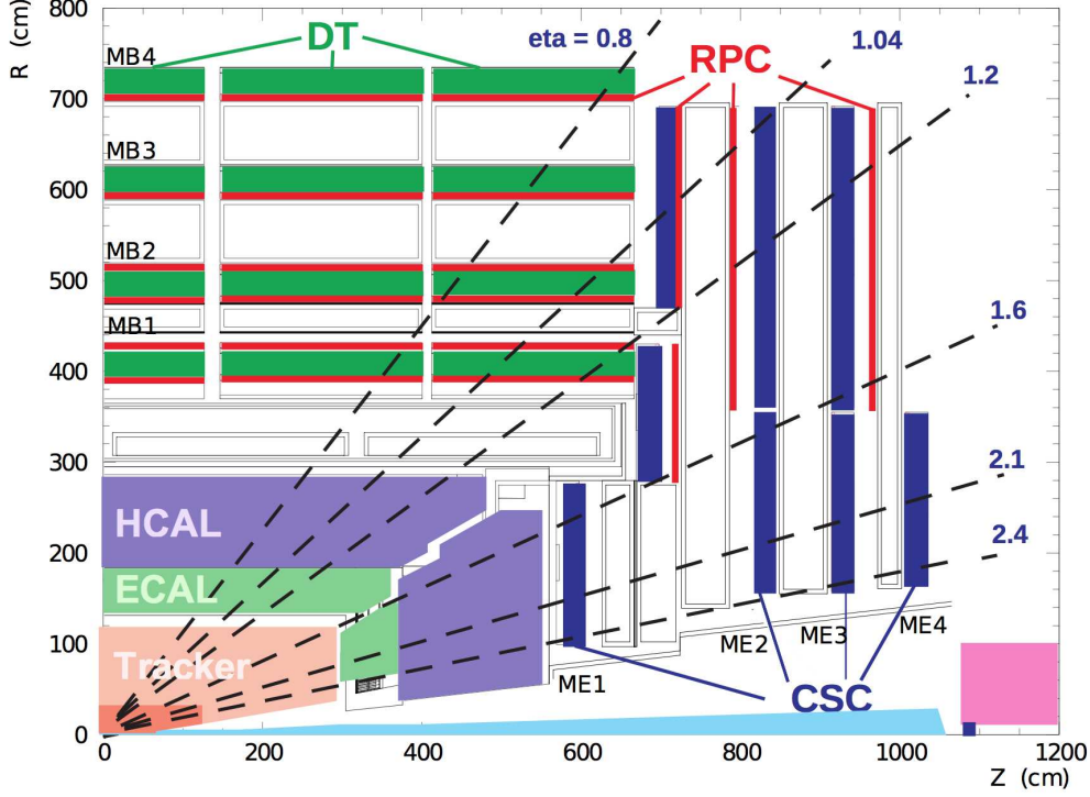
Figure 3.10: Schematic cross-section of one quadrant of the CMS muon detector, showing the arrangement of the various components of the sub-detector: The DTs in the barrel, and CSCs in the endcaps and the RPCs in both [59].
