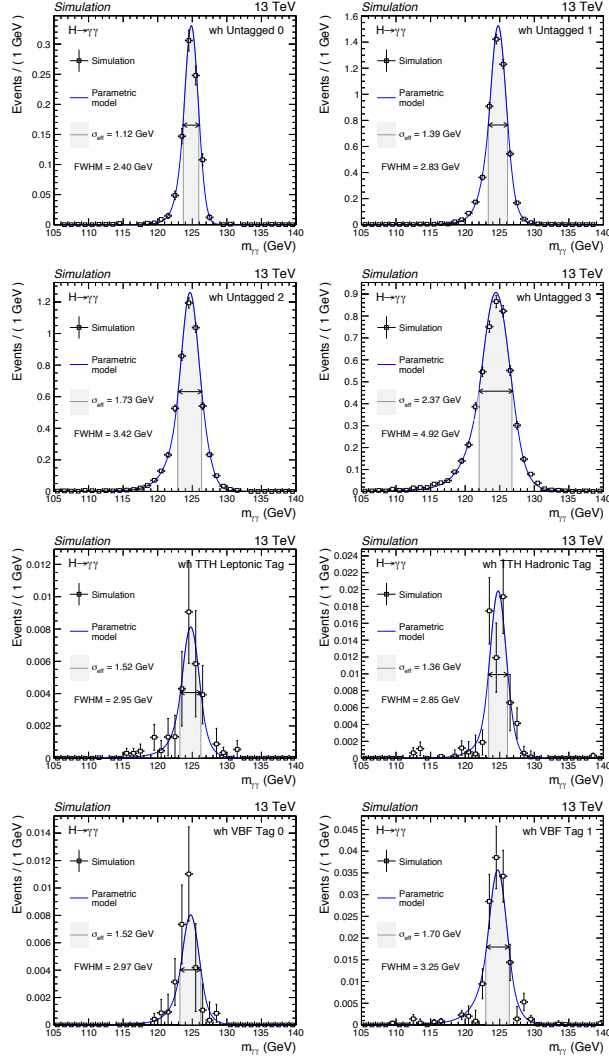
Figure A.4: The signal models for the WH process, which is later combined with ZH to model the VH process, evaluated at m_H = 125 GeV, obtained after application of the SSF interpolation method for the DCB+1G parametrisation of the simulated mass points. The \sigma_{\text{eff}} (half the width of the narrowest interval containing 68.3% of the invariant mass distribution) and the FWHM (the width of the distribution at half of the maximum value) are also shown. Note that the fits here maybe differ slightly from those in shown Figure 6.1, which were produced by fitting the m_H = 125 GeV samples only.
