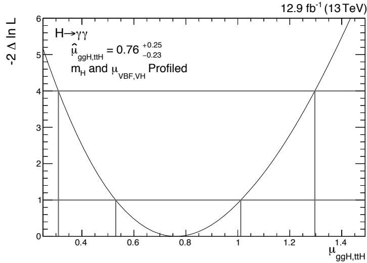
(b) 2 \Delta NLL scan of \mu_{\text{ggH,ttH}} , profiling \mu_{\text{VBF,VH}} and m_H
