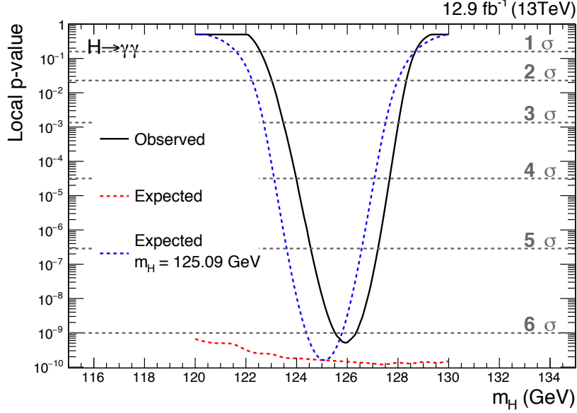
Figure 7.4: The local p -value for the observation as a function of the Higgs boson mass (black), shown with the expected local p -values for a SM Higgs boson, across the range 120-130 GeV. The expected local p -values are obtained using Asimov datasets. The blue dashed line shows the expected local p -value when the mass of the injected signal is m_H = 125.09 GeV, while the red line shows the maximum significance for any injected signal in the range of 120 to 130 GeV.
