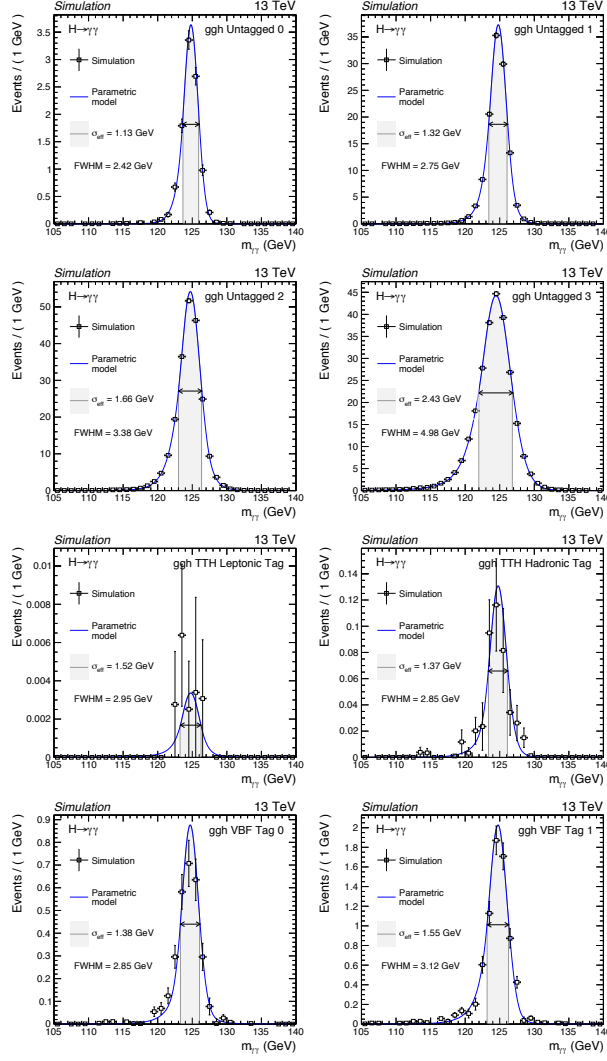
Figure A.1: The signal models for the ggH process, evaluated at m_H = 125 GeV, obtained after application of the SSF interpolation method for the DCB+1G parametrisation of the simulated mass points. The \sigma_{\text{eff}} (half the width of the narrowest interval containing 68.3% of the invariant mass distribution) and the FWHM (the width of the distribution at half of the maximum value) are also shown. Note that the fits here maybe differ slightly from those in shown Figure 6.1, which were produced by fitting the m_H = 125 GeV samples only.
