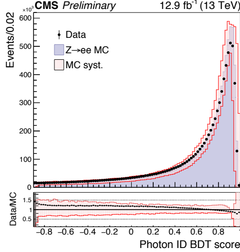
Figure 4.2: The BDT_{\gamma ID} output score for Z \rightarrow e^+e^- events in data and simulation (labelled MC), where the electrons are reconstructed as photons with the electron veto requirement inverted. The red shaded region corresponds to a systematic uncertainty of approximately 3% on the value of the output score which is introduced to cover discrepancies between data and simulation [2].
