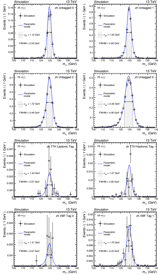
Figure A.5: The signal models for the ZH process, which is later combined with WH to model the VH process, evaluated at m_H = 125 GeV, obtained after application of the SSF interpolation method for the DCB+1G parametrisation of the simulated mass points. The \sigma_{\text{eff}} (half the width of the narrowest interval containing 68.3% of the invariant mass distribution) and the FWHM (the width of the distribution at half of the maximum value) are also shown. Note that the fits here maybe differ slightly from those in shown Figure 6.1, which were produced by fitting the m_H = 125 GeV samples only.
