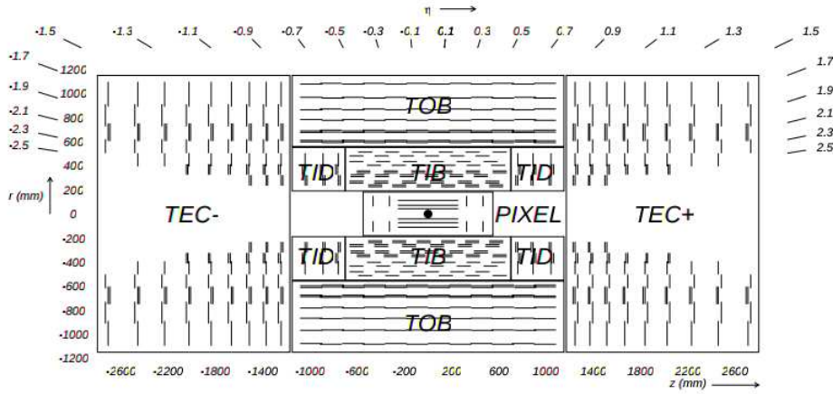
Figure 3.4: A diagram showing the layout of the CMS tracker components: the pixel tracker (labelled PIXEL) is the nearest to the interaction region marked by the black dot. The various sections of the strip tracker (TIB, TID, TOB, TEC+ and TEC-) are arranged around the pixel tracker [50].
