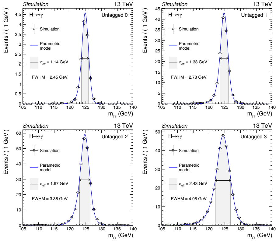
Figure 6.8: The signal models for the Untagged analysis categories for m_H = 125 GeV, obtained by summing the contributions from each production process according to their \epsilon \times A . The \sigma_{\text{eff}} (half the width of the narrowest interval containing 68.3% of the invariant mass distribution) and the FWHM (the width of the distribution at half of the maximum value) are also shown.
