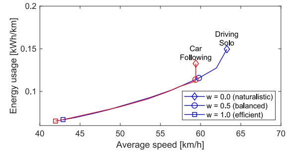
Fig. 9. Pareto comparison of cornering and cornering with following cases.
