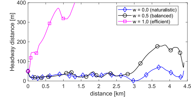
Fig. 10. Solution of the car-following case for three combinations of driving preferences and energy economy.
