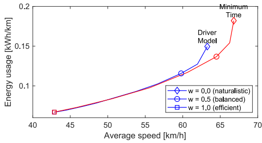
Fig. 7. Pareto comparison of driver model with minimum time optimisation.
