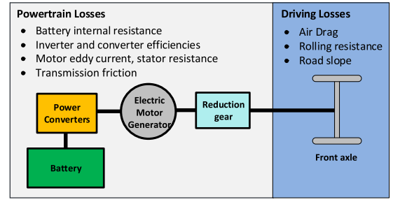
Fig. 1. Electric vehicle powertrain structure and losses considered.
