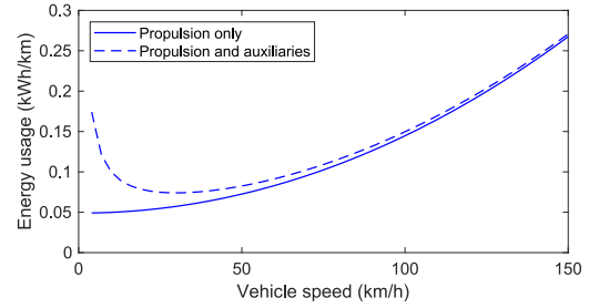
Fig. 3. Specific energy usage while driving at constant speed (the solid line neglects idle losses, the dotted line accounts for an idle power loss of 500 W).
