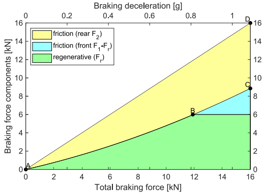
Fig. 4. Braking force distribution and regenerative braking. (the maximum regenerative torque, and the resulting position of B along curve AC, decreases for speeds greater than 16 m/s due to the power limits of the motor).
