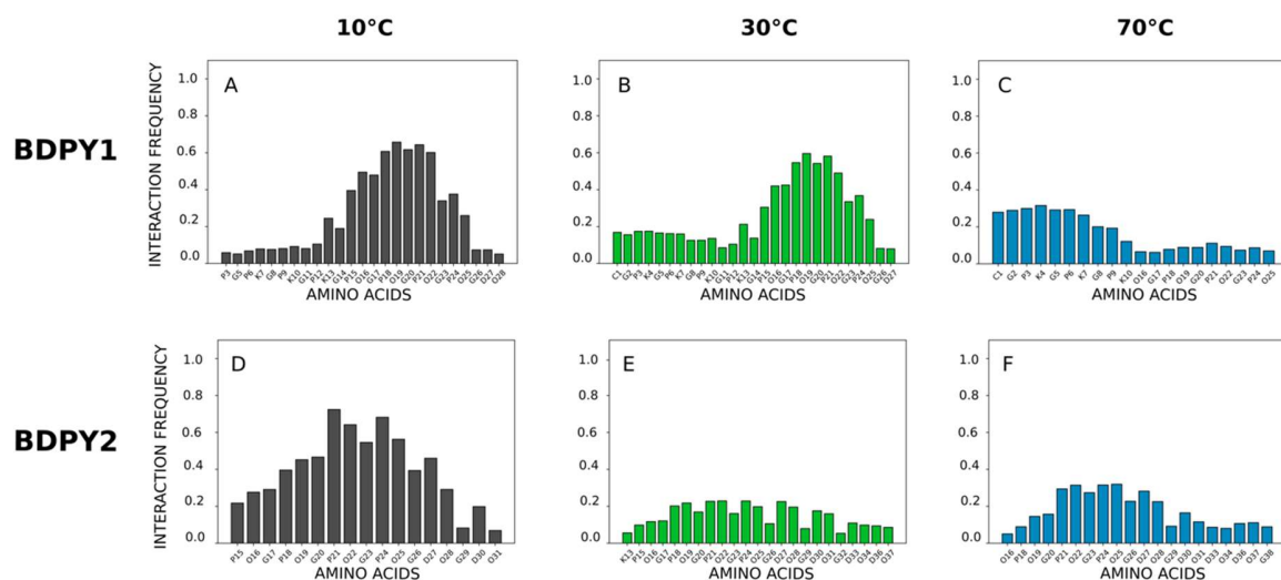
Figure S6. Atomistic contacts between CLP and BDPY1 and BDPY2. (A) Contact frequency between CLP and BDPY1 at 10°C, (B) 30°C and (C) 70°C. (D) Contact frequency between CLP and BDPY2 at 10°C, (E) 30°C and (F) 70°C.
