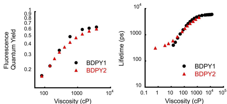
Figure S1. Left: Fluorescence quantum yields (QY) for BDPY1 and BDPY2 measured at different viscosities in glycerol solutions at different temperatures. Right: Fluorescence lifetime for BDPY1 and BDPY2 measured at different viscosities. It is clear to see that both QY and lifetime curves show excellent overlap, which could be expected from their very similar molecular structures, Scheme 1 of the main text. For BDPY2, we infer that the differences in fluorescence intensities seen upon interaction with CLP are, indeed, due to different interactions between these rotors with CPL, rather than differences in calibration vs viscosity. We hypothesise that additional charges on BDPY2 make it more hydrophilic and aid interactions with CPL.
