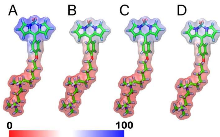
Figure S8. Contact density maps for the interaction of BDPY2 with the three-dimensional structure of CLP. Simulations run at 10°C (A), 30°C (B), 50 °C (C), and 70°C (D) degrees. Colouring represents contact density from 0% (red) to 100% (blue).
