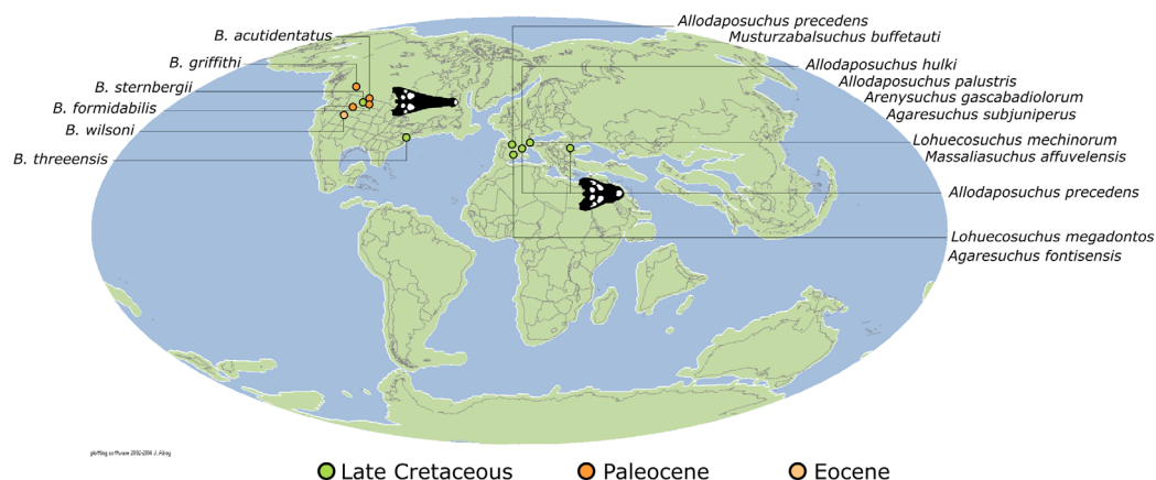
Figure 27 The distribution of named species referred to Allodaposuchidae and Borealosuchus. Global palaeogeographical reconstruction at 66 Ma from Fossilworks ( http://fossilworks.org/ ) (Alroy, 2013) based on data in the Paleobiology Database ( https://paleobiodb.org/ ). Full-size DOI: 10.7717/peerj.12094/fig-27
