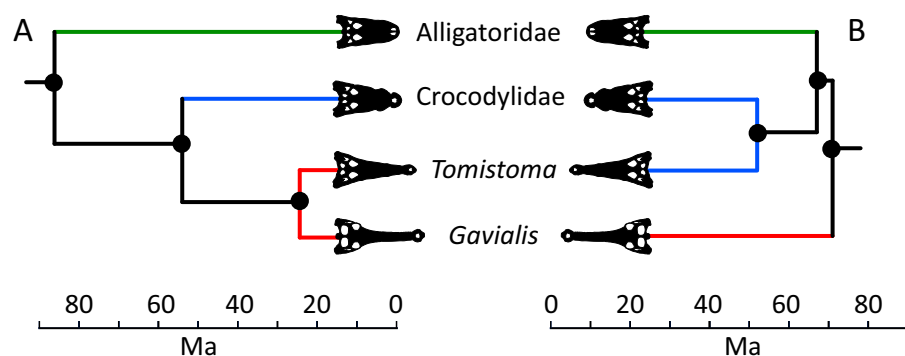
Figure 5 Contrasting topologies of molecular (A) and morphological (B) phylogenies illustrating differences in the divergence of principal crocodylian clades. Molecular divergences based on Oaks (2011) and morphological divergences based on the stratigraphically oldest fossils assigned to each clade prior to the current study. Full-size DOI: 10.7717/peerj.12094/fig-5
