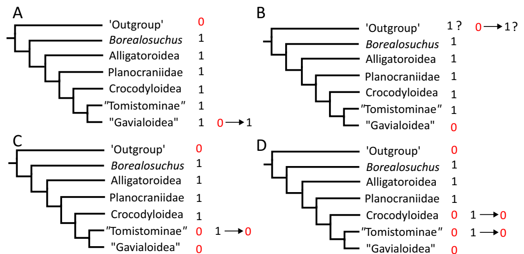
Figure 20 Simplified cladograms illustrating the principal changes in character optimisation of synapomorphies of Brevirostres and stemwards nodes recovered in Narváez et al. (2016). For simplicity, 'outgroup' refers to all taxa stemward of Borealosuchus recovered here. See text for further explanation. Full-size DOI: 10.7717/peerj.12094/fig-20
