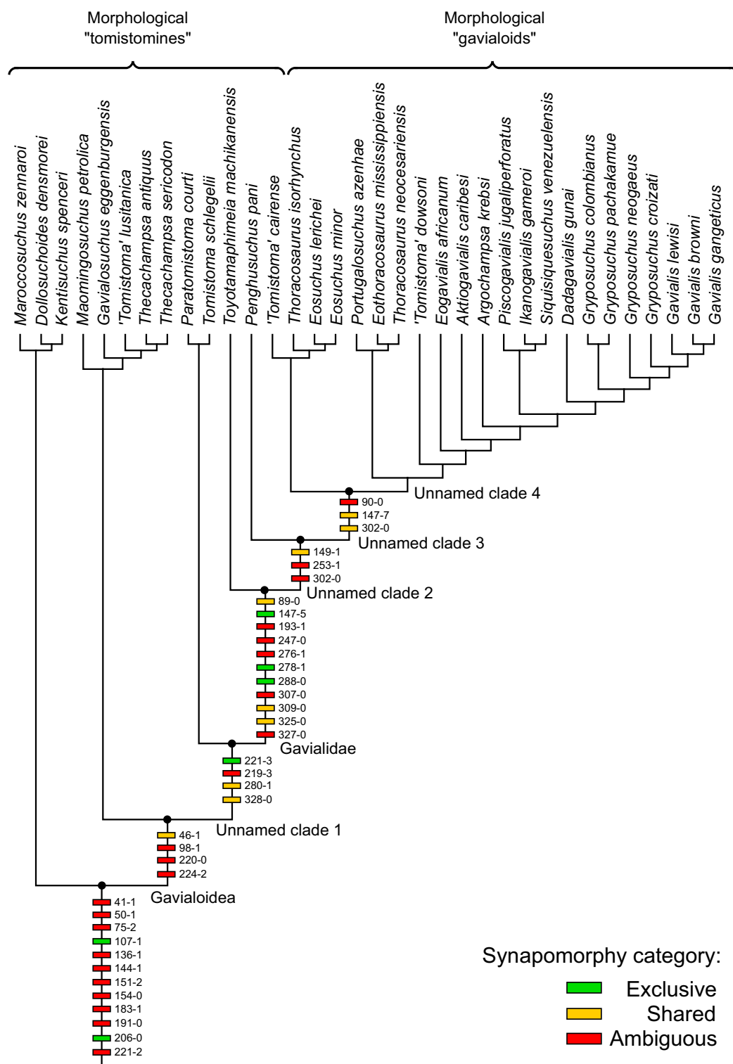
Figure 21 Synapomorphies of Gavialoidea and less inclusive clades that unite morphological (=traditional) tomistomines and gavialoids. Full-size DOI: 10.7717/peerj.12094/fig-21
