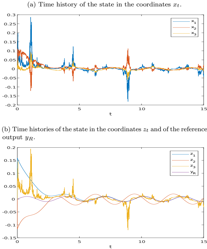
Fig. 2. Local asymptotic output tracking of system (8).
