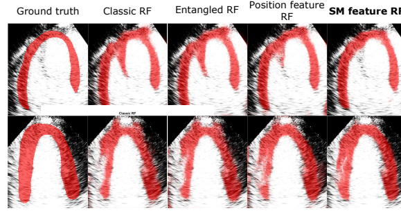
Fig. 3: Effect of bounding box detection on RF segmentation. Error bar denotes the standard deviation over Dataset1 Fig. 4: Visual comparison of the RF probability maps obtained by different RF variants.
