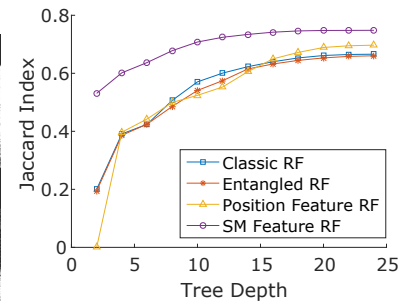
Fig. 5: Comparison of Jaccard indices of different RF variants vs tree depth.
