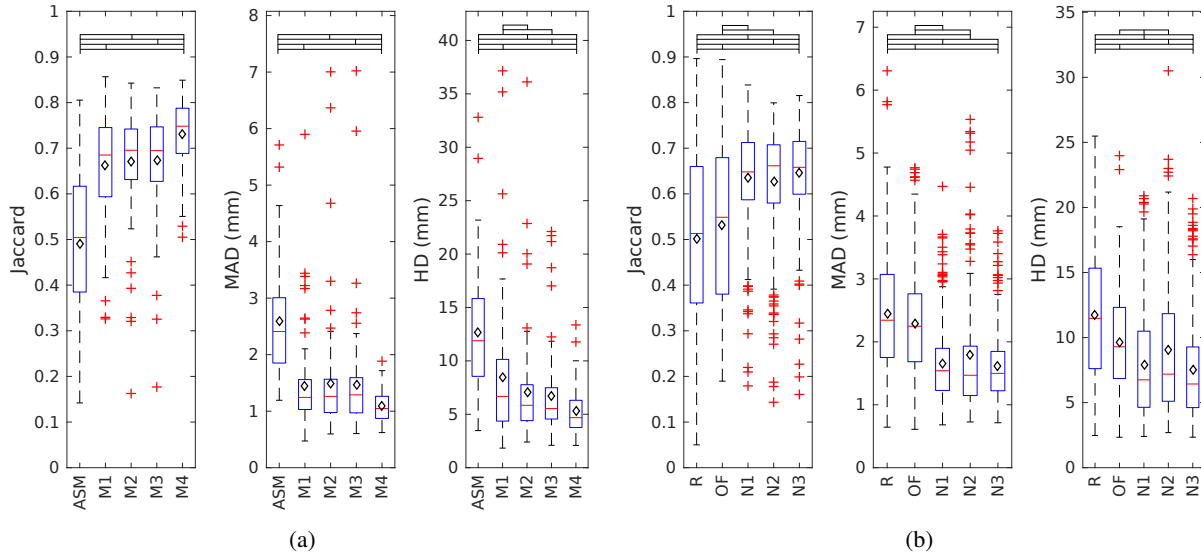
Fig. 6: Segmentation accuracy results of the various approaches for (a) Dataset1 and (b) Dataset2 . The red line and the black diamond marker represent the median and the mean respectively. The ends of the whiskers represent the lowest and highest data point within 1.5 times the interquartile range. Top black brackets indicate the difference between the two approaches is significant using the paired t-test.
