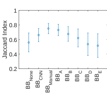
Fig. 3: Effect of bounding box detection on RF segmentation. Error bar denotes the standard deviation over Dataset1 Fig. 4: Visual comparison of the RF probability maps obtained by different RF variants.
