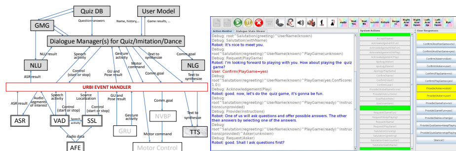
Fig. 2. Left: The components of the integrated system. Filled boxes: components implemented in Java, double-line boxes: C/C++, and plain boxes: UrbiScript. The TTS component is either the Acapela TTS on the Nao or the Mary TTS implemented in Java. Right: The Quiz Game Wizard GUI.
