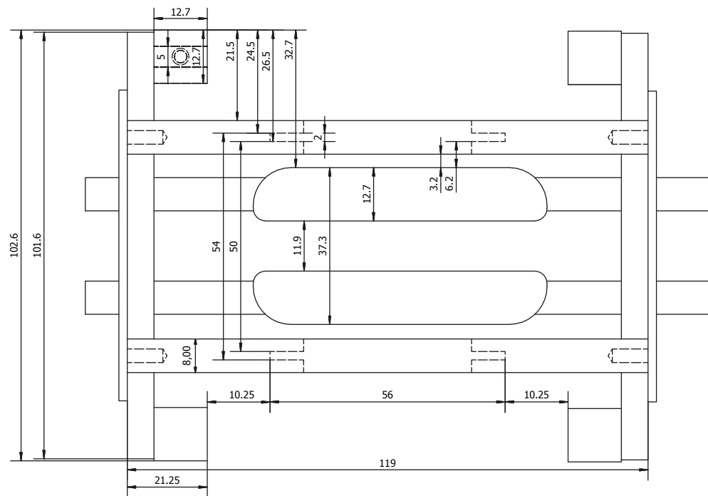
FIGURE C.2: Cross section in the xz -plane of the field plate assembly.
