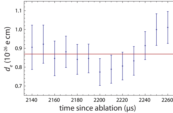
FIGURE 4.7: Variation in d_e across TOF profile observed when \bar{V} = 0.0 \text{ V} . The range of the horizontal axis is set to the interval of the analysis gate specified in section 4.1.
