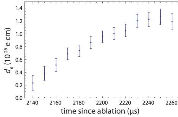
FIGURE 4.5: Variation in d_e across the TOF profile observed when \bar{V} = +102.5 \text{ V} . The range of the horizontal axis is set to the interval of the analysis gate specified in section 4.1.
