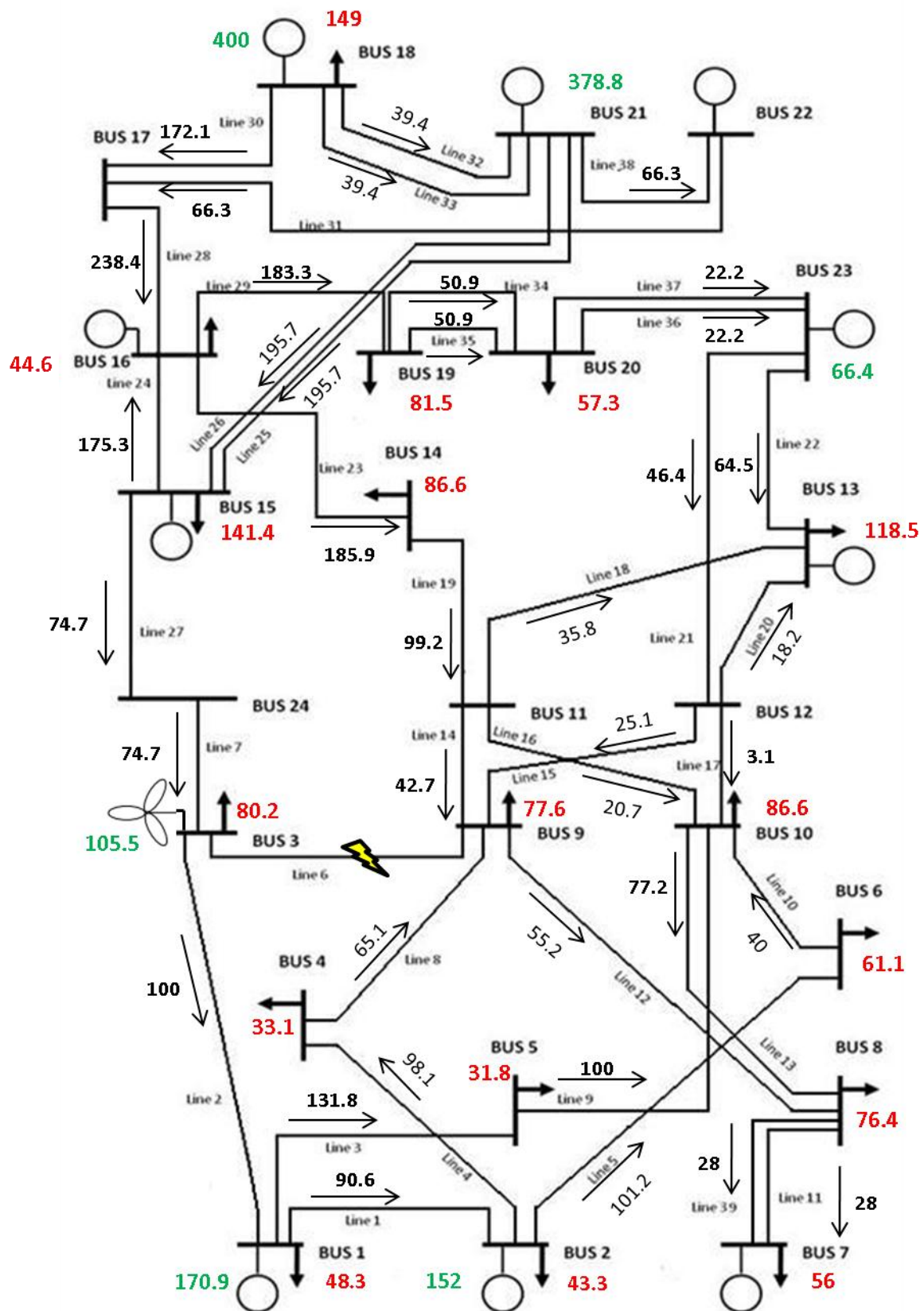
Figure B-2: Optimum generation dispatch and post-fault power flows (line 6 in outage) when no quadrature boosters have been installed. All quantities are in MW.
