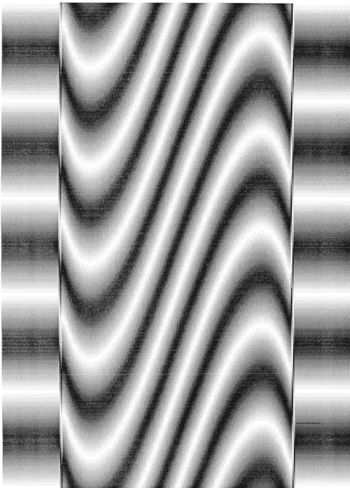
Figure 4.17: Theoretical interferogram : Index mismatch at the rod boundary and a shearing misalignment
