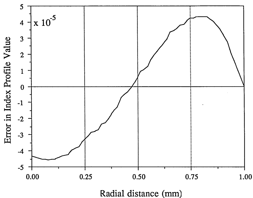
Figure 7.10: Error in the refractive index values of the profile reconstructed using the refractionless limit
