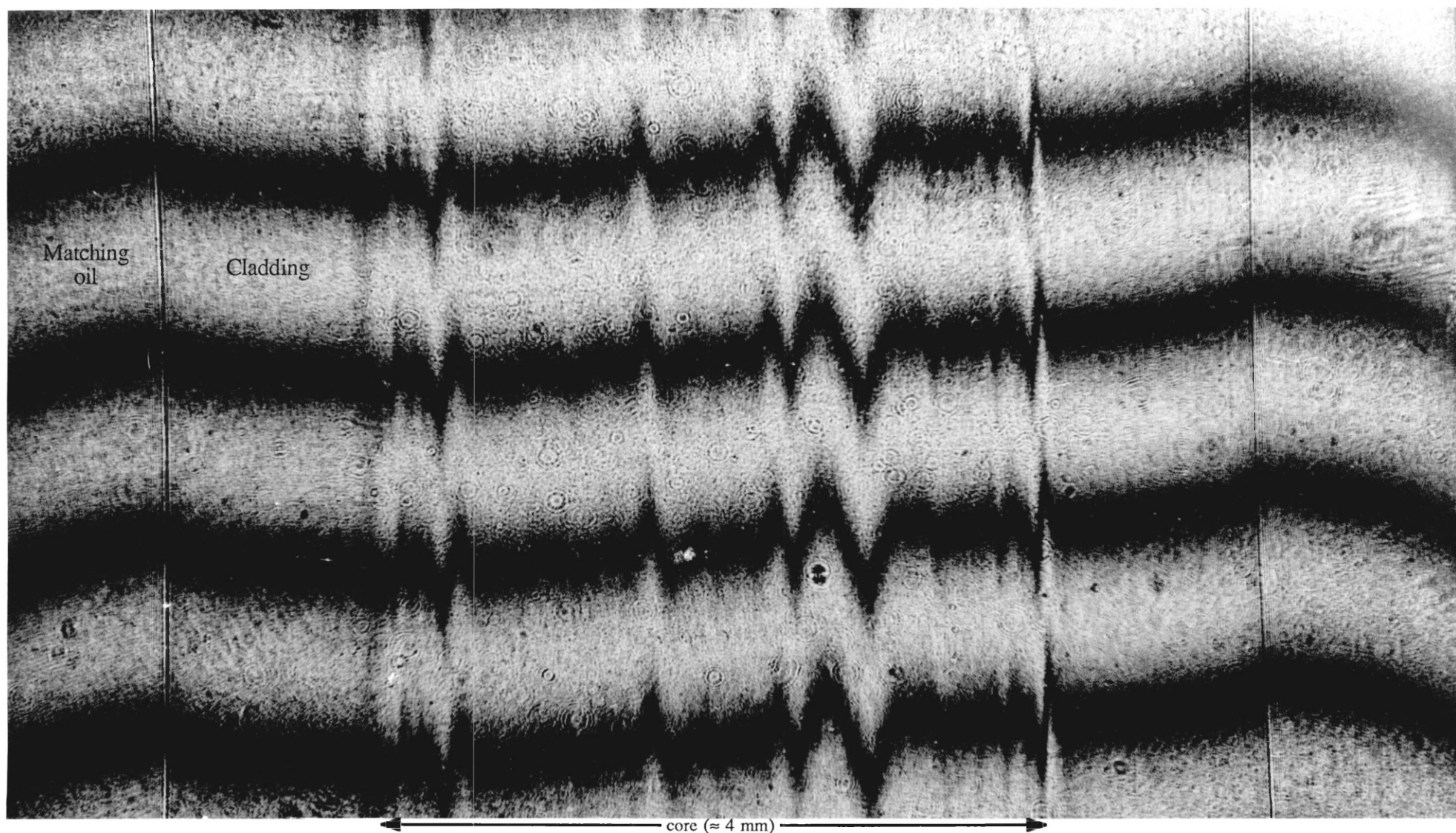
Figure 9.3: Experimental interferogram - Ion stuffing preform: Preform rotated about its axis by 0.5^\circ :
