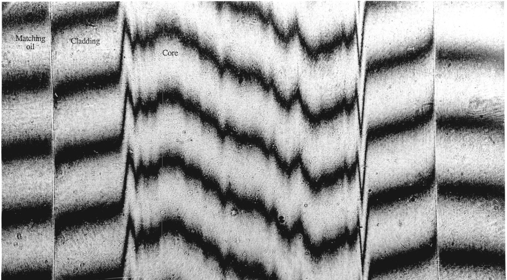
Figure 8.3: Shearing interferogram : Ion stuffing preform
