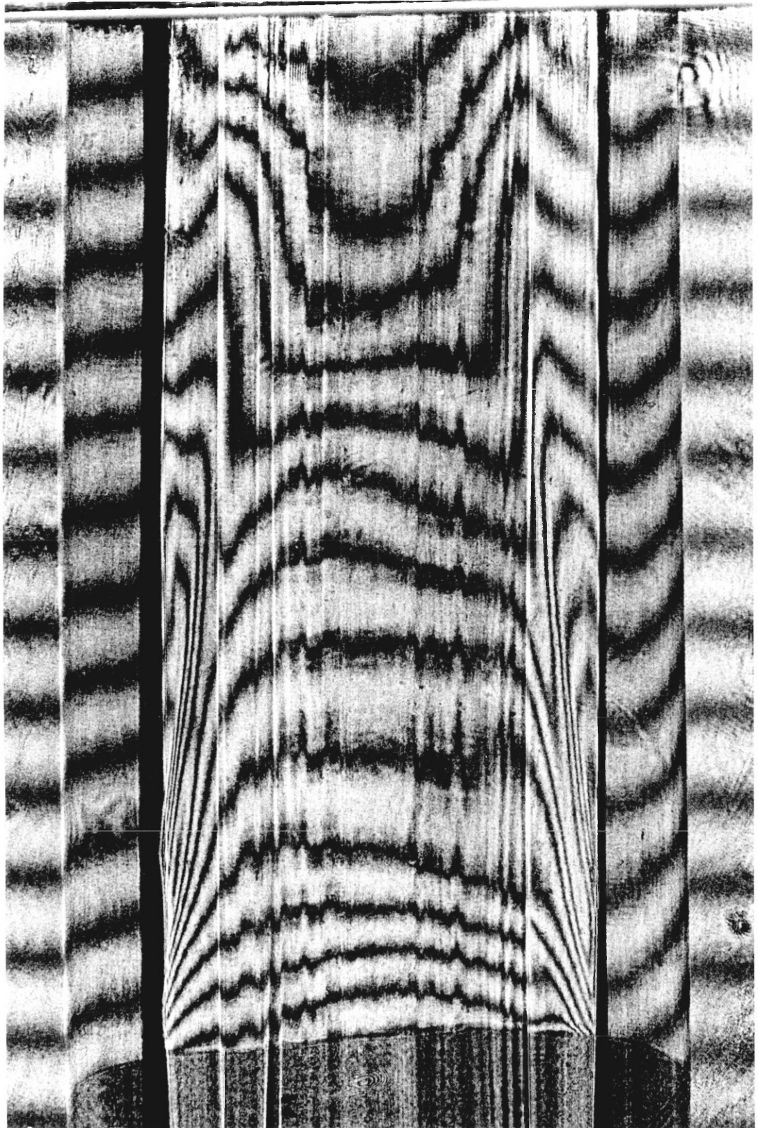
Figure 9.5: Experimental interferogram - Ion stuffing preform: Axial variation of the index distribution.
