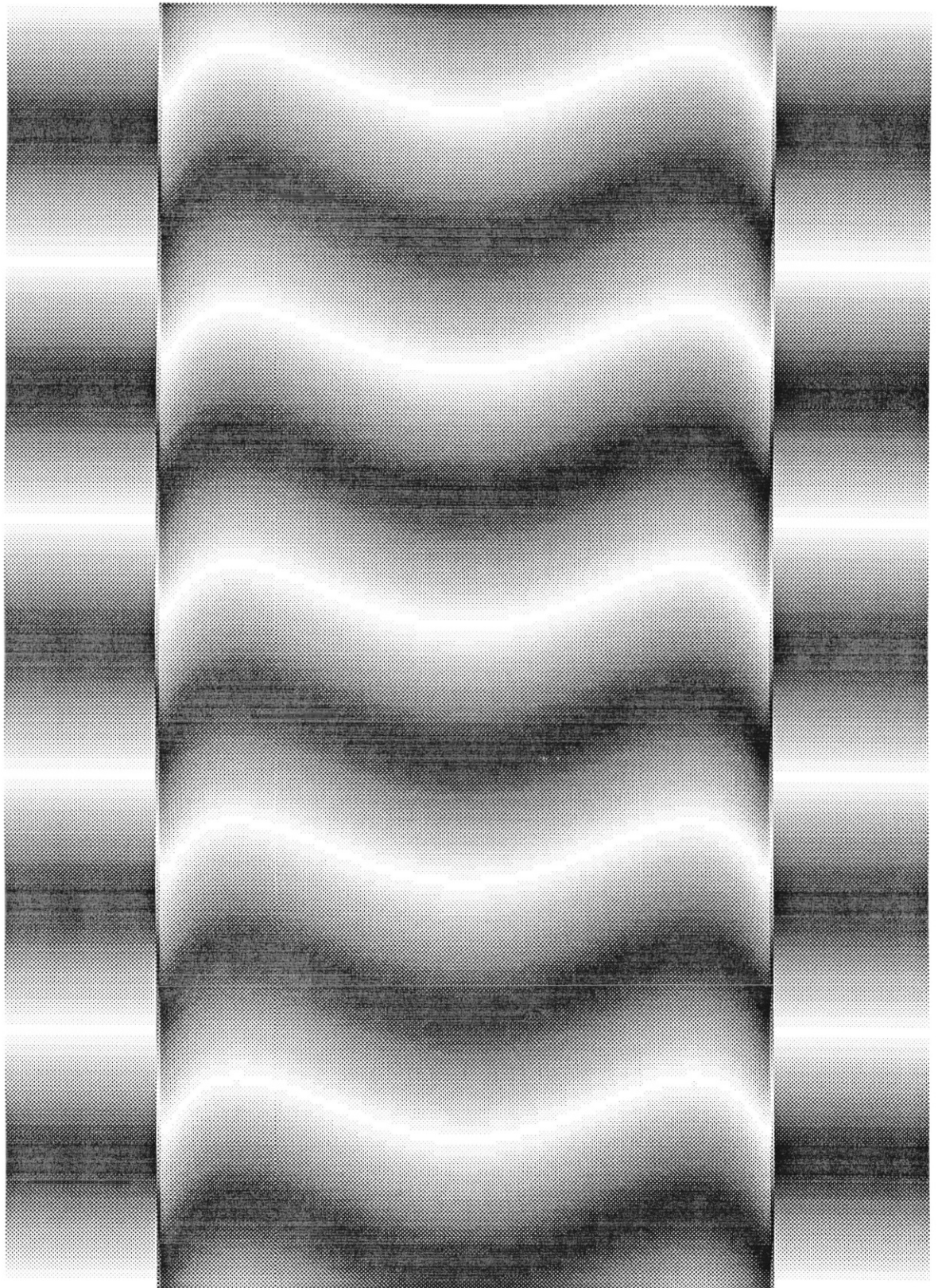
Figure 4.16: Theoretical interferogram : Index mismatch at the rod boundary and a diameter variation
