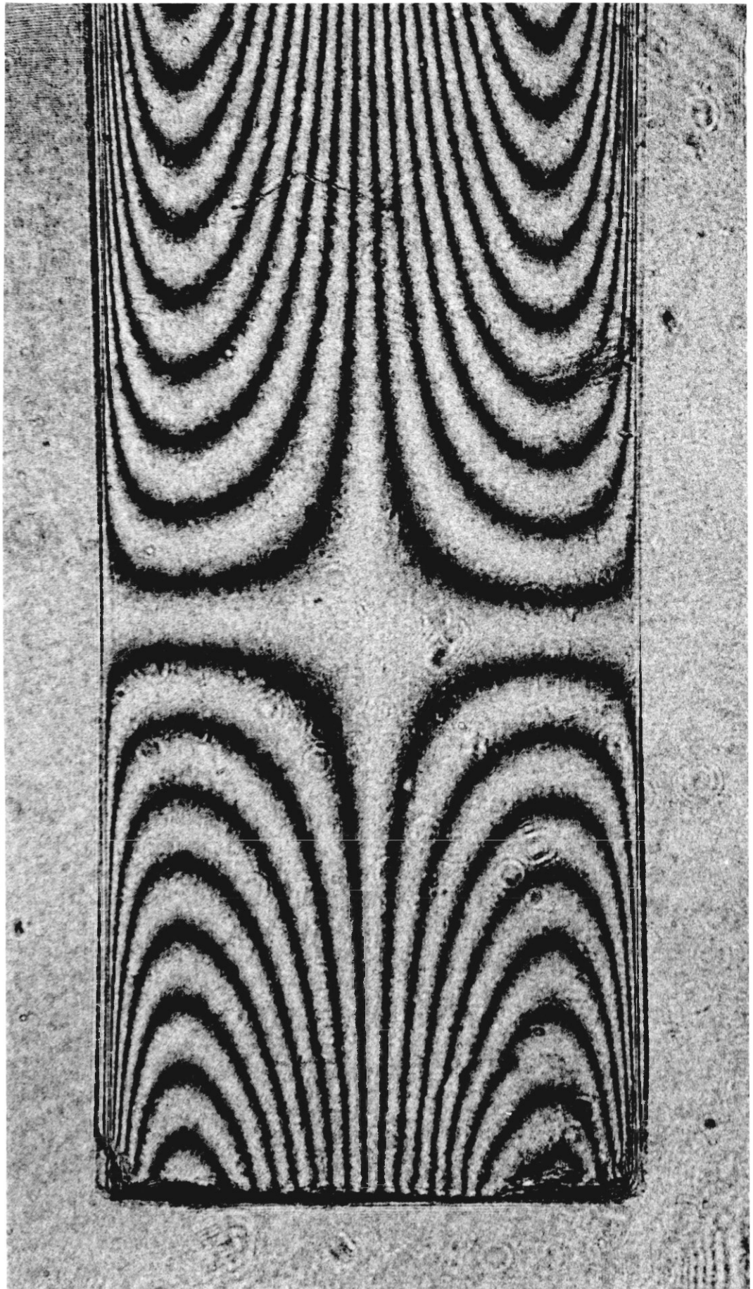
Figure 6.5: Experimental interferogram : Tilt misalignment of the test rod
