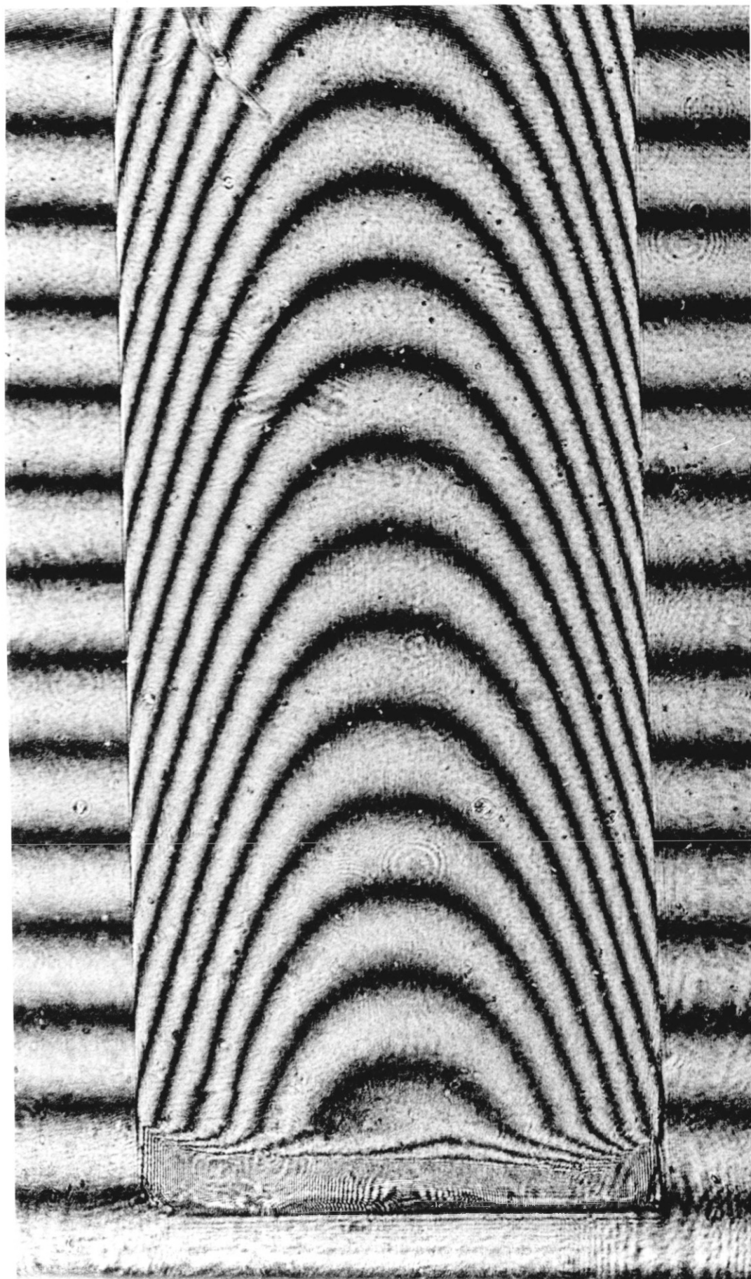
Figure 9.12 : Experimental interferogram - Graded index rod lens: Comparison of rod samples C and B.
