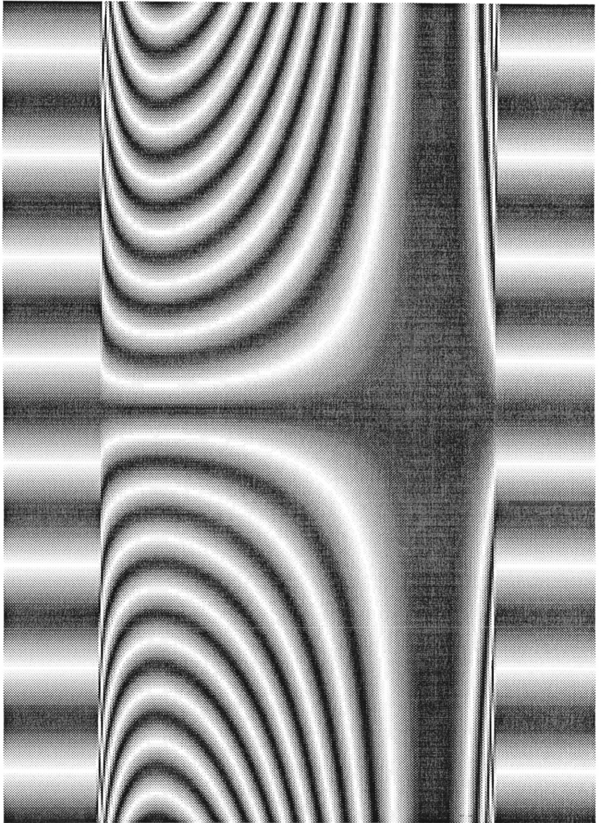
Figure 4.15: Theoretical interferogram : Rotation of rod about optical axis
