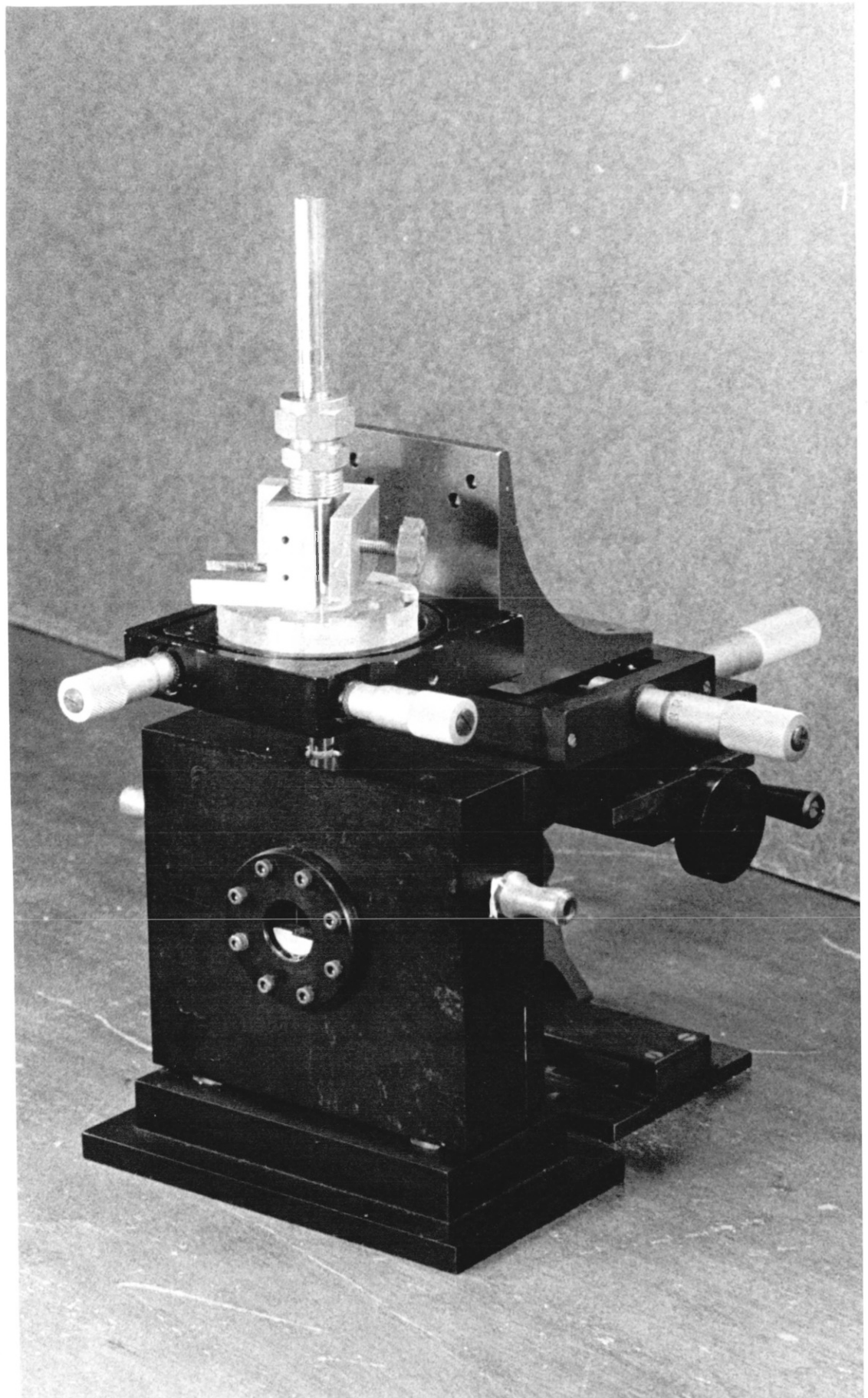
Figure 5.6: The optical cell and rod lens mounting apparatus
