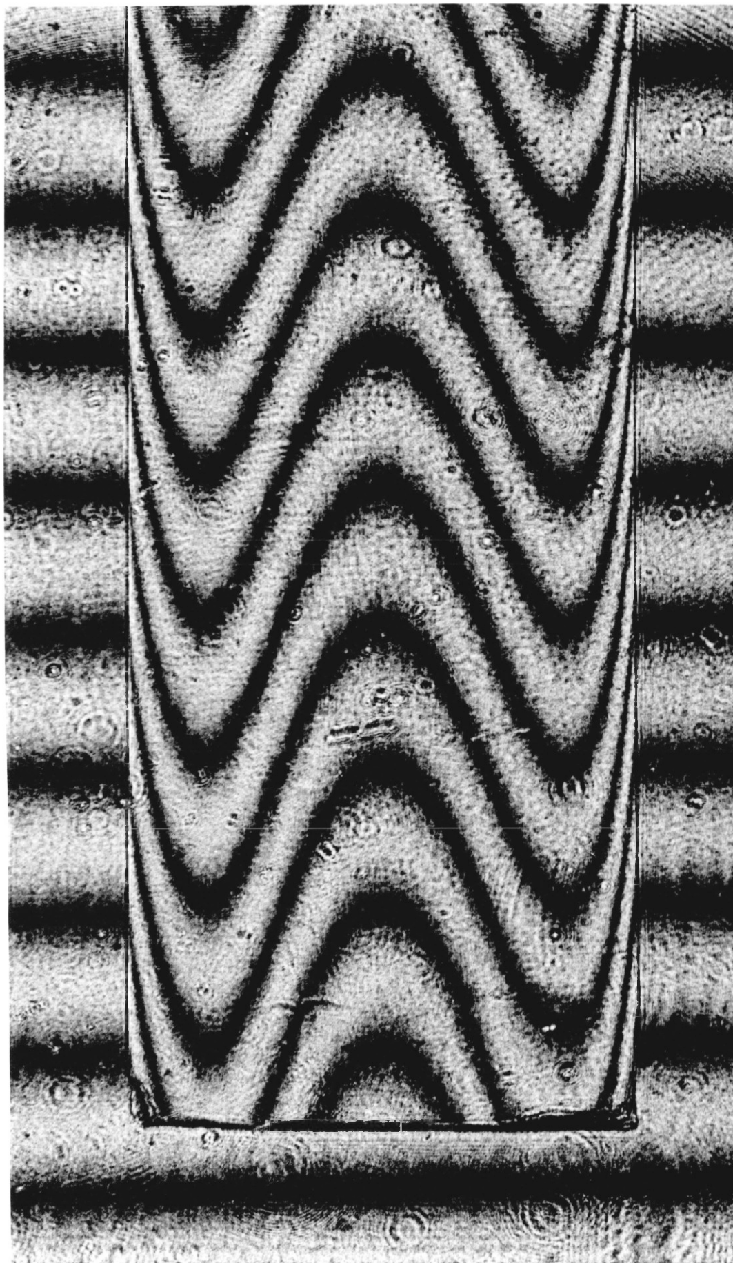
Figure 6.7: Experimental interferogram : Defocus misalignment of the test rod
