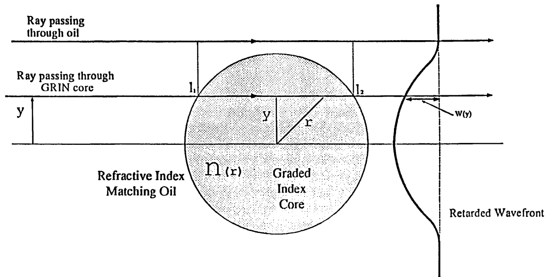
Figure 4.2: The Refractionless Limit Approximation
