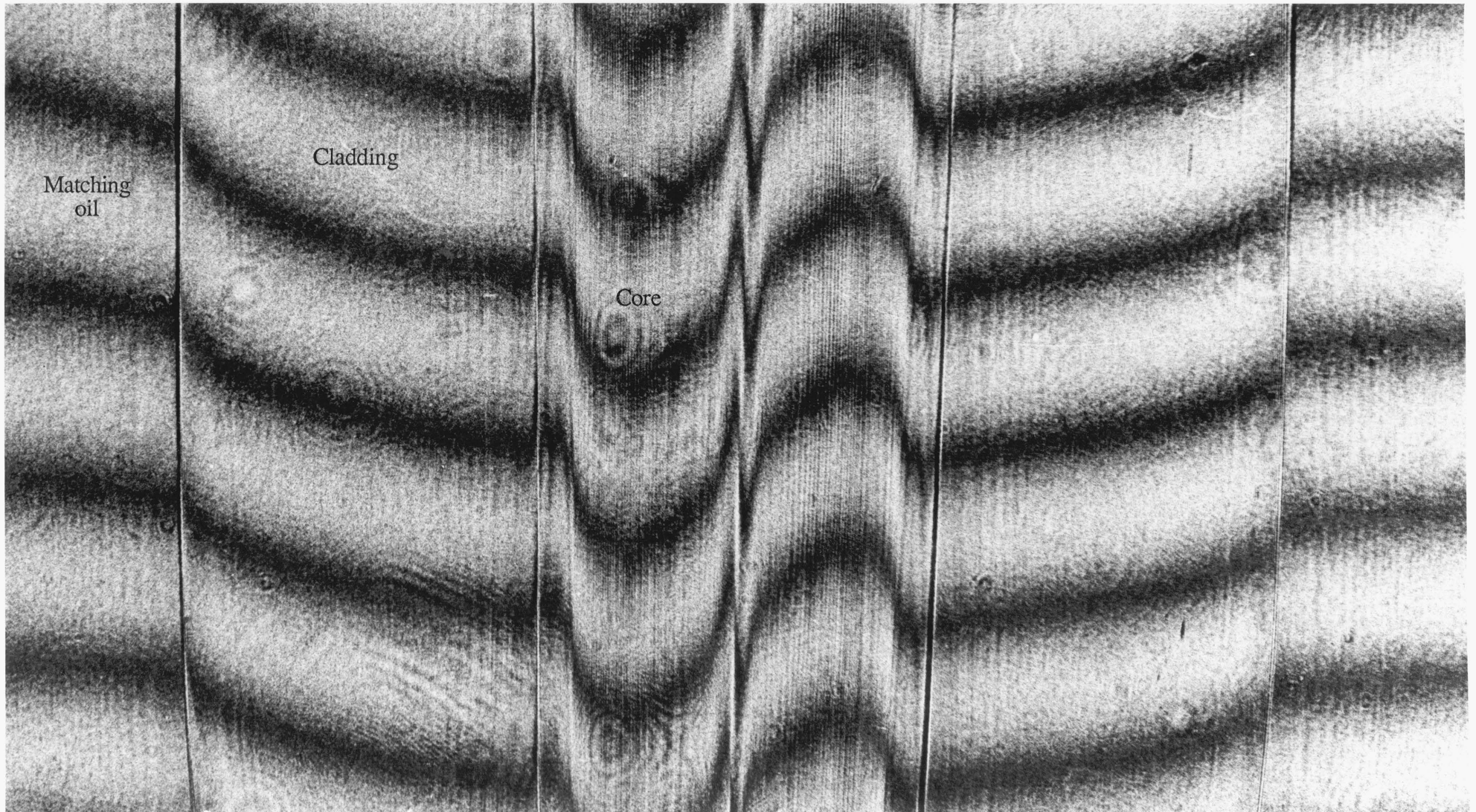
Figure 8.2: Shearing interferogram : Ion deposition preform
