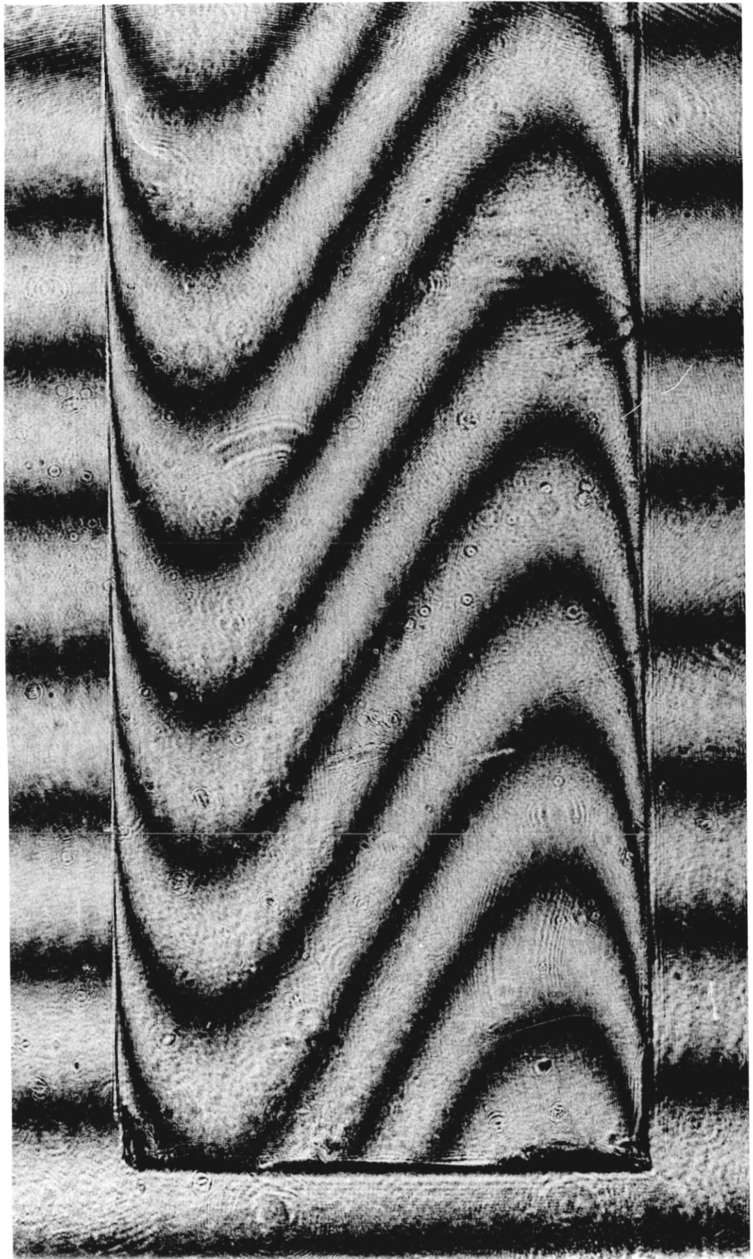
Figure 8.7: Shearing interferogram : Graded index rod micro lens
