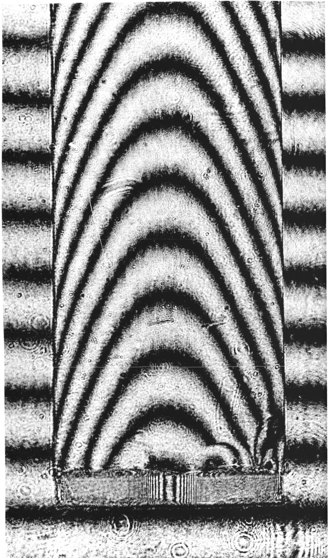
Figure 9.7: Experimental interferogram - Graded index rod lens: Comparison of rod samples A and B.
