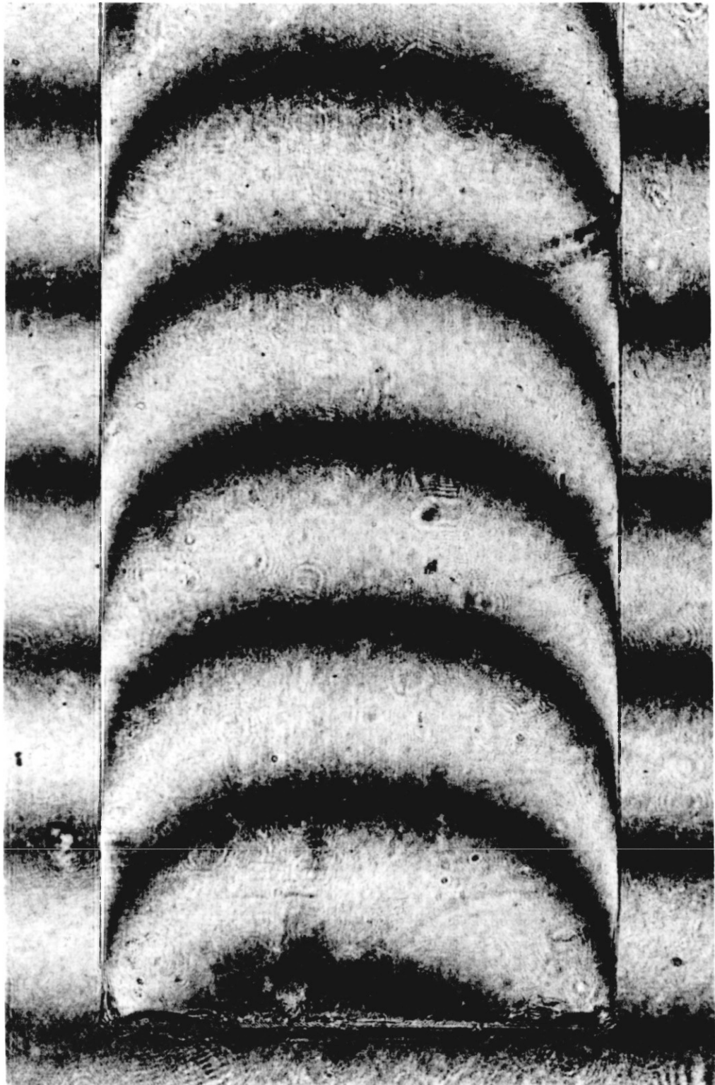
Figure 6.1: Experimental interferogram : Change in the matching oil temperature of 1°C
