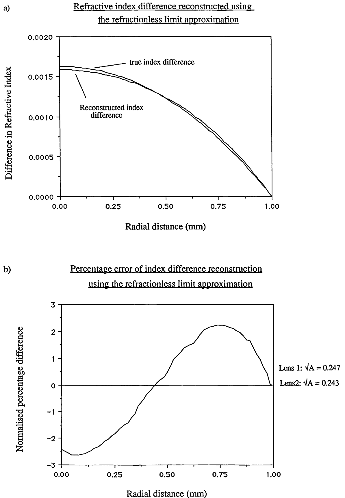
Figure 7.9: Error of reconstructing the refractive index difference using the refractionless limit approximation
