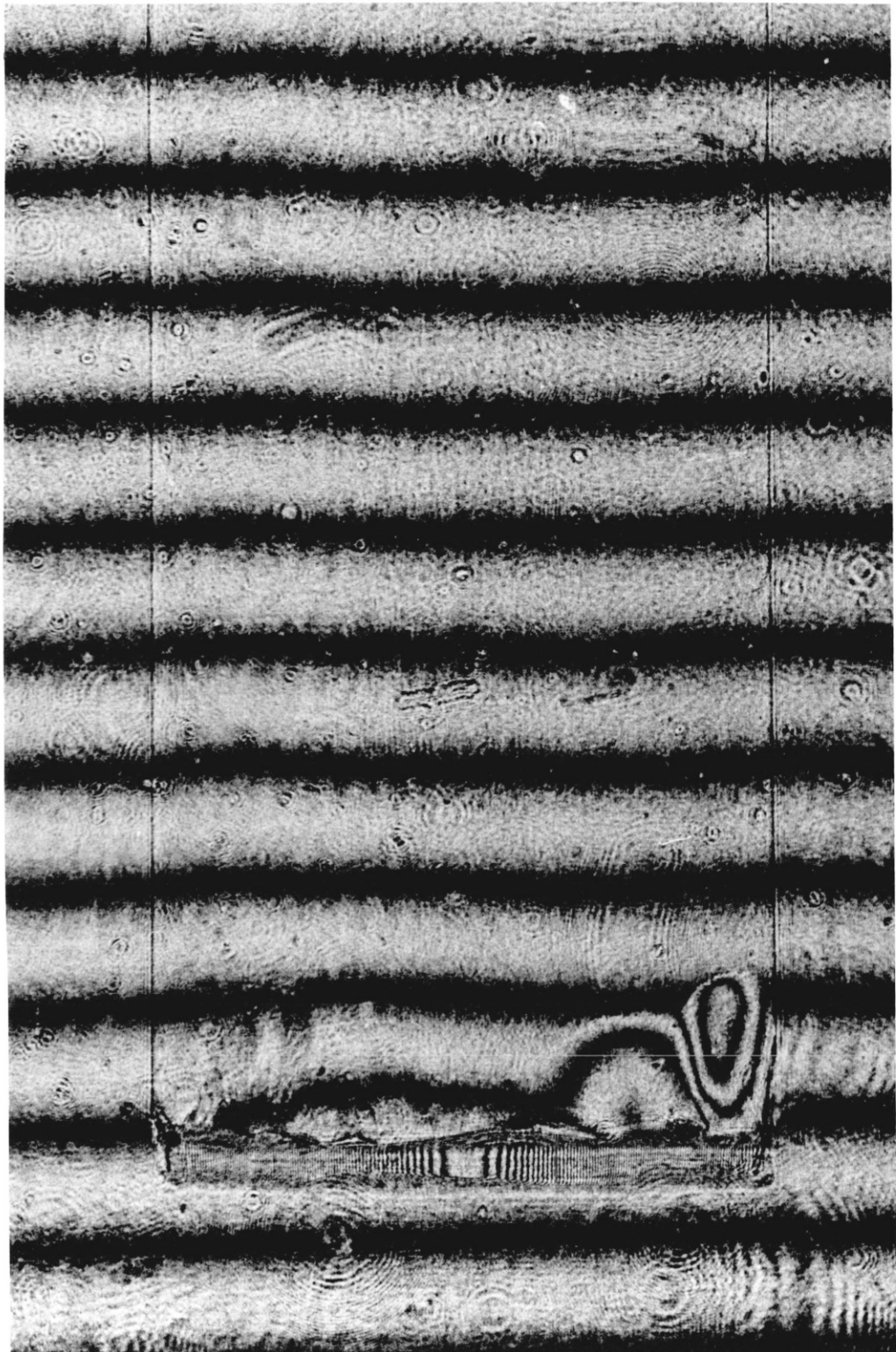
Figure 6.10: Experimental interferogram : Test rod realigned in the optical cell
