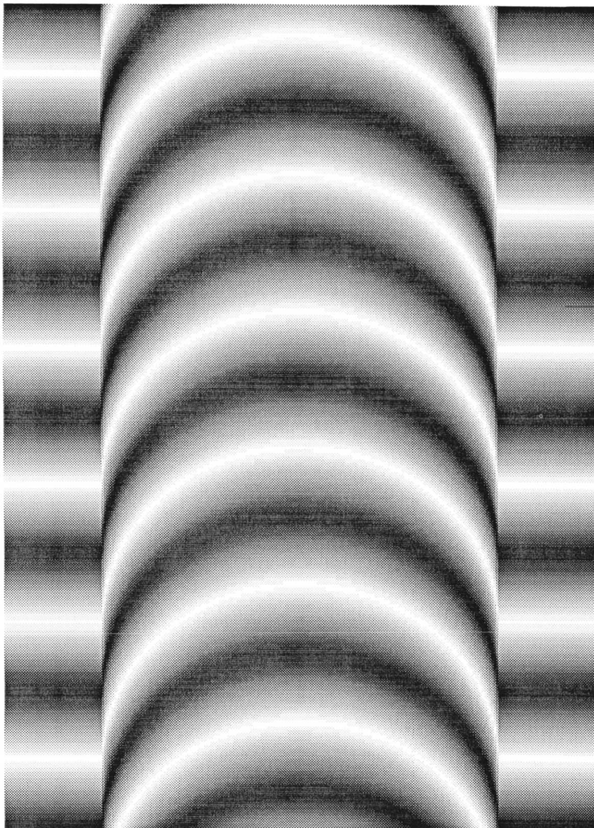
Figure 4.18: Theoretical interferogram : Change in the index matching oil temperature of 1°C
