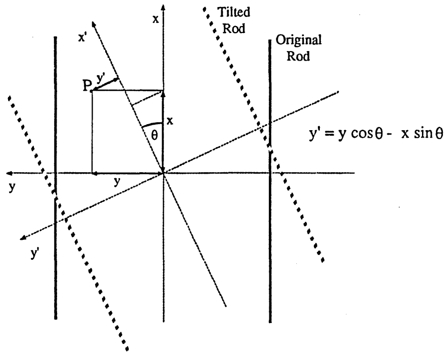
Figure 4.14: Rotation of Rod about the Optical Axis
