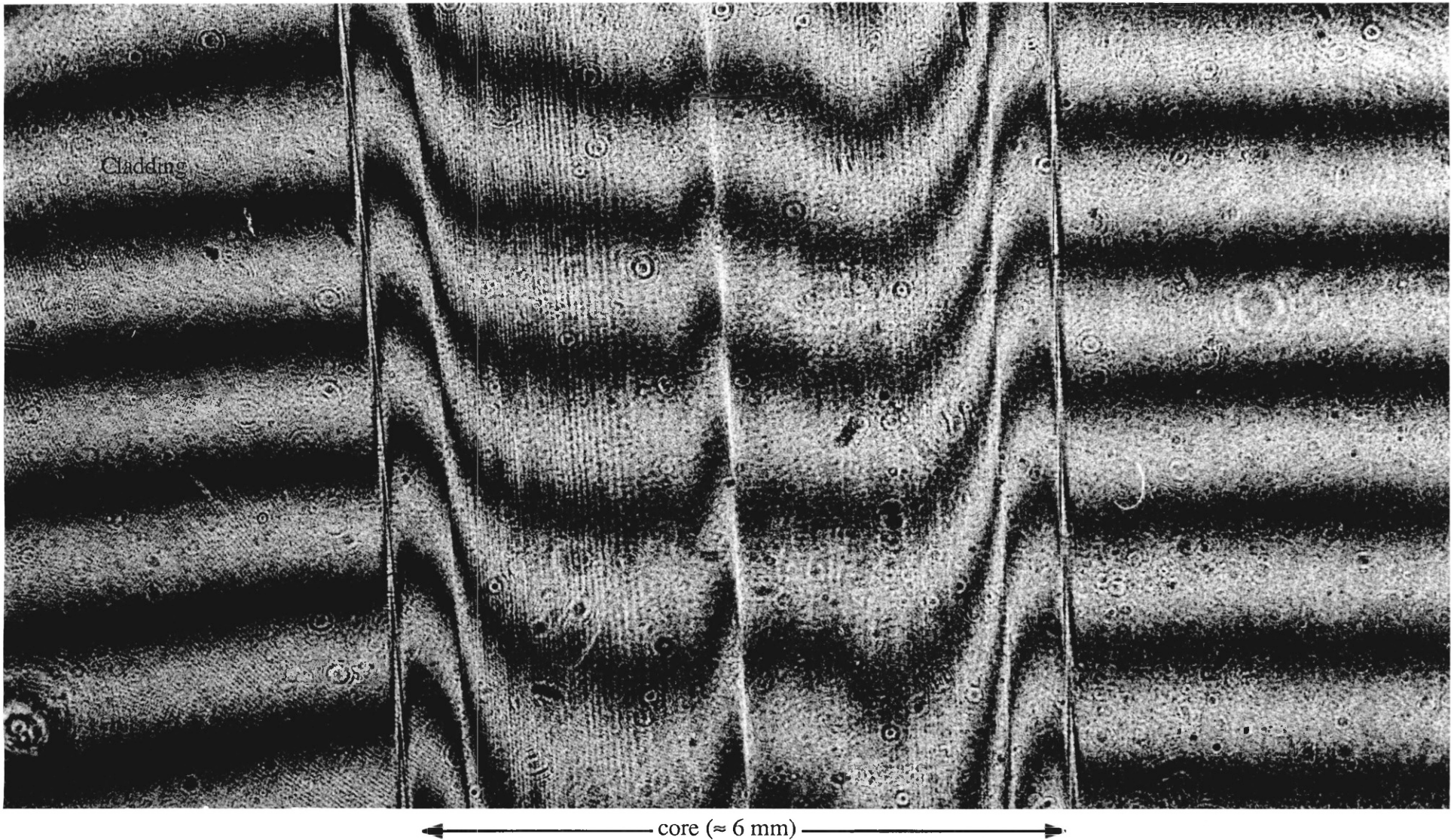
Figure 9.2: Experimental interferogram - Ion deposition preform Preform displaced vertically by \approx 10 mm
