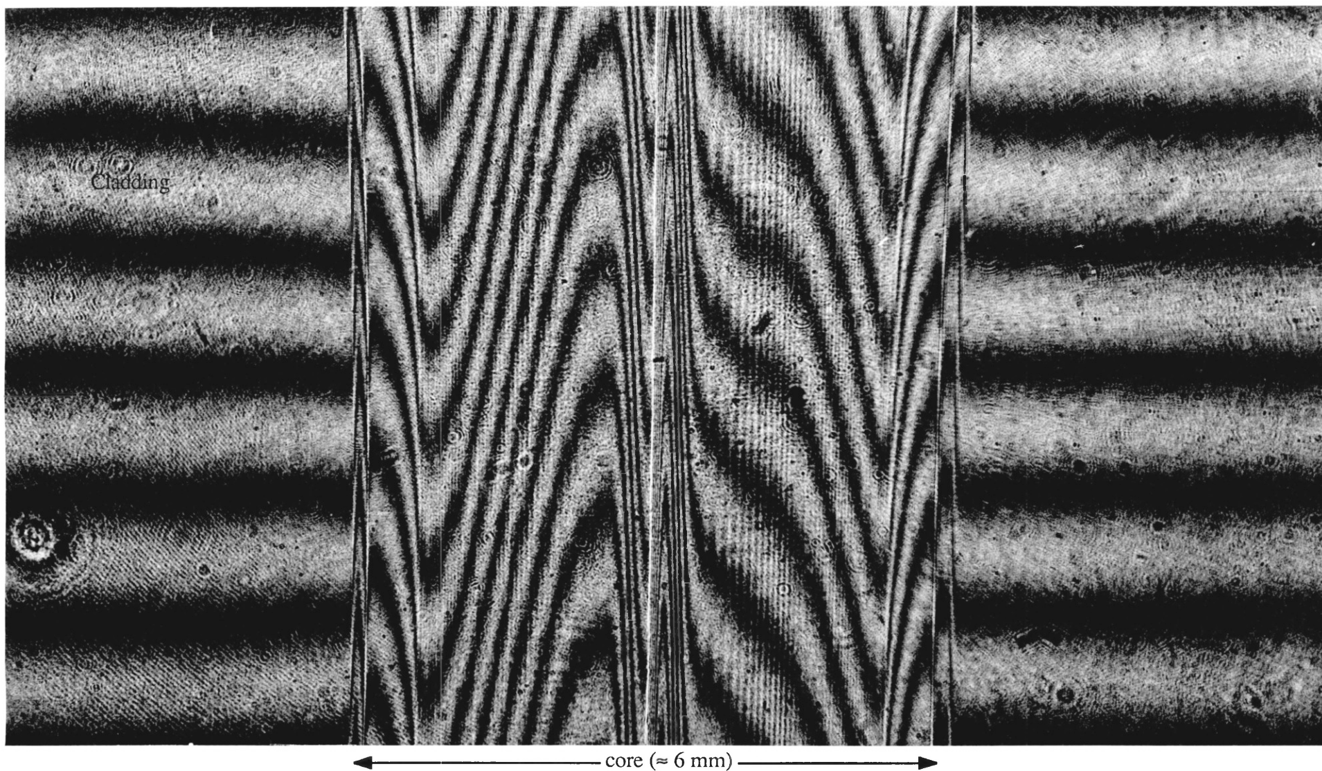
Figure 9.1: Experimental interferogram - Ion deposition preform Preform rotated about its axis by 90°
