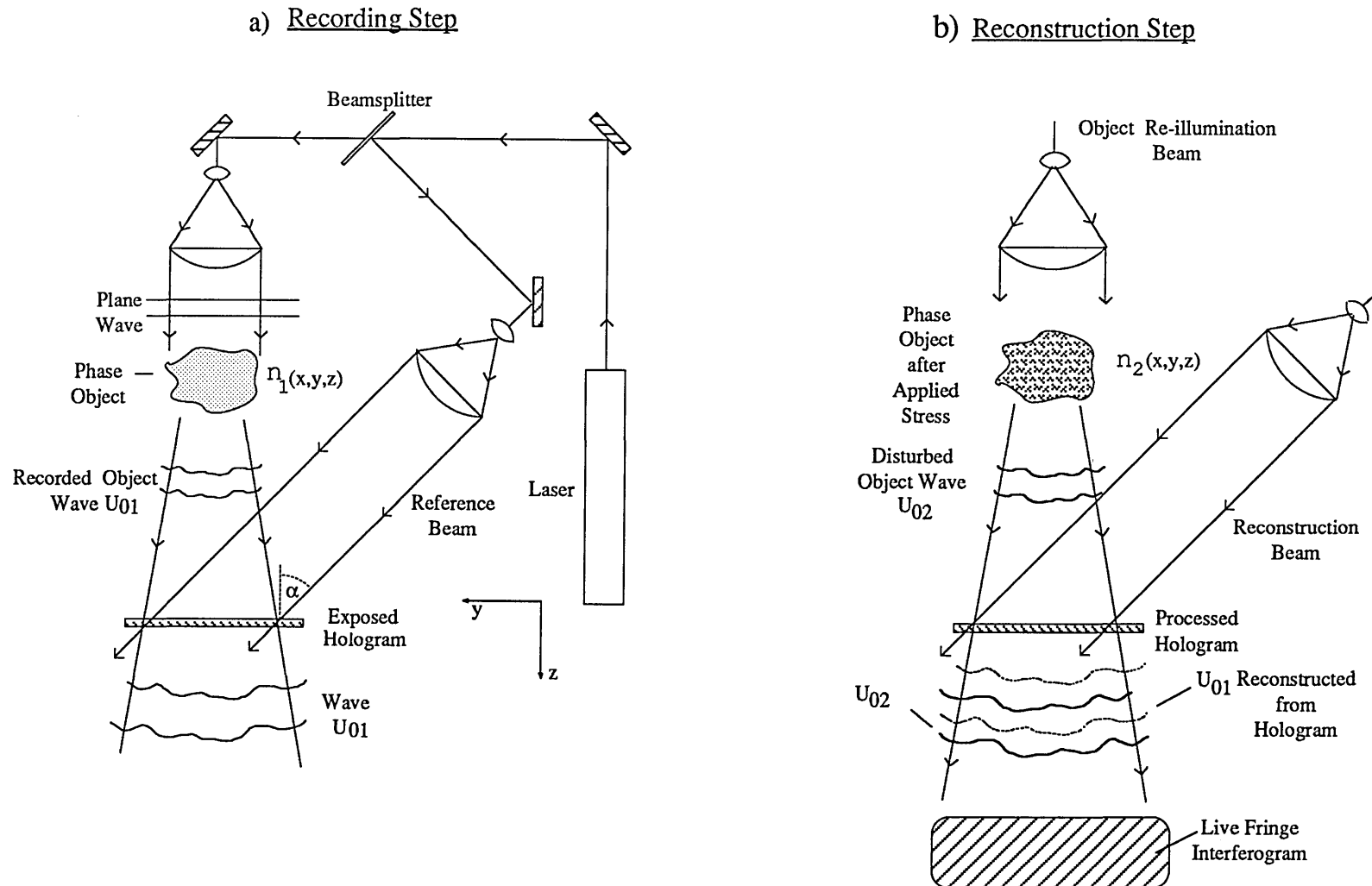
Figure 3.2: Holographic Phase Interferometry
