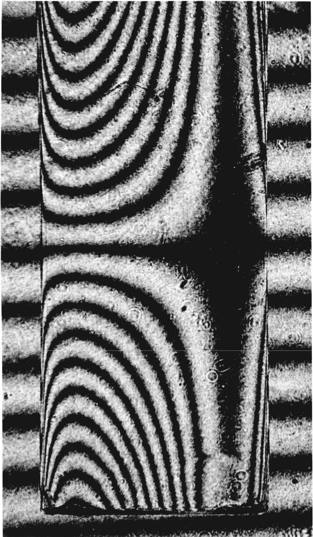
Figure 6.6: Experimental interferogram : Towards a realignment of the test rod
