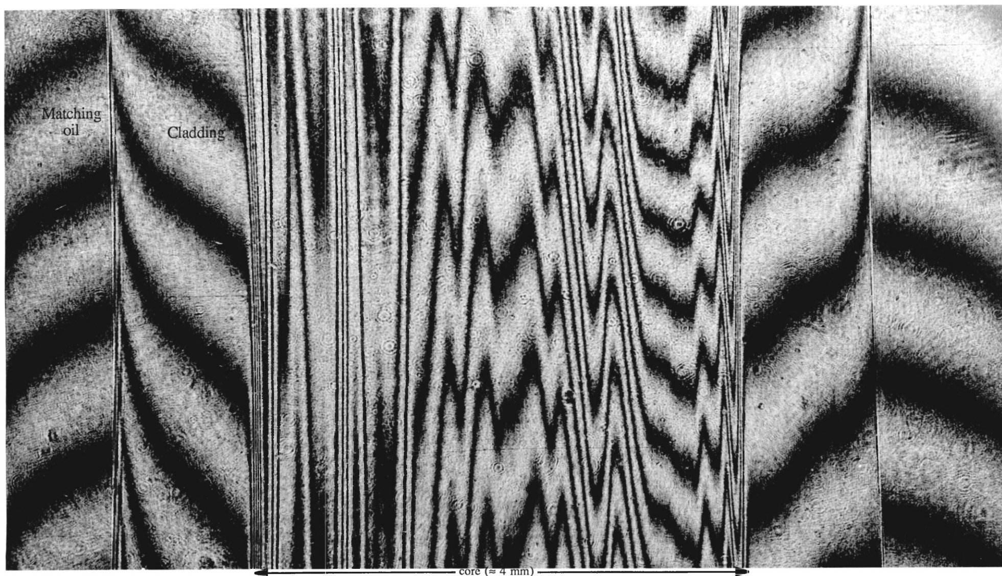
Figure 9.4: Experimental interferogram - Ion stuffing preform: Preform rotated about its axis by 90°:
