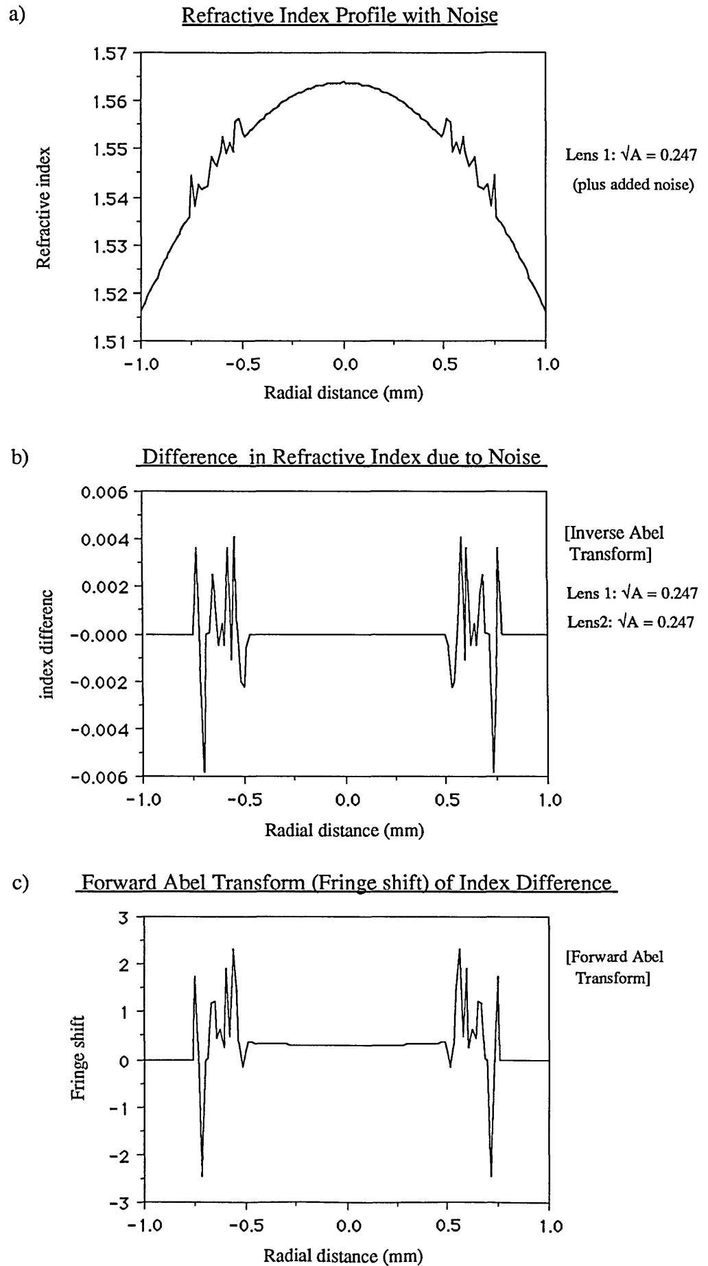
Figure 7.3: Computing a fringe shift for profiles having a random fabrication error
