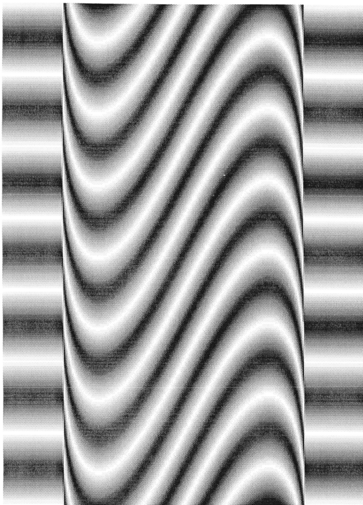
Figure 4.11: Theoretical interferogram : Shearing misalignment of the rod
