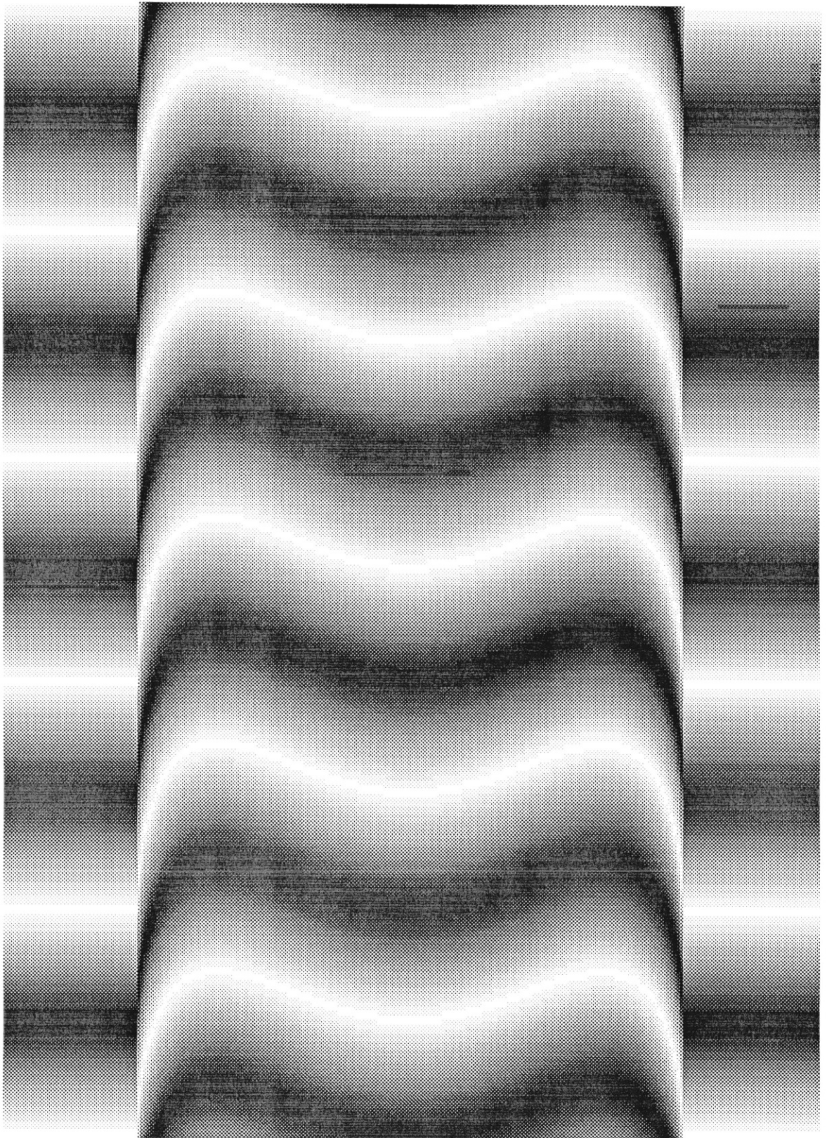
Figure 4.8: Theoretical interferogram : 10 micron change in the diameter of the rod
