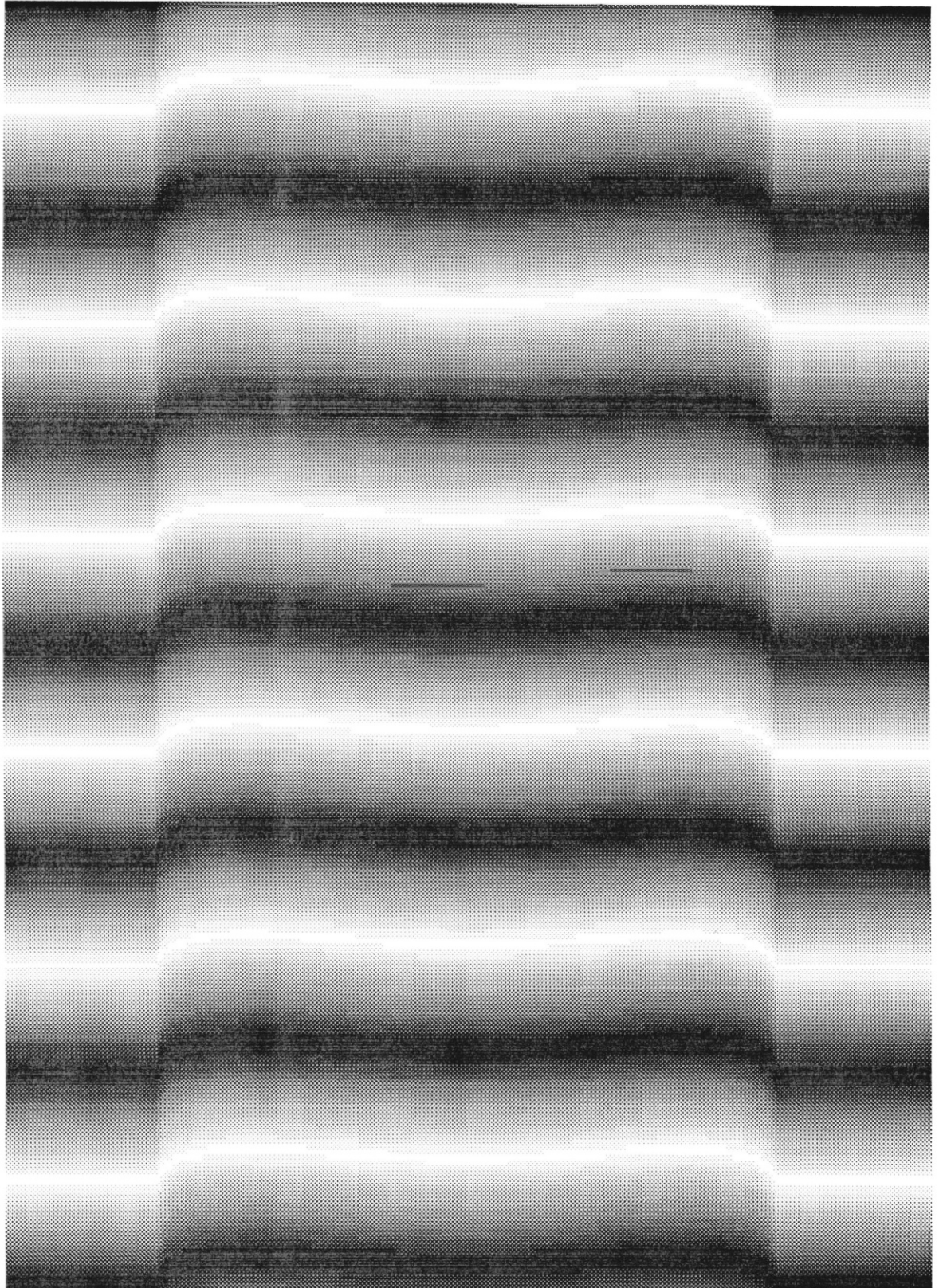
Figure 7.17: Theoretical interferogram : A 2 micron change in the diameter of a 2mm rod lens
