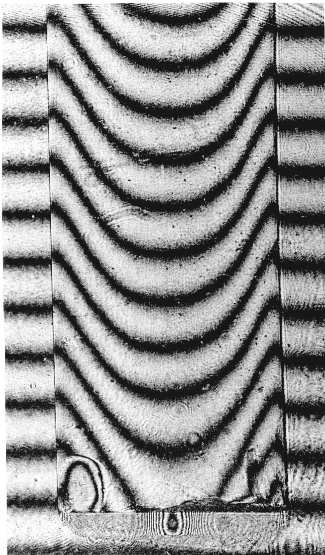
Figure 9.9: Experimental interferogram - Graded index rod lens: Comparison of rod samples A and C.
