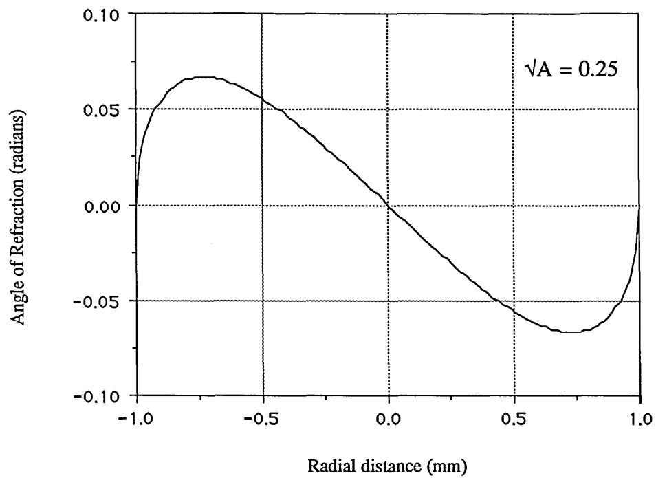
Figure 7.6: The deflection function for a graded index rod lens
