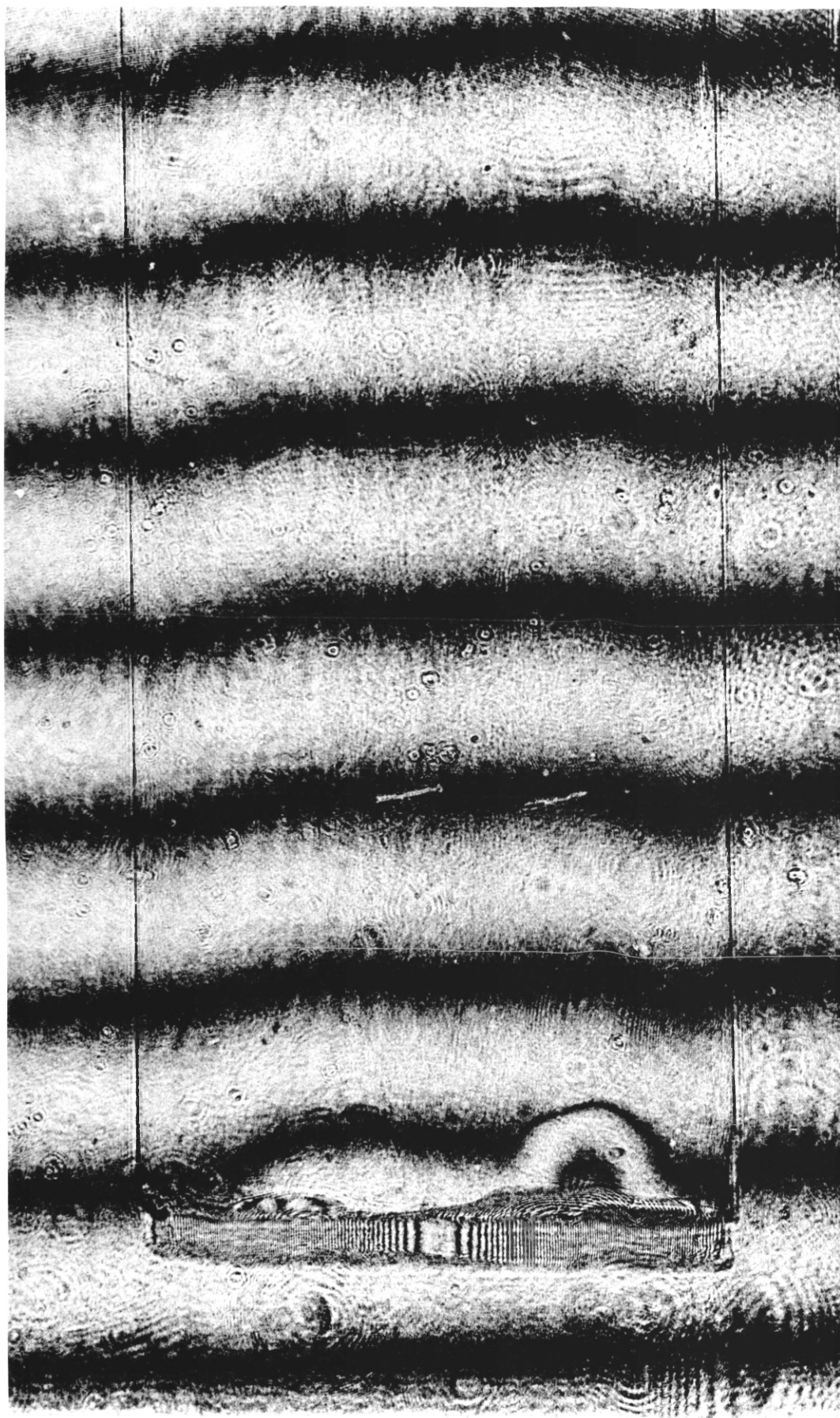
Figure 9.6: Experimental interferogram - Graded index rod lens: Comparison of rods produced within the same production lot.
