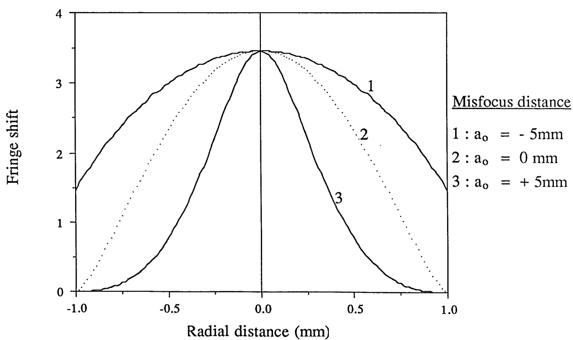
Figure 7.11: Fringe shift as a function of the misfocus of the observation plane
