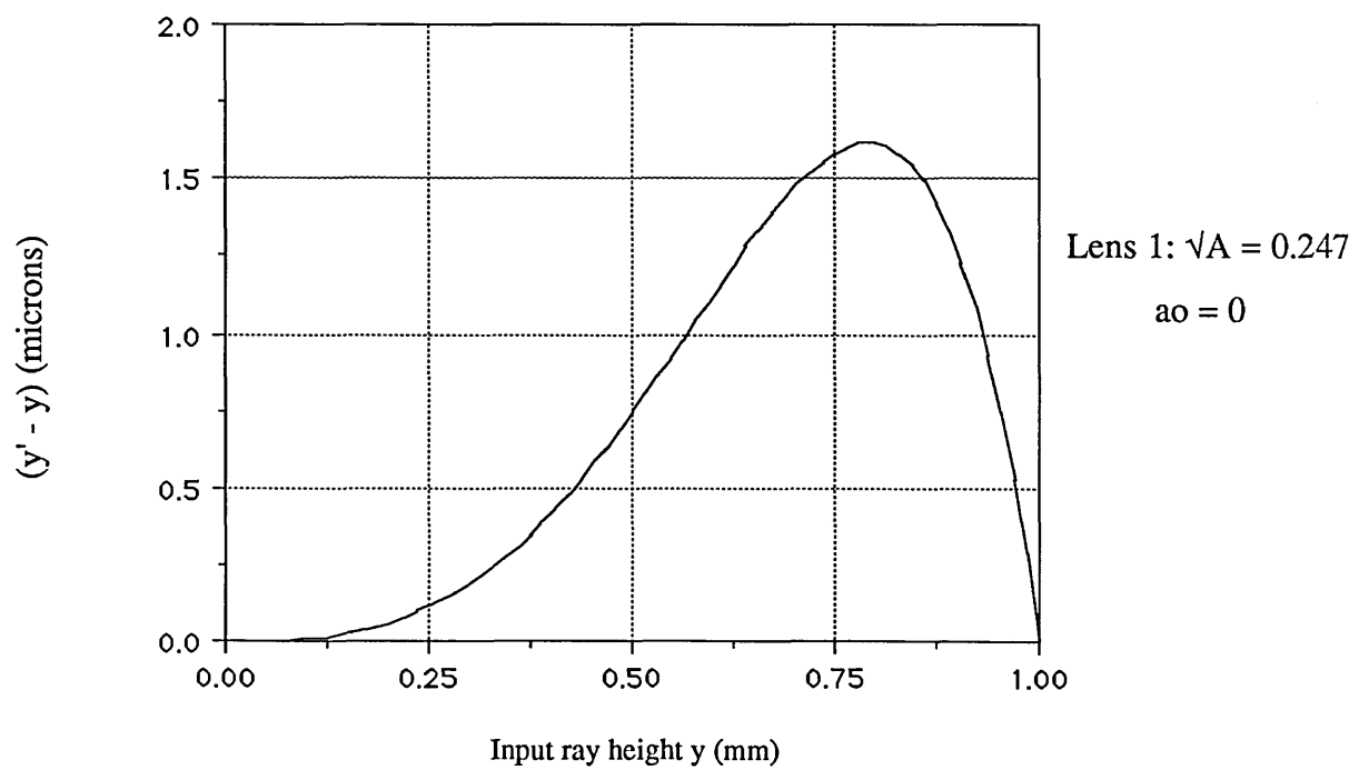
Figure 7.7: Difference between Apparent ray height and Input ray height
