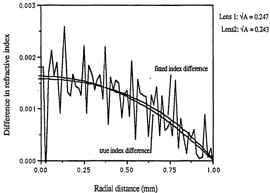
Figure 13: Fitting an even order power series to the reconstructed index difference
