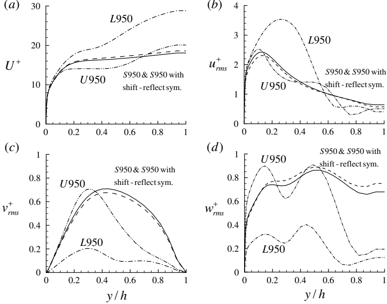
FIGURE 4. The wall-normal profile of (a) mean velocity and (b) streamwise, (c) wall-normal, (d) spanwise velocity fluctuations: —, S950; ---, the symmetry-constrained S950; ·····, U950; -·-·-, L950.
