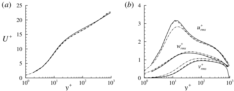
FIGURE 1. (a) Mean velocity and (b) turbulent velocity fluctuations: —, half channel simulation with C_s = 0.05 (F950); ---, full channel simulation with C_s = 0.05 (Hwang & Cossu 2011); - · - · -, DNS at Re_\tau = 934 by del Álamo et al. (2004).
