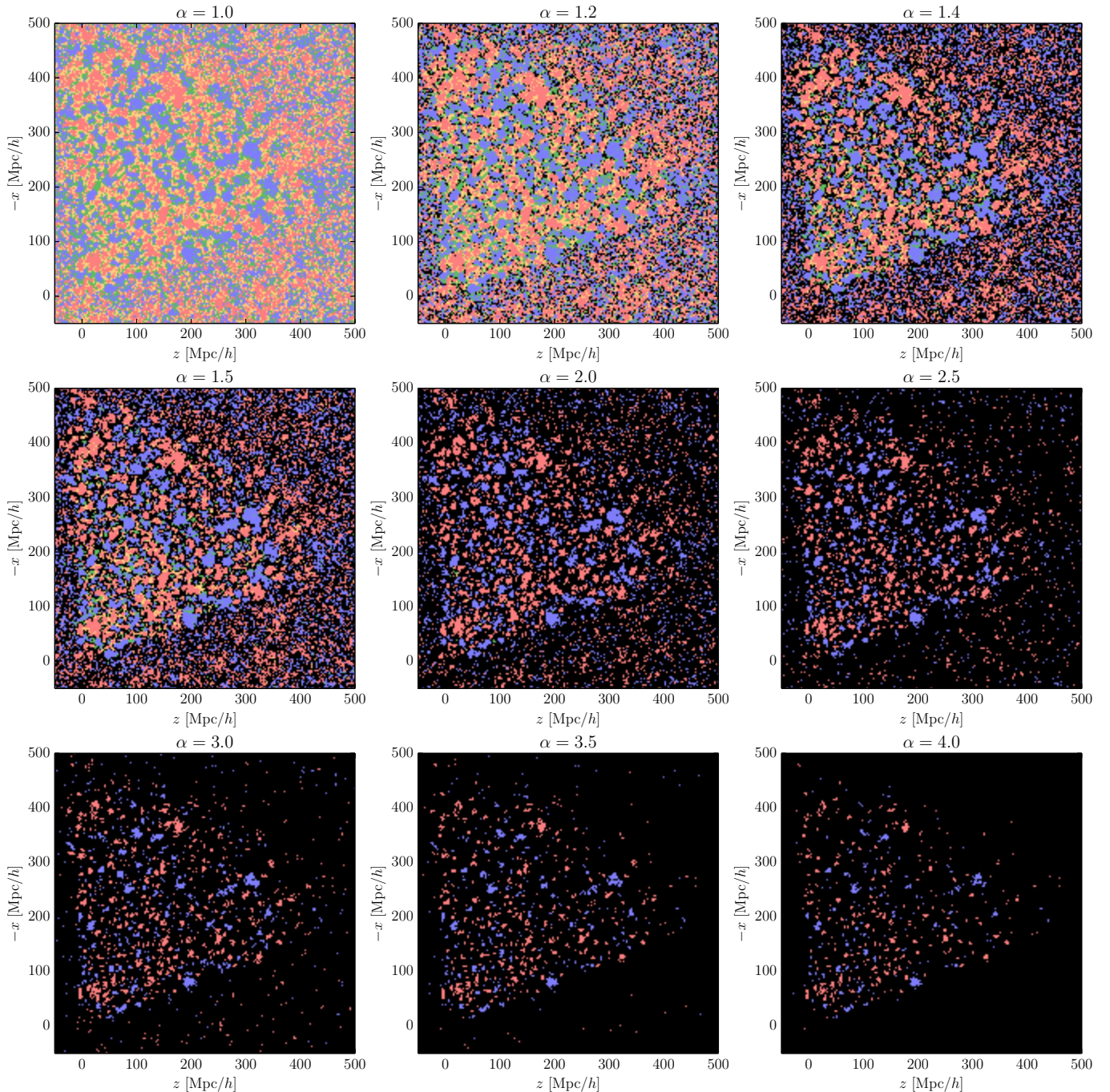
FIG. 2. Same as figure 1 for the primordial large-scale structure, at a = 10^{-3} .
