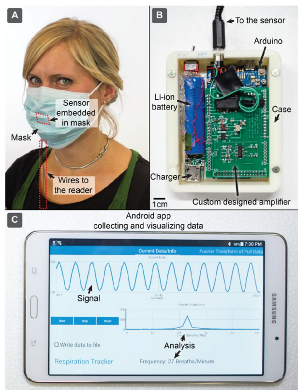
Figure 3. (A) The facemask with the embedded paper-based sensor. (B) Photograph of the data acquisition electronics with Li-ion batteries, Arduino microcontroller board, custom designed amplifier board, and 3D printed casing. (C) Photograph of tablet computer running the Android app, which can display and analyze the incoming data stream from the data acquisition electronics.
