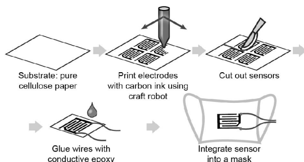
Figure 2. Schematic illustration of the fabrication of digitally printed paper sensors with graphite ink.
