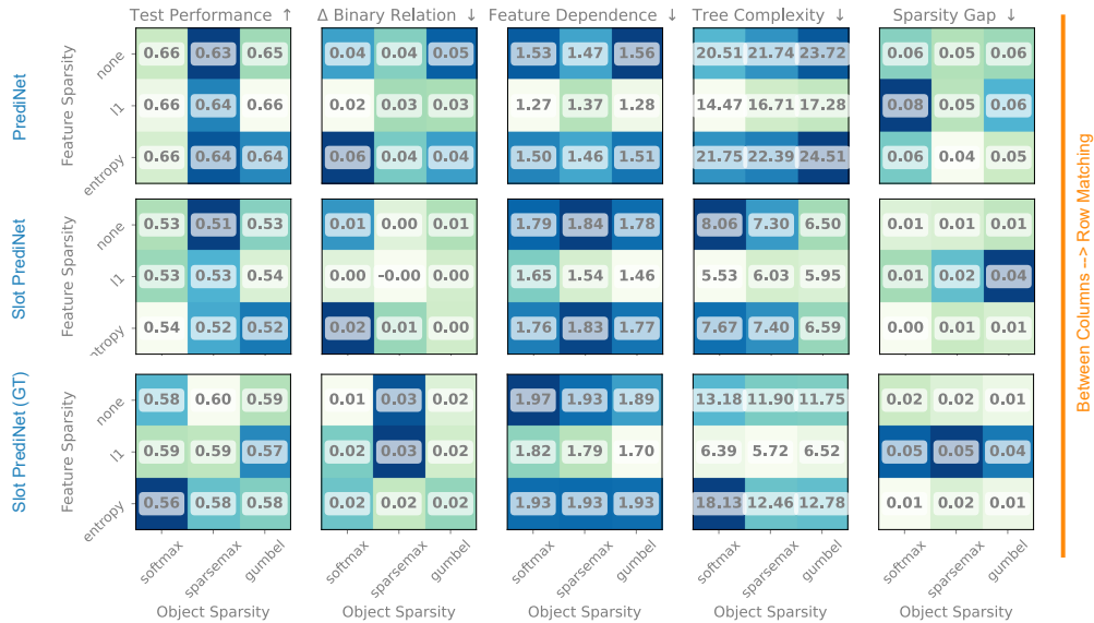
Figure C.3: Sparsity sweeps on the Between Columns Row Matching curriculum.
