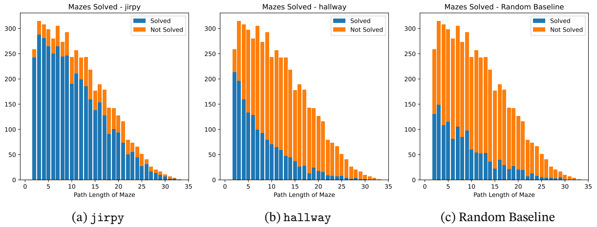
Figure E.1: Performance of our models on a held-out test set of RDFS mazes. Noticeably, the performance appears roughly consistent over path length for jirpy which was trained to solve mazes, and similarly for the random baseline (which follows corridors and chooses a random continuation of its path when reaching a fork). The hallway model, on the other hand, is able to “solve” some of the very short mazes but struggles with longer mazes (where it is likely to encounter forking points).
