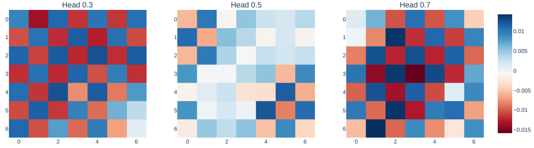
Figure F.11: Stan scalar products of query vector for ; token and key vectors for maze-cell tokens, arranged on maze grid. Note the clear correspondence with Figure 9.3. These patterns account for why LH03 directs its attention to even-parity cells, while odd-parity cells are attended to by LH07 or LH05.
