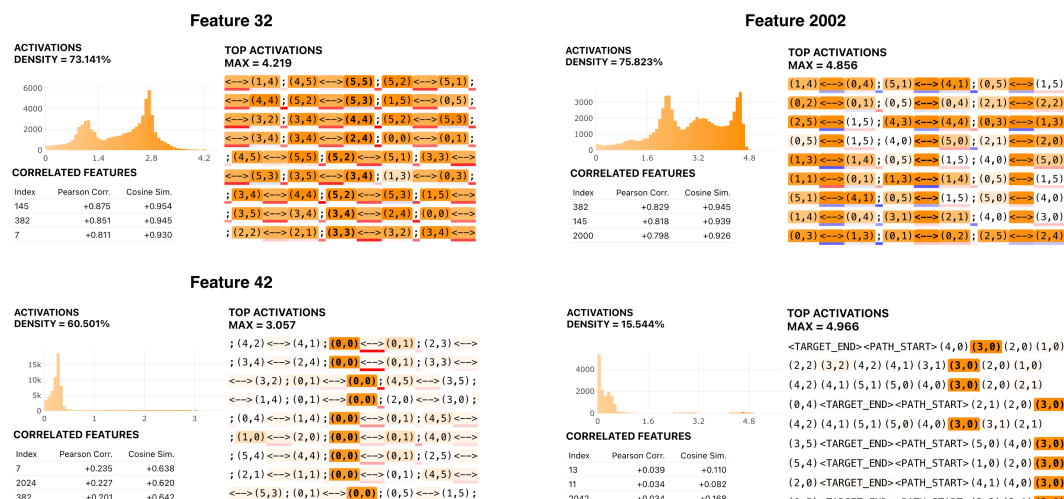
(a) Representative SAE features for Terry.
