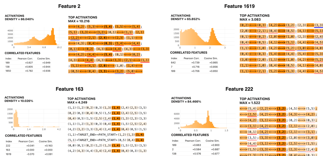
(b) Representative SAE features for Stan.
