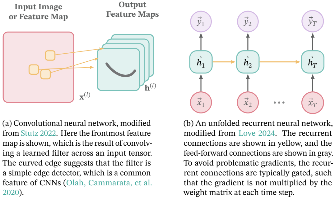
Figure 2.2: Two foundational neural network architectures that encode distinct inductive biases: (a) CNNs leverage spatial locality through shared filters that detect features across image regions, while (b) RNNs process sequential data by maintaining temporal state through recurrent connections.
