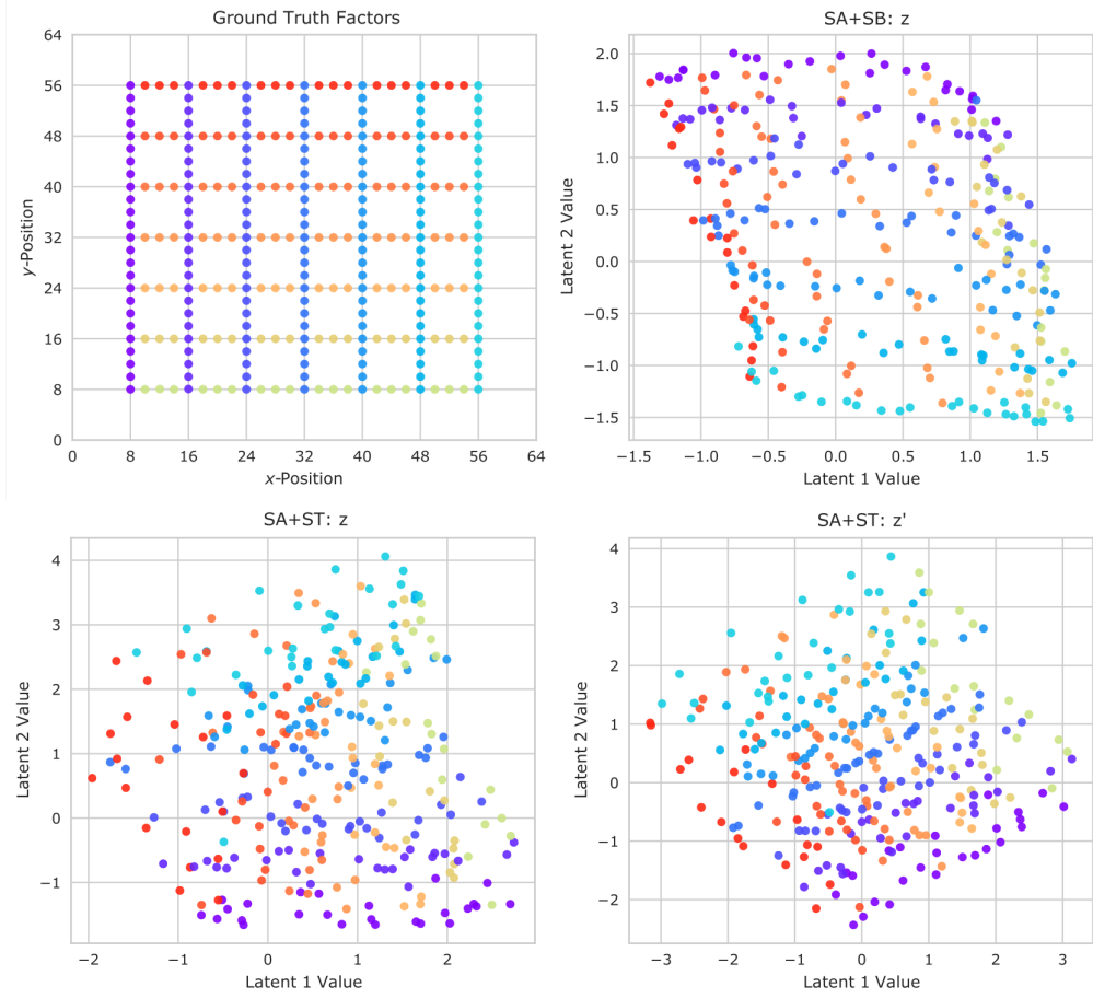
Figure 4.6: Latent manifolds obtained by i) taking the two elements of a latent which had the highest associated feature importance on regressors for ground truth position, and ii) finding the values of those latent elements when encoding objects whose positions corresponded to the x, y grid shown in the upper left. From the learned mapping we can qualitatively gauge the explicitness of the representation for position — In this case, both SB and ST do well, though ST more consistently learned a highly explicit mapping across our runs.
