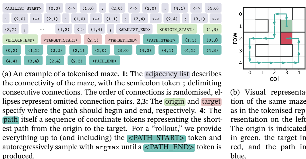
Figure 7.2: Tokenisation scheme and visualisation of a shortest-path maze task generated using the MazeDataset library (Ivanitskiy, Sandoval, et al. 2025).
