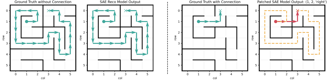
Figure 9.8: An example of an intervention on Terry where a connection is added by enabling the relevant feature in the SAE’s latent space (in this case, feature 250 for (1,2) \leftrightarrow (1,3) ). From left to right: 1) input maze with ground truth 2) model’s prediction with the unperturbed SAE reconstruction patched in 3) perturbed ground truth 4) model’s prediction with the perturbed SAE reconstruction patched into its residual stream after the first layer.
