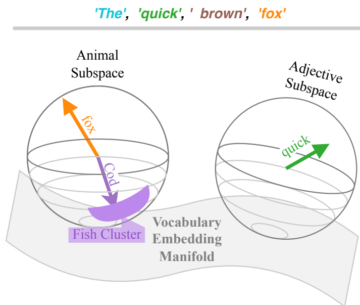
Figure 7.1: We attempt to visualise how high-dimensional vectors can exist in multiple structured sub-spaces simultaneously. In this example, the sentence ‘The quick brown fox’ has been tokenised into ‘The’, ‘quick’, ‘brown’, ‘fox’, and we attempt to show the local substructure that may emerge in the embeddings of these tokens based on their semantic contents. In practice, a single token is likely to span many such subspaces, with varying magnitudes capturing the degree of importance and saliency of a given concept; whilst here these concepts are direct reflections of the original tokens, most interesting structure in a models’ representations will exist in computational subspaces learned by the model to perform tasks.
