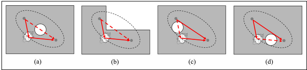
Figure 3. Disruption of wave propagation by openings: direct path between (a) actuator or (b) sensor; (c) path between the actuator and pixel; (d) path between the pixel and the sensor.
