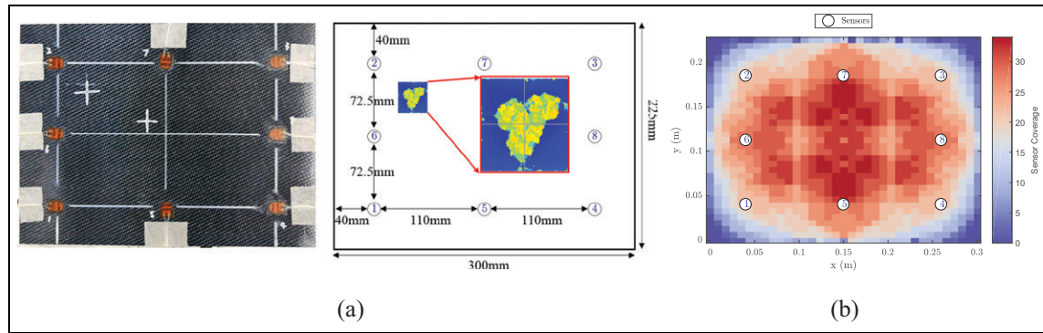
Figure 13. Quasi-isotropic woven CFRP panel. (a) Sensor placement. (b) Sensor coverage.
