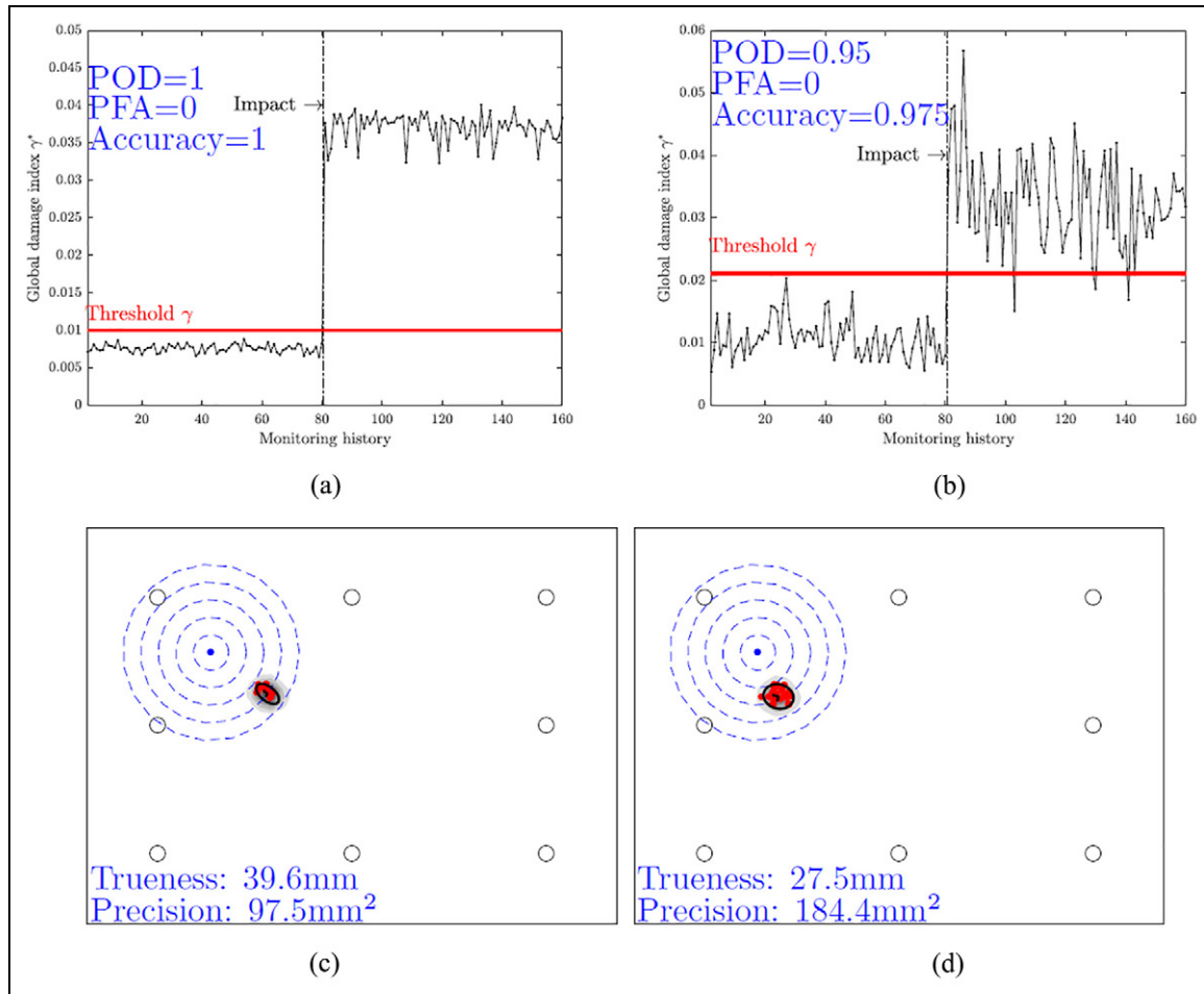
Figure 14. Damage identification results on the quasi-isotropic woven CFRP panel. Monitoring history of GDI \gamma^* derived from guided wave response at (a) 50 kHz and (b) 250 kHz. Damage localisation results and performance quantification at (c) 50 kHz and (d) 250 kHz.
