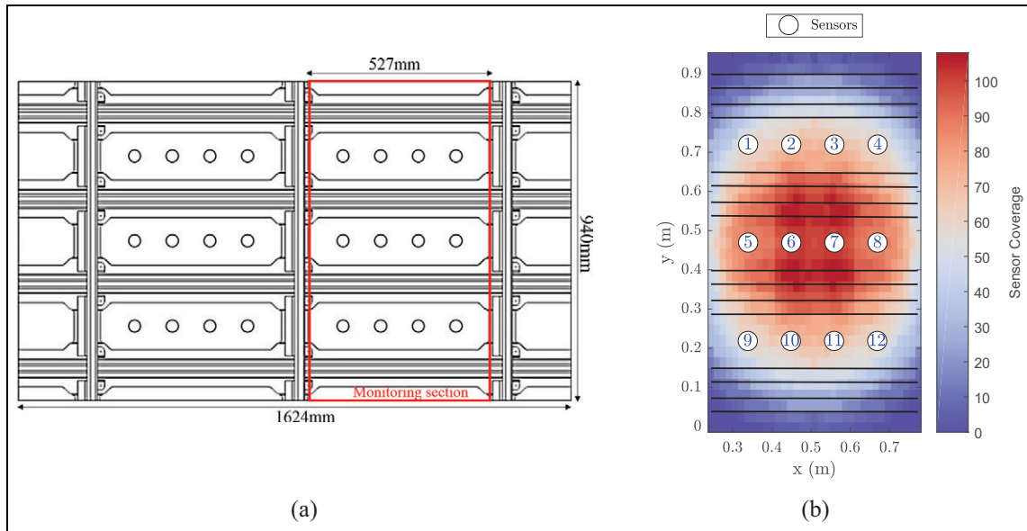
Figure 21. Flat stiffened panel with multiple stiffeners instrumented with DuraAct sensors. (a) Sensor placement. (b) Sensor network coverage of the highlighted monitoring section.
