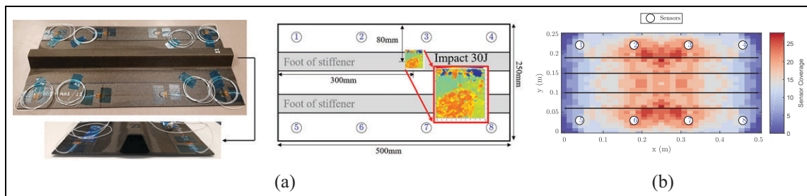
Figure 19. Anisotropic unidirectional CFRP panel with an omega stiffener: (a) Sensor placement. (b) Sensor coverage.
