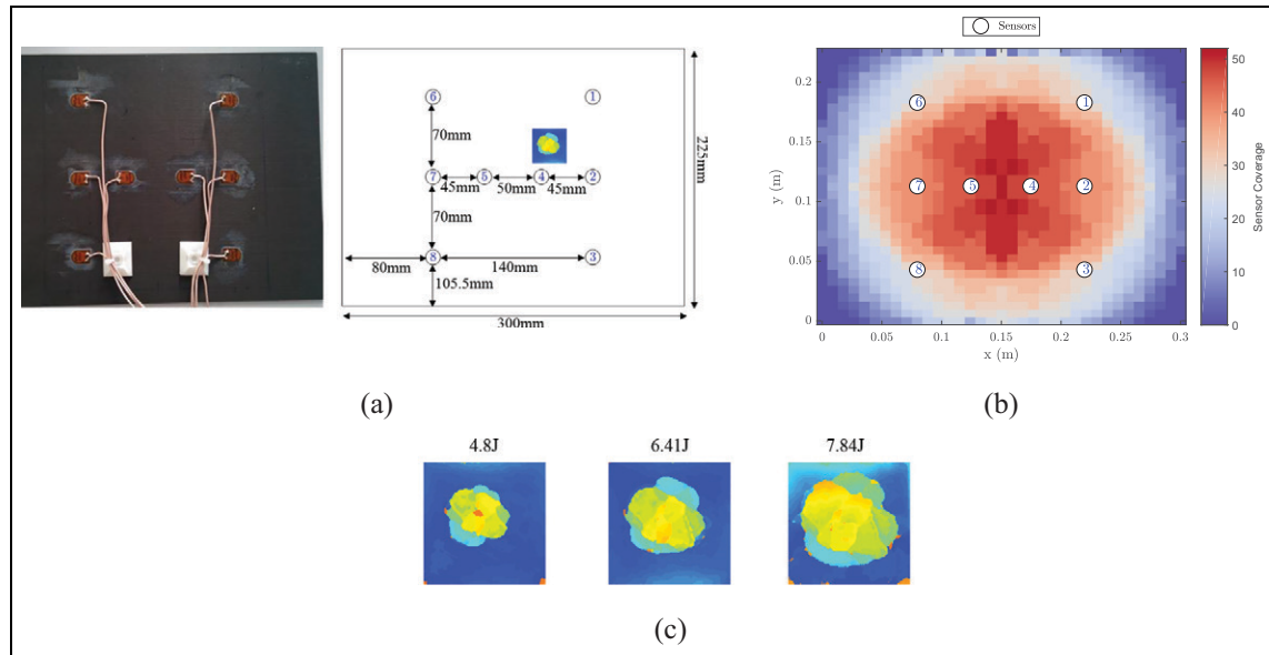
Figure 11. Quasi-isotropic unidirectional CFRP panel. (a) Sensor placement. (b) Coverage. (c) C-scan image of BVID after each impact event. The image size is 35 \times 35 \text{ mm}^2 .
