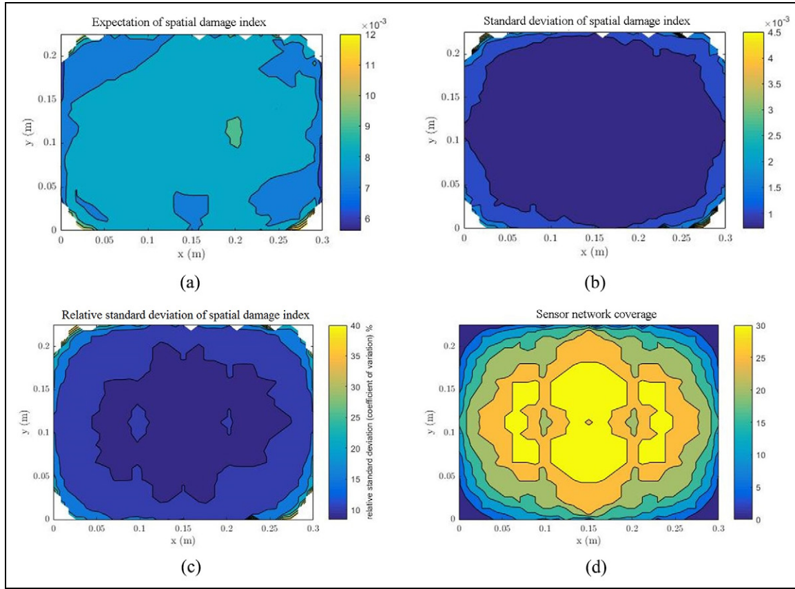
Figure 6. Spatial distribution of (a) expectation of the spatial damage index \mathbf{I} , \hat{\mu}_j , (b) standard deviation of the spatial damage index \mathbf{I} , \hat{\sigma}_j , (c) relative standard deviation \hat{\sigma}_j/\hat{\mu}_j and (d) sensor network coverage.
