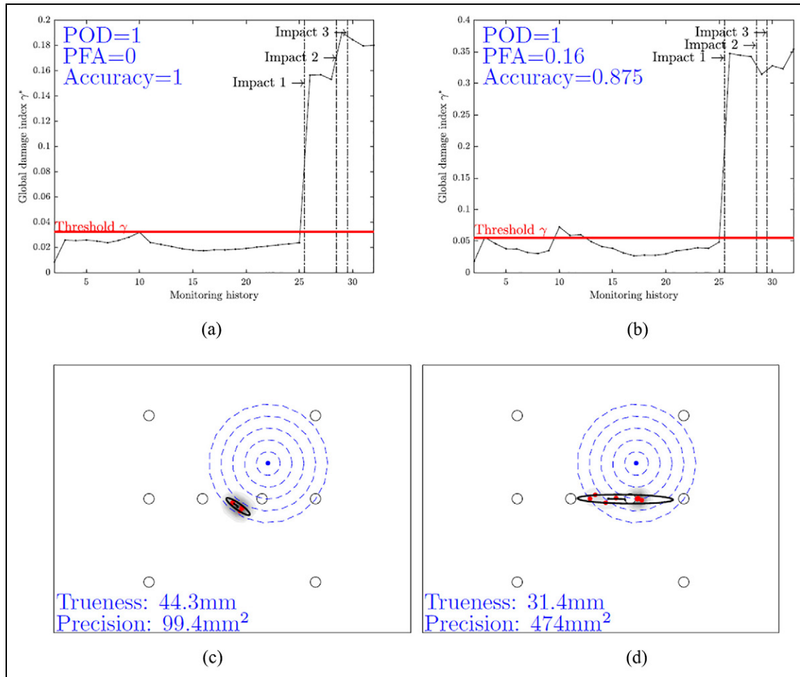
Figure 12. Damage identification results on the quasi-isotropic unidirectional CFRP panel. The monitoring history of the GDI \gamma^* derived from guided wave response at (a) 50 kHz and (b) 300 kHz. Damage localisation results and performance quantification at (c) 50 kHz and (d) 300 kHz.
