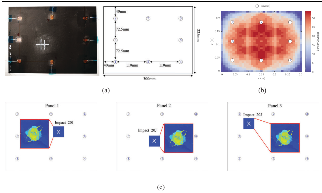
Figure 15. Anisotropic unidirectional CFRP panel. (a) Sensor placement. (b) Sensor coverage. (c) C-scan images of BVID after each impact event on three panels. The zoomed in area is 35 \times 35 \text{ mm}^2 .
