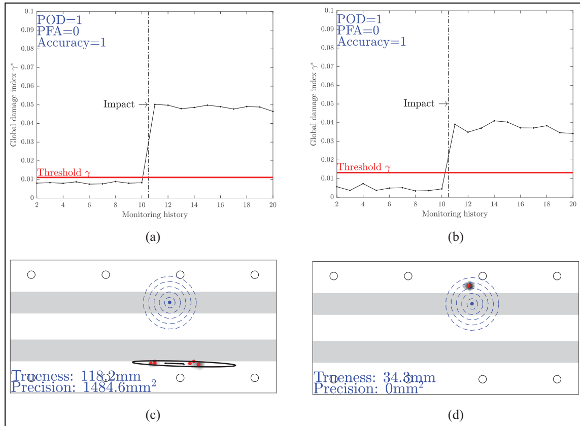
Figure 20. Damage identification results on anisotropic unidirectional CFRP panel with omega stiffener. Monitoring history of GDI \gamma^* at (a) 50 kHz and (b) 250 kHz. Damage localisation results and performance quantification at (c) 50 kHz and (d) 250 kHz.
