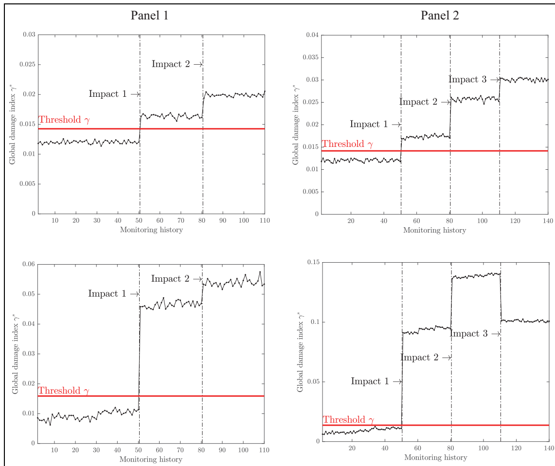
Figure 24. Monitoring history of GDI \gamma^* on stiffened panels at 50 and 250 kHz. For all cases, POD = 1, PFA = 0, accuracy = 1.
