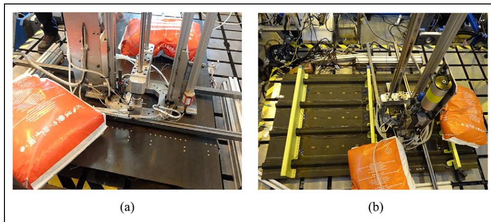
Figure 22. Impact setup. (a) Impact on the skin under the stiffener, simulating impact by runway debris. (b) Impact on the skin, simulating tool drop impact.
