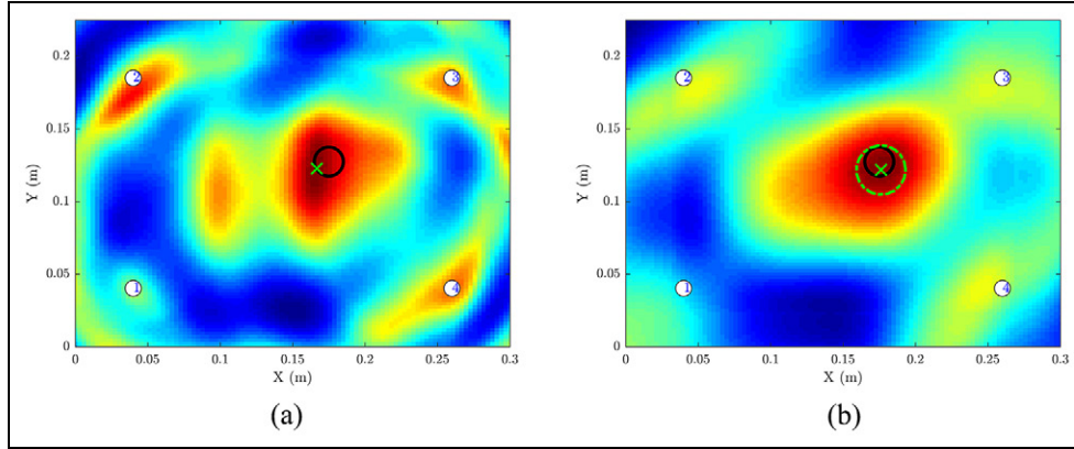
Figure 10. Application of a mean filter on the spatial likelihood index L(x) . L(x) is derived from DAS (a) before mean filtering and (b) after mean filtering. The black circle indicates the actual damage location. The green circle marks the estimated damage location.
