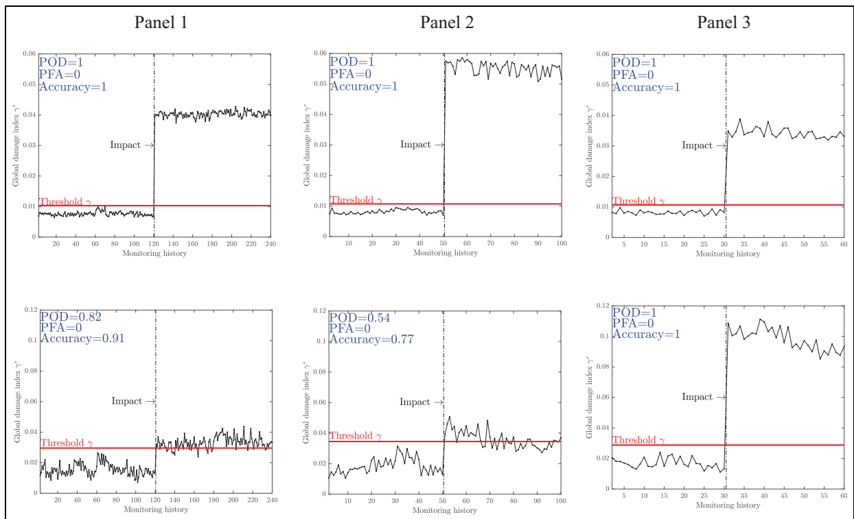
Figure 16. Monitoring history of GDI \gamma^* on three anisotropic unidirectional CFRP panels at 50 and 250 kHz.
