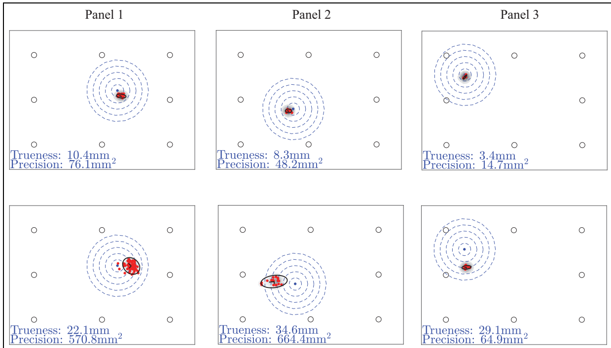
Figure 17. Damage localisation results and performance quantification on three anisotropic unidirectional CFRP panels at 50 and 250 kHz.
