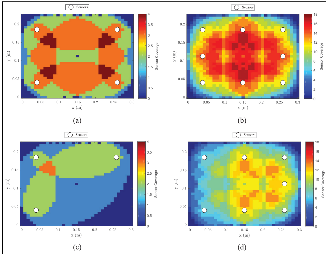
Figure 9. Sensor coverage of (a) four sensors, (b) eight sensors, (c) three sensors and (d) seven sensors.
