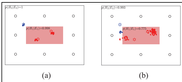
Figure 18. Probability of correctly indicating damage in a critical zone with guided waves at (a) 50 kHz and (b) 250 kHz.
