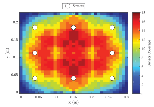
Figure 4. Sensor coverage of an eight-sensor network.
