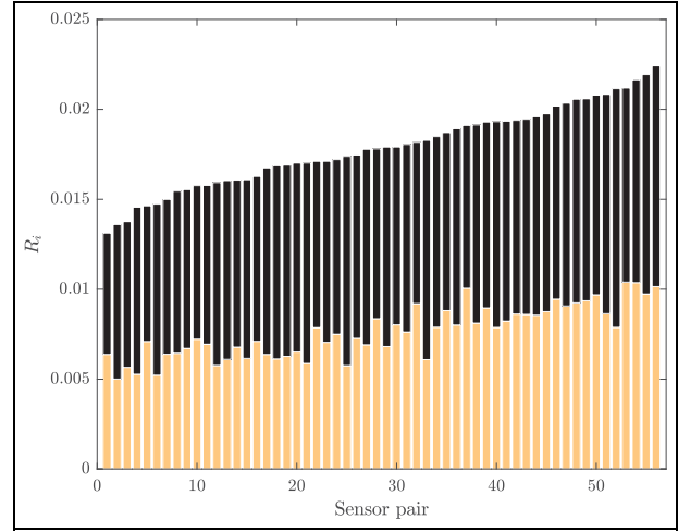
Figure 5. The upper bound of 56 damage-sensitive features in pristine state. The yellow bar represents the value of \hat{\mu}_i and the black bar indicates the value of Z_{99.9\%}\hat{\sigma}_j . The sensor pairs are sorted by their upper confidence bound value.
