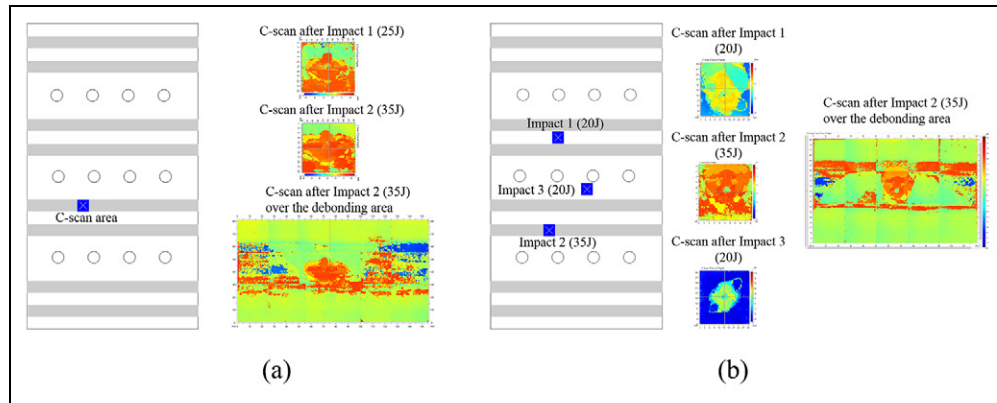
Figure 23. Impact location and C-scan after impact on (a) Panel 1 and (b) Panel 2.
