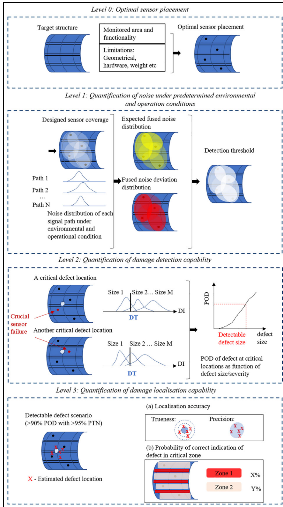
Figure 1. Hierarchical approach.
