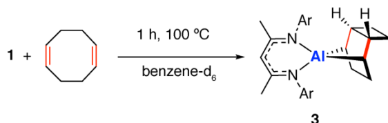
Scheme 2. Reaction of 1 with 1,5-cyclooctadiene to form 3 .
