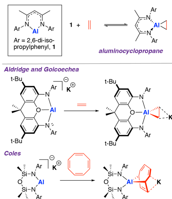
Figure 1. Reaction of selected aluminium(I) compounds with unsaturated hydrocarbons.
