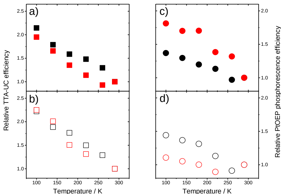
Figure 5. The relative efficiency of the green-to-blue PF TTA-UC PL intensity, as a function of temperature for a) PFO:PtOEP 6 wt% films cast from chloroform (black-filled squares) and toluene (red-filled squares) and b) PF26:PtOEP 6 wt% films cast from chloroform (black-open squares) and toluene (red-open squares). The relative efficiency of the PtOEP phosphorescence intensity, as a function of temperature for c) PFO:PtOEP 6 wt% films cast from chloroform (black-filled circles) and toluene (red-filled circles) and d) PF26:PtOEP 6 wt% films cast from chloroform (black-open circles) and toluene (red-open circles). In all cases the films were photoexcited at 532 nm, in resonance with the Q- absorption band of the PtOEP annihilator/sensitizer.
