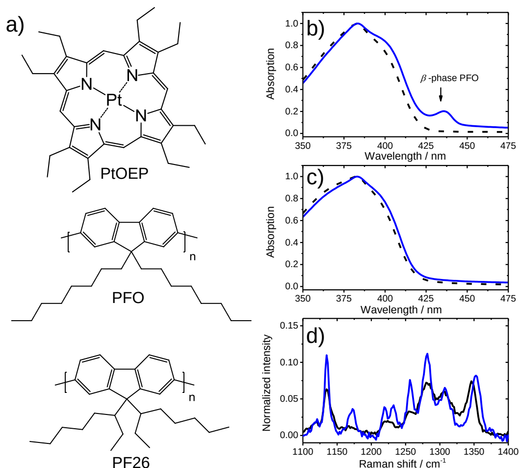
Figure 2. a) The chemical structures of the annihilator/sensitizer (PtOEP) and activator (PFO and PF26) materials used in this study, b) UV-Vis absorption spectra of PFO:PtOEP 6 wt% films spun from chloroform (black dash line) and toluene (blue solid line), c) UV-Vis absorption spectra of PF26:PtOEP 6 wt% films spun from chloroform (black dash line) and toluene (blue solid line), d) Normalized Raman spectra of PFO:PtOEP 6 wt% films spun from chloroform (black line) and toluene (blue line).
