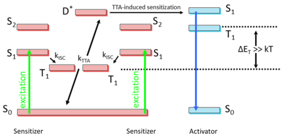
Figure 1. Triplet-triplet-annihilation-induced photon energy up-conversion in unconventional composites where no exothermic triplet energy transfer from sensitizer to activator is energetically probable. Triplet-triplet annihilation between triplet-excited sensitizers is followed by energy transfer from a doubly photoexcited sensitizer state ( D^* ) to a nearby activator that exhibits TTA-UC luminescence. In this scheme the low-energy photon absorber holds a dual annihilator/sensitizer role that drives the sensitization of a high-photon energy emitting activator.
