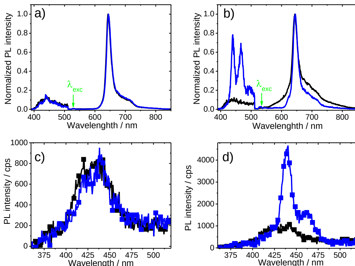
Figure 3. Normalized time-gated PL spectra of PF26:PtOEP 6 wt% (black lines) and PFO:PtOEP 6 wt% (blue lines) films, cast from a) chloroform and b) toluene. In both a) and b), the PL spectra are collected at room temperature, with a gate-width of 10 ns, 10 ns after photoexcitation. For clarity the PL intensity of the spectral region between 358 – 511 nm is multiplied by a factor of 15. Time-integrated PL spectra of PF26:PtOEP 6 wt% (black lines-squares) and PFO:PtOEP 6 wt% (blue lines-squares) films, cast from c) chloroform and d) toluene. In both c) and d) the data are collected at room temperature and corrected for the absorbance (1-T) of the films at the photoexcitation at 532 nm, in resonance with the Q-absorption band of the PtOEP annihilator/sensitizer.
