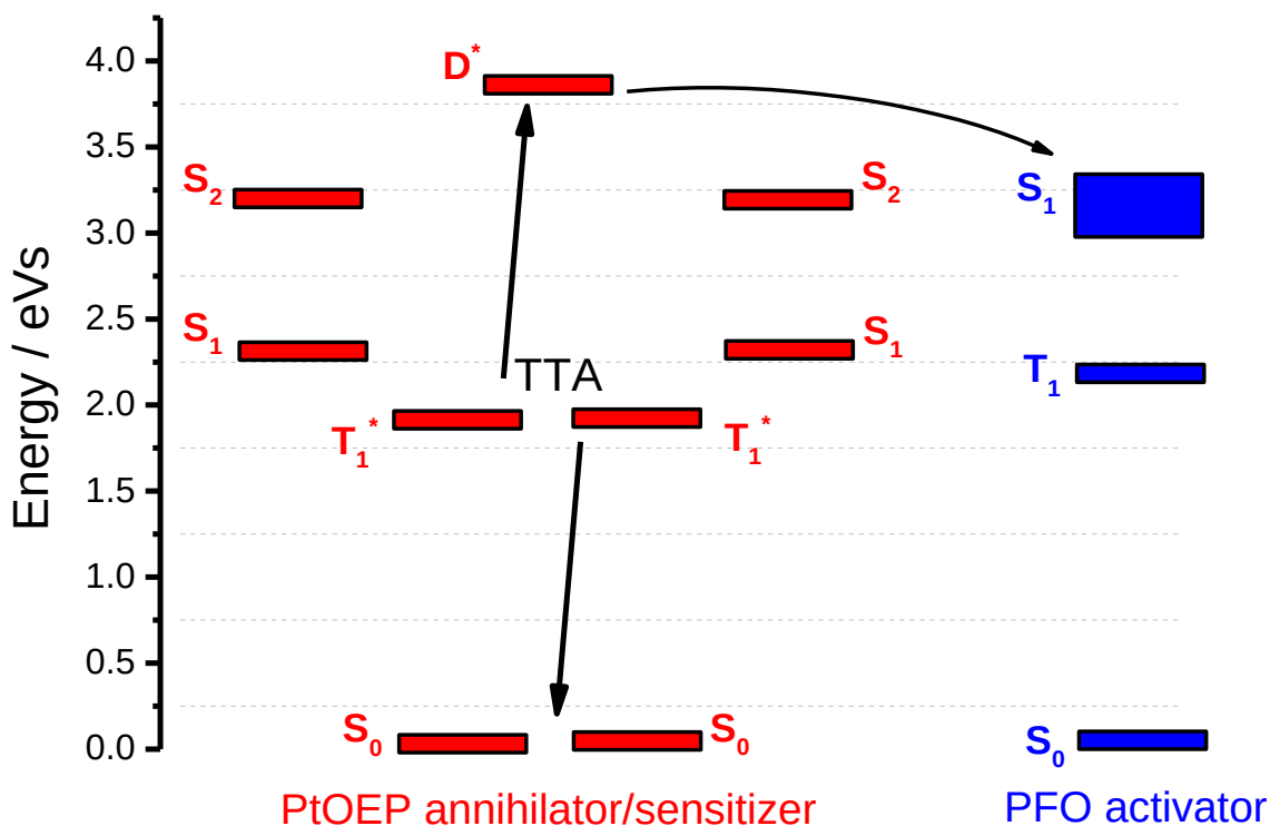
Figure 7. The energy diagram of the PFO:PtOEP composite system depicting the energetics of the levels that are involved in the generation of green-to-blue TTA-UC luminescence.
